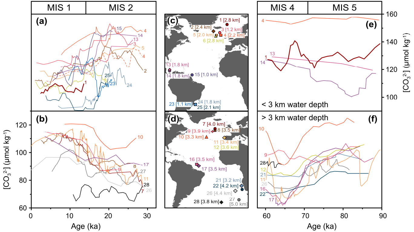
Fig. 9: Compilation of Atlantic bottom water [\text{CO}_3^{2-}] reconstructions (five point-running means) for the time intervals a, b) MIS 2 to MIS 1 (i.e., the last deglaciation) and e, f) MIS 5a to MIS 4 (i.e., the last glacial inception) (numbers at core locations and timeseries refer to core locations given in Table 1). c, d) Core locations of epibenthic foraminiferal B/Ca-based [\text{CO}_3^{2-}] reconstructions from the Atlantic Ocean and the Nordic Seas (numbers at core locations refer to metadata given in Table 1 and numbers in brackets highlight the water depth at the core sites), with colours equivalent to those shown at the onset (a, b) and end (e, f) of the reconstructed bottom water [\text{CO}_3^{2-}] records. The bottom water [\text{CO}_3^{2-}] record of ODP Site 980 (with label number 4) in a) is shown as solid line following Chalk et al. (2019) and as dashed orange line following the record of Crocker et al. (2016). C. wuellerstorfi B/Ca from Crocker et al. (2016) was converted into [\text{CO}_3^{2-}] using the calibration applied in section 3.3 (Yu and Elderfield 2007) and using the core-top [\text{CO}_3^{2-}] value (119 \mu\text{mol/kg} ) reported by Chalk et al. (2019). Upper and lower panels show core sites shallower and deeper than 3 km water depth, respectively. Boxes at the top indicate marine isotope stages (MIS) following Lisiecki and Raymo (2005) and marine isotope substages (MIS 5a) according to Railsback et al. (2015).
