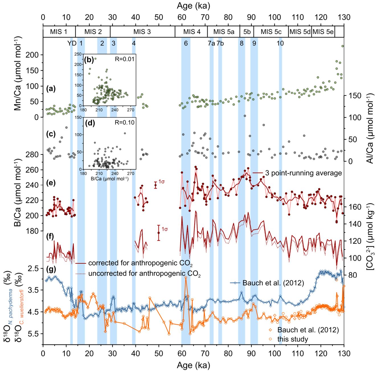
300 Fig. 3: Foraminiferal trace element and stable oxygen isotope variations during the last glacial cycle in core PS1243. (a) C. wuellerstorfi Mn/Ca and (b) cross-plotted against C. wuellerstorfi B/Ca ratios, (c) C. wuellerstorfi Al/Ca and (d) cross-plotted against C. wuellerstorfi B/Ca ratios. (e) C. wuellerstorfi B/Ca ratios (error bar indicates the mean 1 \sigma -uncertainty of B/Ca down -
