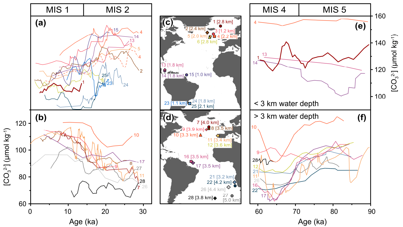
Fig. 98: Compilation of Atlantic bottom water [\text{CO}_3^{2-}] reconstructions (five point-running means) for the time intervals a, b MIS 2 to MIS 1 (i.e., the last deglaciation) and e, f MIS 5a to MIS 4 (i.e., the last glacial inception) (numbers at core locations and timeseries refer to core locations given in Table 1). Dashed line displays the average reconstructed bottom water [\text{CO}_3^{2-}] value ( -111 \pm 26 \mu\text{mol/mol} ) from all compiled sediment cores with core-top ages younger than 3000 years before present. b, c, d Core locations of epibenthic foraminiferal B/Ca-based [\text{CO}_3^{2-}] reconstructions from the Atlantic Ocean and the Nordic Seas (numbers at core locations refer to metadata given in Table 1 and numbers in brackets highlight the water depth at the core sites), with symbol type and colour equivalent to those shown at the onset ( a, b ) and end ( e, f ) of the reconstructed bottom water [\text{CO}_3^{2-}] records. The bottom water [\text{CO}_3^{2-}] record of ODP Site 980 (with label number 4 in a ) is shown as solid line following yellow, Chalk et al. (2019) and as dashed orange line following the record of Crocker et al. (2016). C. wuellerstorfi B/Ca from Crocker et al. (2016) was converted into [\text{CO}_3^{2-}] using the calibration applied in section 3.3 (Yu and Elderfield 2007) and using the core-top [\text{CO}_3^{2-}] value ( 119 \mu\text{mol/kg} ) reported by Chalk et al. (2019). Upper and lower panels show core sites shallower and deeper than 3 km water depth, respectively, was recalibrated according to younger epibenthic core-top B/Ca values presented in Crocker et al. (2016) (dashed line). Boxes at the top indicate marine isotope stages (MIS) following Lisiecki and Raymo (2005) and marine isotope substages (MIS 5a) according to Railsback et al. (2015).
