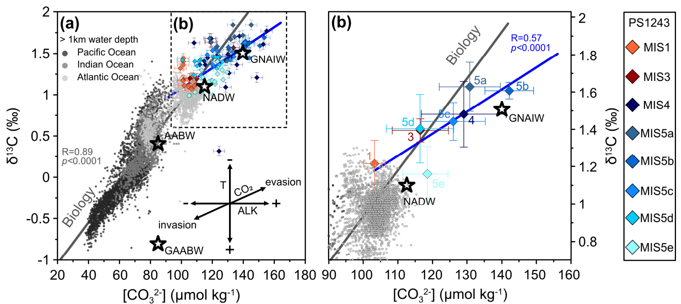
370 Fig. 5: Correlation of C. wuellerstorfi \delta^{13}\text{C} and B/Ca-based [\text{CO}_3^{2-}] estimates in sediment core PS1243. (a) Modern seawater \delta^{13}\text{C} and [\text{CO}_3^{2-}] (Lauvset et al., 2022). Black stars indicate endmember values of North Atlantic Deep Water (NADW), Antarctic Bottom Water (AABW), Glacial North Atlantic Intermediate Water (GNAIW) and Glacial Antarctic Bottom Water (GAABW) after Yu et al. (2008; 2020). Diamonds indicate paired C. wuellerstorfi \delta^{13}\text{C} and B/Ca-based [\text{CO}_3^{2-}] estimates in core PS1243 (color-coded according to time interval) with blue line showing a linear regression of the downcore data (excluding C. wuellerstorfi \delta^{13}\text{C} values lower than 0.5 ‰). (b) Averaged C. wuellerstorfi \delta^{13}\text{C} and B/Ca-based [\text{CO}_3^{2-}] estimates (stippled box in a) for marine isotope stages (MIS) and substages following Lisiecki and Raymo (2005) and Railsback et al. (2015), respectively (color-coded according to the time interval), with blue line indicating the linear regression. Grey lines in a) and b) show the Redfield slope, while vectors in the right-bottom corner of panel (a) indicate an increase in seawater \delta^{13}\text{C} with decreasing temperature (T), an increase in [\text{CO}_3^{2-}] with rising alkalinity (ALK) and increases in both [\text{CO}_3^{2-}] and \delta^{13}\text{C} with \text{CO}_2 evasion/invasion to/from the atmosphere (Yu et al. 2008).
