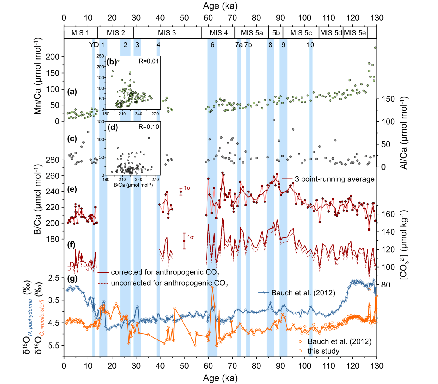
Fig. 3: Foraminiferal trace element and stable oxygen isotope variations during the last glacial cycle in core PS1243. (a) C. wuellerstorfi Mn/Ca and (b) cross-plotted against C. wuellerstorfi B/Ca ratios, (c) C. wuellerstorfi Al/Ca and (d) cross-plotted against C. wuellerstorfi B/Ca ratios. (e) C. wuellerstorfi B/Ca ratios (error bar indicates the mean 1\sigma -uncertainty of B/Ca down ).
