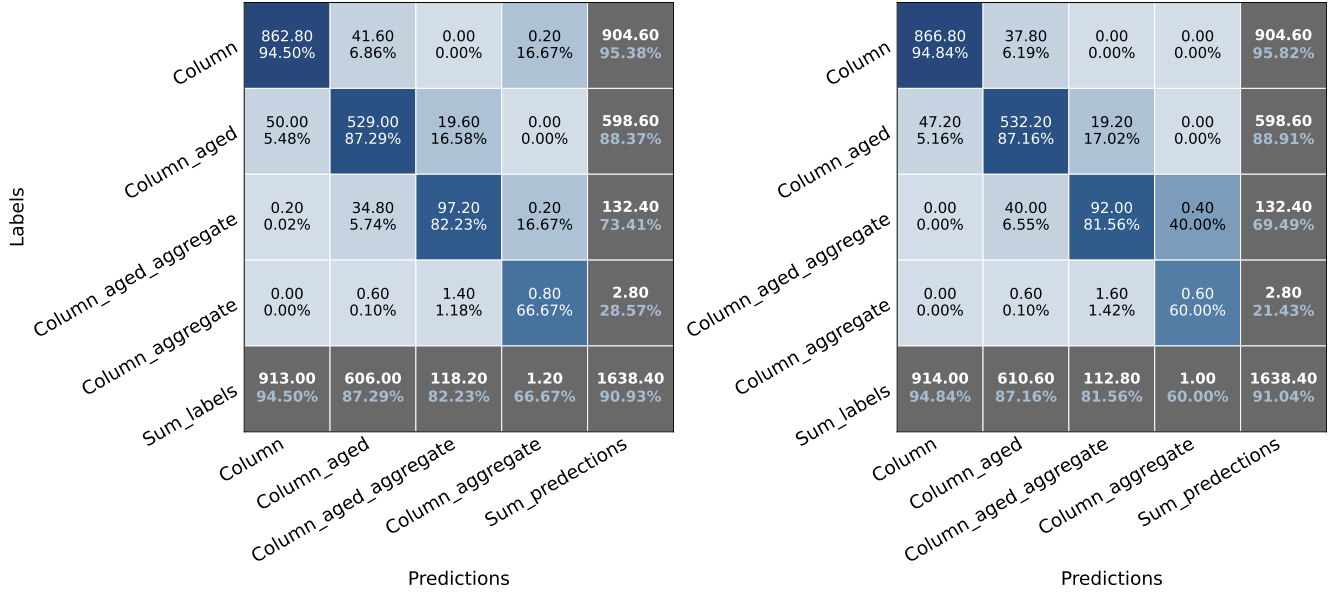
Figure 11. The same as Fig. 6 and Fig. 7 but for NASCENT-4CAT. The confusion matrix is not divided into basic habits as complex shapes because there are only 4 categories in the dataset.
