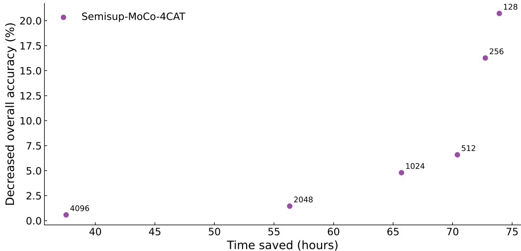
Figure 10. The same as Fig. 5 but for Semisup-MoCo-4CAT.
