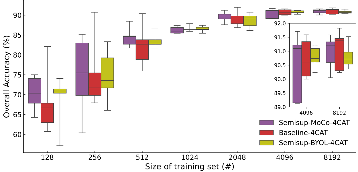
Figure 9. The same as Fig. 4 except the results are evaluated on NASCENT19-4CAT. The result from IceDetectNet is not shown here because it was not trained on NASCENT19-4CAT. The maximum size of training set here is set to 8192 instead of 16384 because the size of NASCENT19-4CAT is smaller than 16384.
