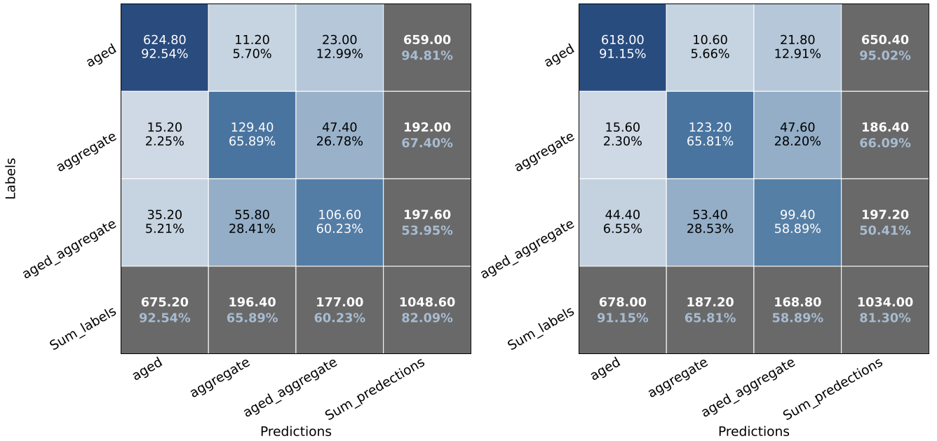
Figure 7. The same as Fig. 6 but the confusion matrix is calculated on the complex shapes of ice crystals. The rest 13 complex shapes are merged down to 3 types here: "aged", "aggregate", "aged_aggregate", which represents the microphysical processes happened to the ice crystals.
