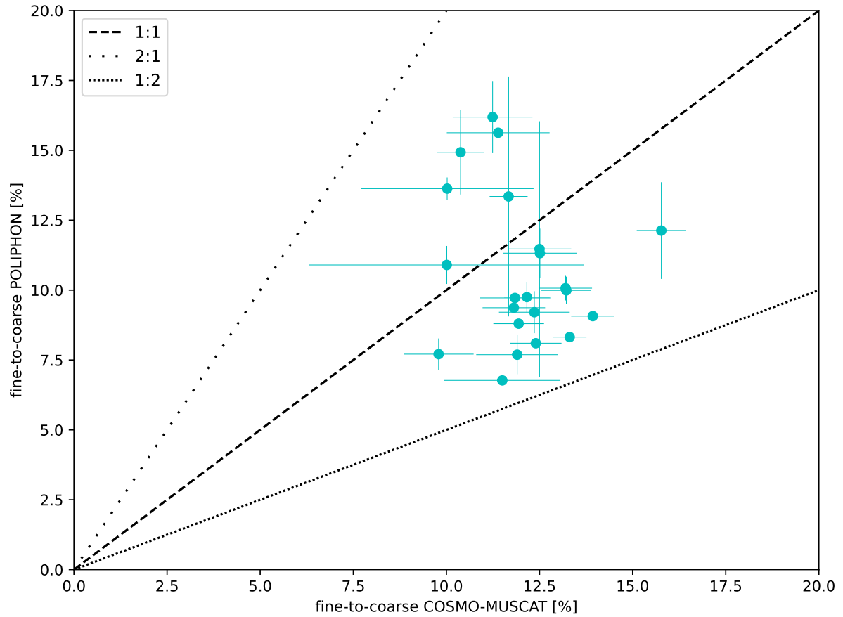
Figure 6. Fine-to-coarse dust mass concentrations comparison between COSMO-MUSCAT and POLIPHON. The dashed line represents the 1:1 line and the dotted lines represent the 2:1 and 1:2 lines as indicated in the legend. The error bars represent the standard deviation of the ratio per dust layer.
