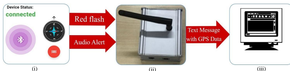
Figure 12. SOS/Emergency Response model deployed in STMET. (i) Display with SOS (ii) Receiver module (iii) PC monitor
