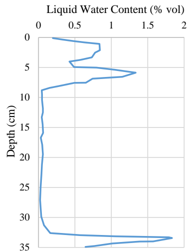
Figure 10. Water content in snowpack using STMET
