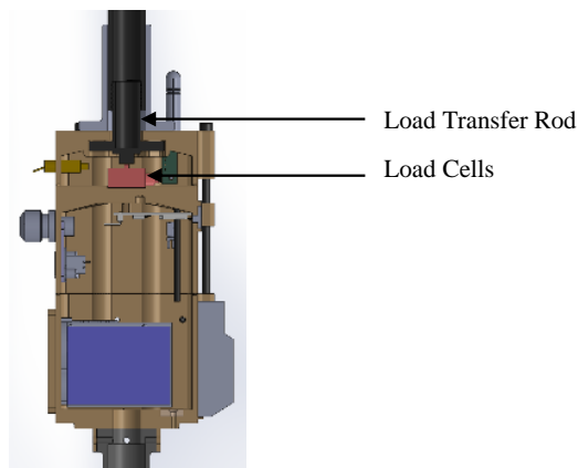
Figure 3. Load cell assembly
