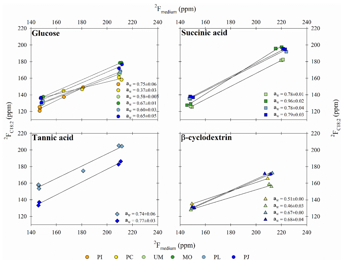
Figure 4. The water hydrogen assimilation factor ( a_w values) estimated as the slope of the fractional ^2\text{H} abundance ( ^2\text{F} ) in lipids (y-axis) versus medium water (x-axis). Data are shown for fungal biomarker \text{C}_{18:2} produced during growth on the different substrates (glucose, succinic acid, tannic acid and \beta -cyclodextrin) and harvested from the different fungal isolates [ Paxillus involutus (PI), Phanerodonta chrysosporium (PC), Mortierella sp. (MO), Umbelopsis sp. (UM), Penicillium janczewskii (PJ), and Paecilomyces lilacinus (PL)]. R^2 values for all slopes were > 0.97 .
