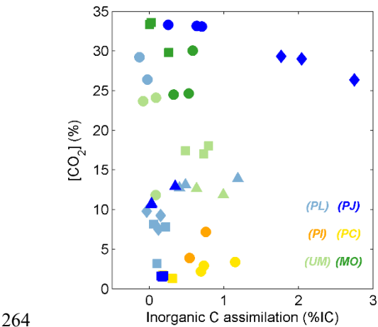
264 265 266 Figure 3. %IC values for fungal species respiring glucose (circles), succinate (squares), tannic acid (diamonds), or \beta - 267 cyclodextrin (triangles). Colors represent individual fungal isolates as described in Fig. 1.
