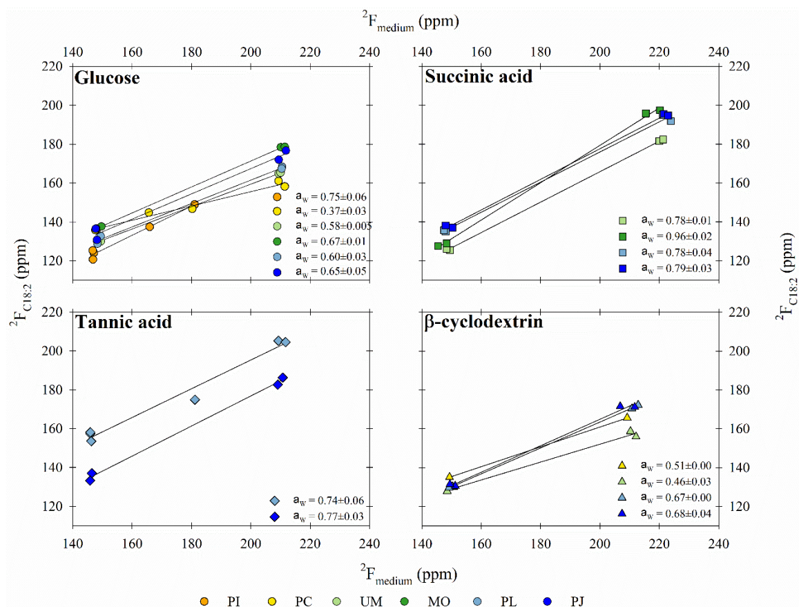
Figure 4. The water hydrogen assimilation factor ( a_w values) estimated as the slope of the fractional ^2H abundance ( ^2F ) in lipids (y-axis) versus medium water (x-axis). Data are shown for fungal biomarker C_{18:2} produced during growth on the different substrates (glucose, succinic acid, tannic acid and \beta -cyclodextrin) and harvested from the different fungal isolates [ Paxillus involutus (PI), Phanerodonta chrysosporium (PC), Mortierella sp. (MO), Umbelopsis sp. (UM), Penicillium janczewskii (PJ), and Paecilomyces lilacinus (PL)]. R^2 values for all slopes were > 0.97 .
