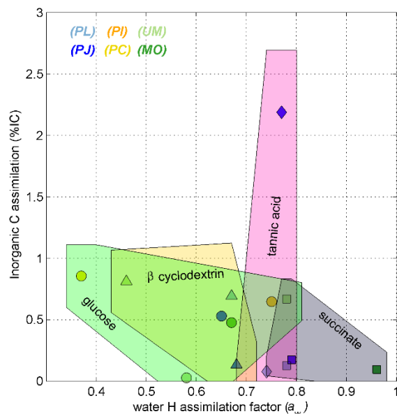
Figure 7. Scatterplot of %IC and a_w values plot for C_{18:2} harvested from incubations of Ascomycota (blue symbols), Basidiomycota (yellow and orange symbols), and Zygomycota (green symbols). The shaded polygons span the range of %IC and a_w values ( \pm propagated error) for fungal growth on glucose (circles, green shape), succinate (squares, grey shape), tannic acid (diamonds, pink shape), or \beta -cyclodextrin (triangles, yellow shape). Each data point represents one species-substrate pair determined for n > 4 growth experiments.
