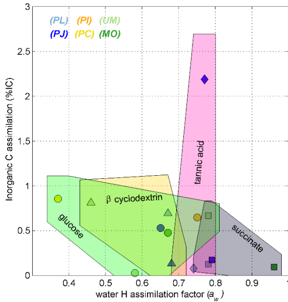
Figure 7. Scatterplot of %IC and a_w-a_w values plot for C 18:2 harvested from incubations of Ascomycota (blue symbols), Basidiomycota (yellow and orange symbols), and Zygomycota (green symbols). The shaded polygons span the range of %IC and a_w-a_w values ( \pm propagated error) for fungal growth on glucose (circles, green shape), succinate (squares, grey shape), tannic acid (diamonds, pink shape), or \beta -cyclodextrin (triangles, yellow shape). Each data point represents one species-substrate pair determined for n > 4 growth experiments.
