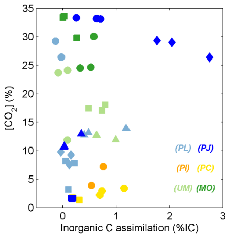
266 267 268 Figure 3. %IC values for fungal species respiring glucose (circles), succinate (squares), tannic acid (diamonds), or \beta - 269 cyclodextrin (triangles). Colors represent individual fungal isolates as described in Fig. 1.
