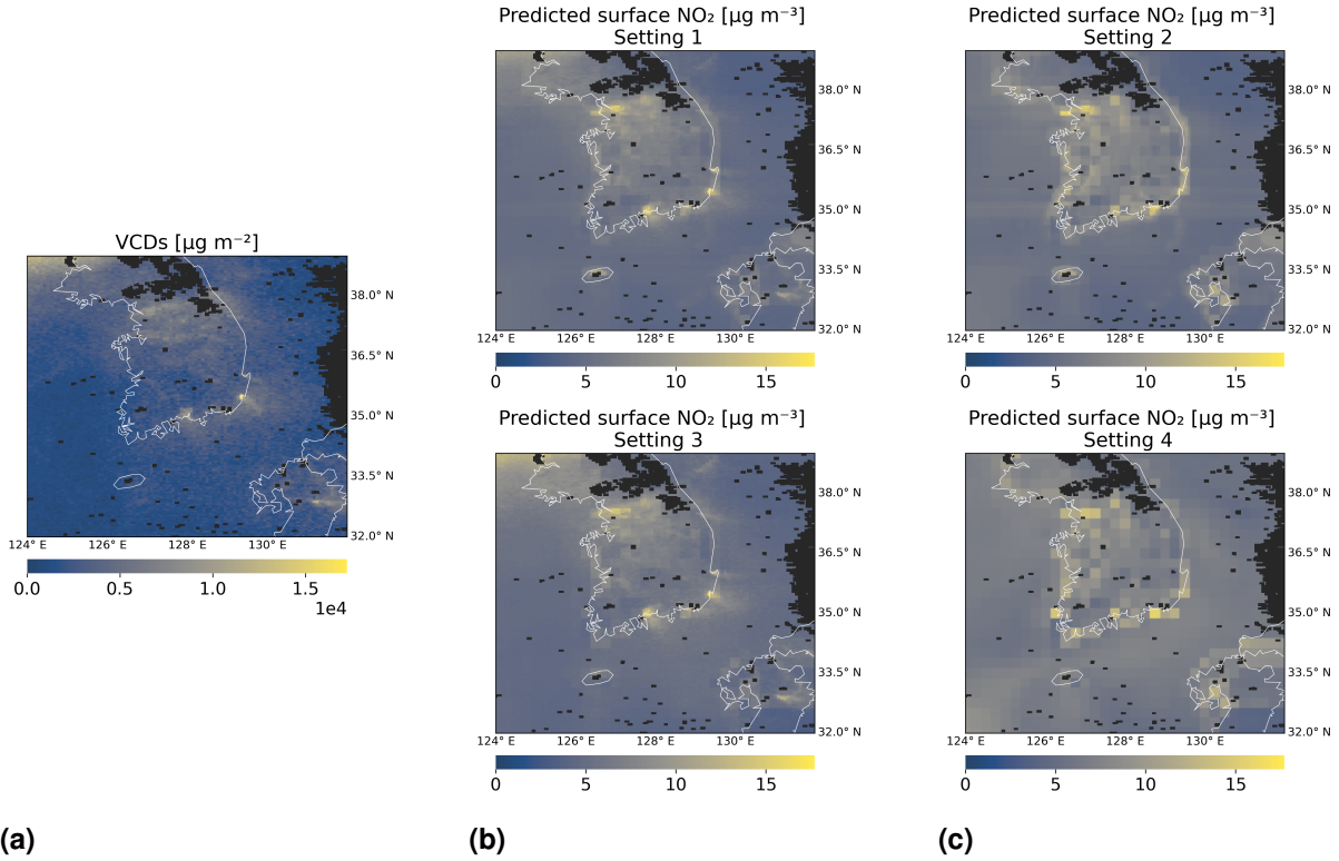
Figure 11. Same as Fig. 10, but on 27 February 2022. Column (a) shows the VCDs from 06:45 to 07:15 UTC. Columns (b) and (c) show predicted surface \text{NO}_2 from 06:00 to 07:00 UTC, for the four settings of Experiment 3.
