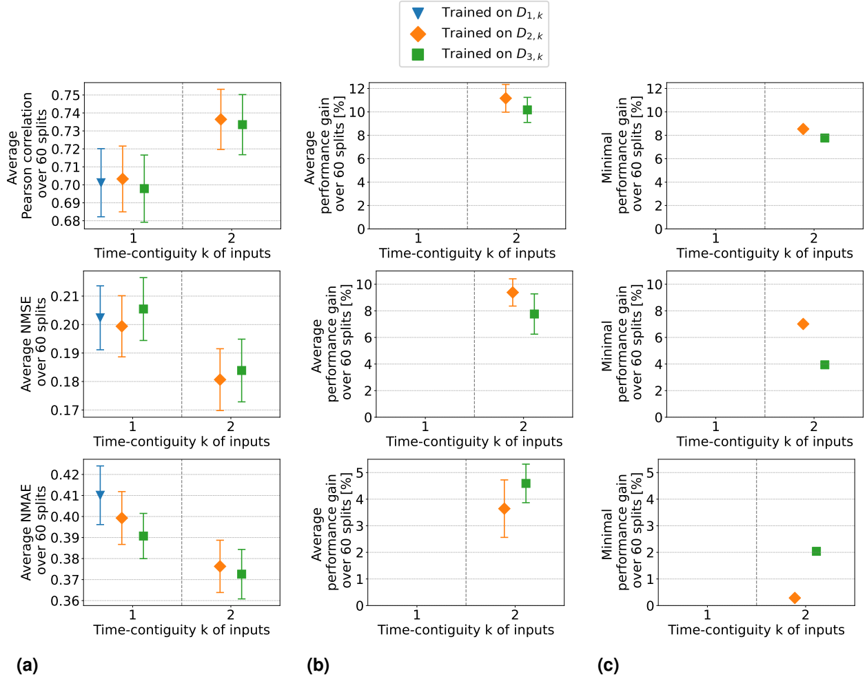
Figure C2. Linear regression models have been trained on D_{M,k} for M \leq 3 with different time-contiguities k and input features selected in Sect. 3.1. Performance on D_{2,k} has been evaluated by six times 10-fold spatial cross validation. Column (a) shows the average performance over all 60 station splits for three performance measures. Column (b) shows the average performance gain (Eq. (6)) relative to the best case of k = 1 . Errorbars illustrate the standard deviation. Column (c) shows the minimal performance gain. Across each row the same performance measure is considered.
