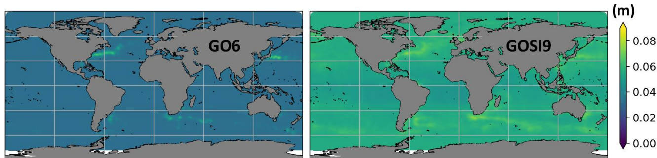
Figure 1. ORCA025 SLA observation errors (m) for the December to February season for GO6 (left) and GOSI9 (right).
