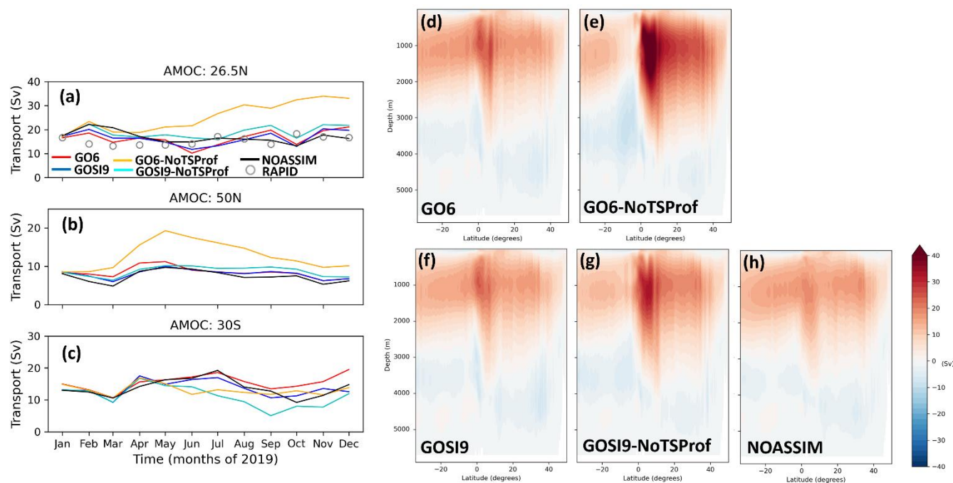
Figure 14. Monthly AMOC transports (Sv) in 2019 at (a) 26.5°N, (b) 50°N and (c) 30°S for FOAM GO6 (red), GO6-NoTSPProf (orange), GOSI9 (blue), GOSI9-NoTSPProf (cyan) and NOASSIM (black). Note that observed AMOC transports from the RAPID array (grey) are also included at 26.5°N. (d-h) AMOC stream function (Sv) for all the FOAM runs.
