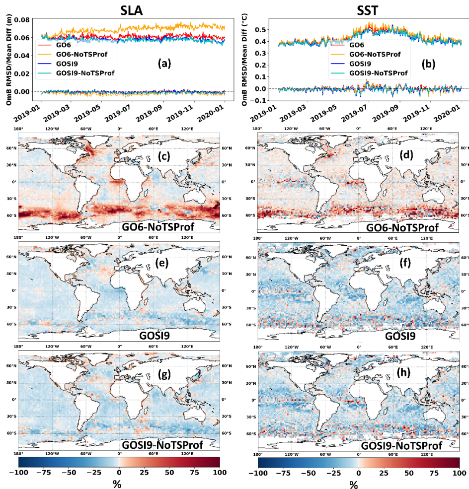
Figure 10. (a, b) 2019 ORCA025 OmB statistics for FOAM GO6 (red), GO6-NoTSPProf (orange), GOSI9 (blue) and GOSI9-NoTSPProf (cyan), calculated against SLA (m) and SST ( ^{\circ} C) observations, respectively. The solid lines correspond to RMSDs, and the dashed lines represent mean differences. 2019 RMSD percentage improvements (blue) and degradations (red) of (c, d) GO6-NoTSPProf, (e, f) GOSI9 and (g, h) GOSI9-NoTSPProf relative to GO6 for SLA and SST, respectively. Observations used for SLA are all the along-track altimeters available, whereas for SST observations used are in situ drifters.
