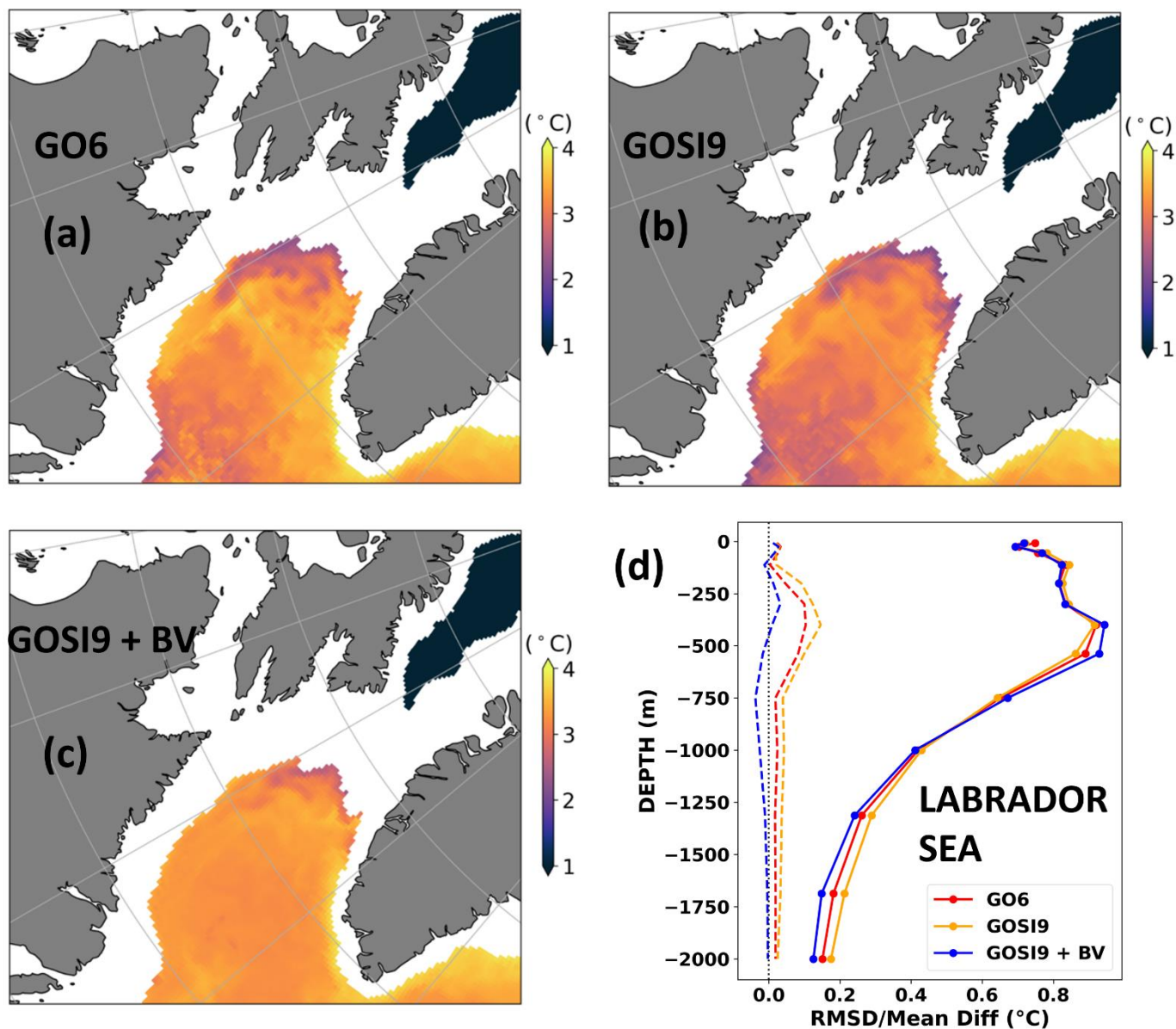
Figure 4. FOAM ORCA025 temperature fields ( ^{\circ}\text{C} ) at 1200 m in the Labrador Sea for (a) GO6, (b) GOSI9 and (c) GOSI9 additionally applying Brunt-Väisälä verifications on the T/S increments. These are snapshots of 31 March 2019 after all runs have been initialised on 1 January 2019 from the same initial condition. (d) FOAM ORCA025 OmB RMSD (solid) and mean difference (dashed) relative to T profiles observations between January and April 2019 for the Labrador Sea region.
