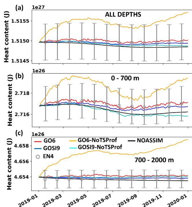
Figure 13. Daily heat content (J) time series for the global ocean calculated (a) at all depths, (b) 0-700 m and (c) 700-2000 m. Monthly heat content and its uncertainties from the EN4 objective analysis are also shown. The heat content uncertainties are derived from EN4 monthly temperature uncertainties.
