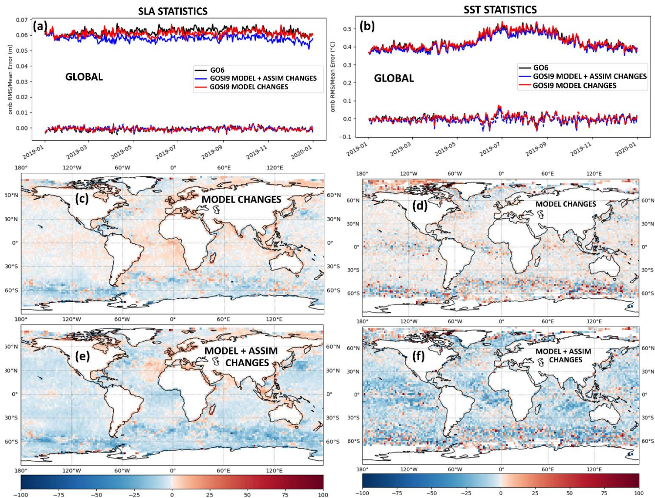
64 Figure S7. (a, b) 2019 FOAM ORCA025 OmB statistics for GO6 (black), GOSI9 only considering model updates (red) and GOSI9 65 considering both model and DA updates (blue), calculated against SLA (m) and SST ( ^{\circ} C) observations, respectively. The solid lines 66 correspond to RMSDs, and the dashed lines represent mean differences. 2019 RMSD percentage improvements (blue) and 67 degradations (red) of (c, d) ORCA025 GOSI9 with only model updates and (e, f) ORCA025 GOSI9 with model and DA updates 68 relative to GO6 for SLA and SST, respectively. Observations used for SLA are all the along-track altimeters available, whereas for 69 SST observations used are in situ drifters.
