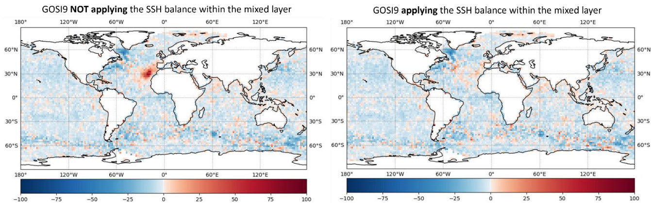
24 Figure S4. SLA observation-minus-background RMSD percentage improvement (blue) and degradation (red) of ORCA12 GOSI9 25 not applying (left) and applying (right) the SSH balance within the mixed layer relative to ORCA12 GO6. The statistics are calculated 26 from January to March 2019.
