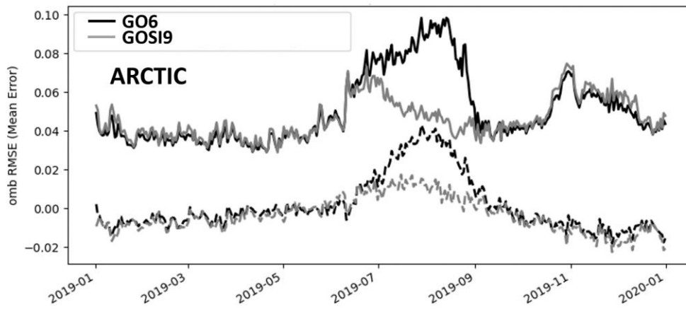
82 Figure S10. 2019 FOAM ORCA025 OmB statistics for GO6 (black) and GOSI9 (grey), calculated against SSMIS SIC observations 83 in the Arctic. The solid lines correspond to RMSDs, and the dashed lines represent mean differences.
