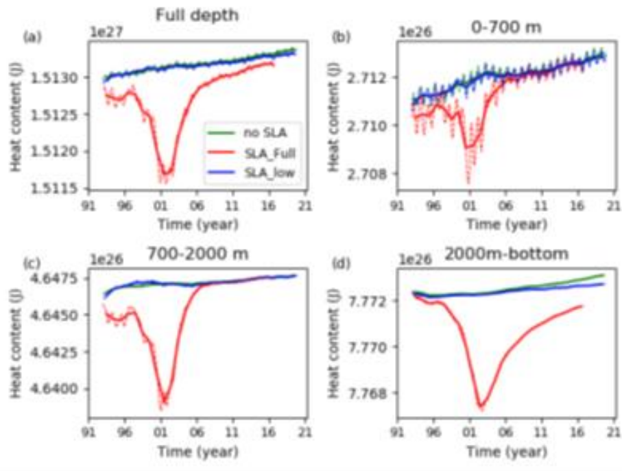
18 Figure S3. Annual-mean (solid lines) and monthly-mean (dotted lines) ocean heat content in the 1993-2020 FOAM reanalysis, 19 averaged globally over varying depths. The green line corresponds to a run without SLA assimilation, the red line corresponds to a 20 run assimilating SLA observations, and the blue line corresponds to a run giving low weights to SLA observations in the assimilation.
