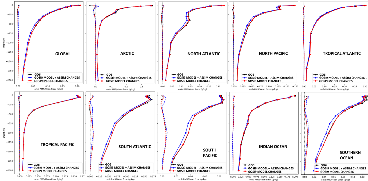
77 Figure S9. 2019 ORCA025 OmB salinity statistics for GO6 (black), GOSI9 only considering model updates (red) 78 considering both model and DA updates (blue), calculated against profile observations. The solid lines correspond to 79 RMSDs, and the dashed lines represent mean differences.
