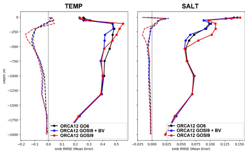
35 Figure S6. Observation-minus-background statistics for temperature (left) and salinity (right) in the Mediterranean Outflow region, 36 considering ORCA12 GO6 (black), ORCA12 GOSI9 (red) and ORCA12 GOSI9 applying the Brunt-Väisälä checks on T/S 37 increments (blue). The solid lines correspond to the RMSD and the dashed lines correspond to the mean differences with respect to 38 T/S profile observations in January-April 2019.
