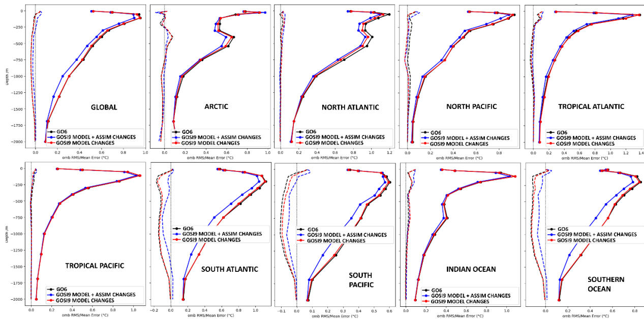
72 Figure S8. 2019 FOAM ORCA025 OmB temperature statistics ( ^{\circ}\text{C} ) for GO6 (black), GOSI9 only considering model updates (red) 73 and GOSI9 considering both model and DA updates (blue), calculated against profile observations. The solid lines correspond to 74 RMSDs, and the dashed lines represent mean differences.
