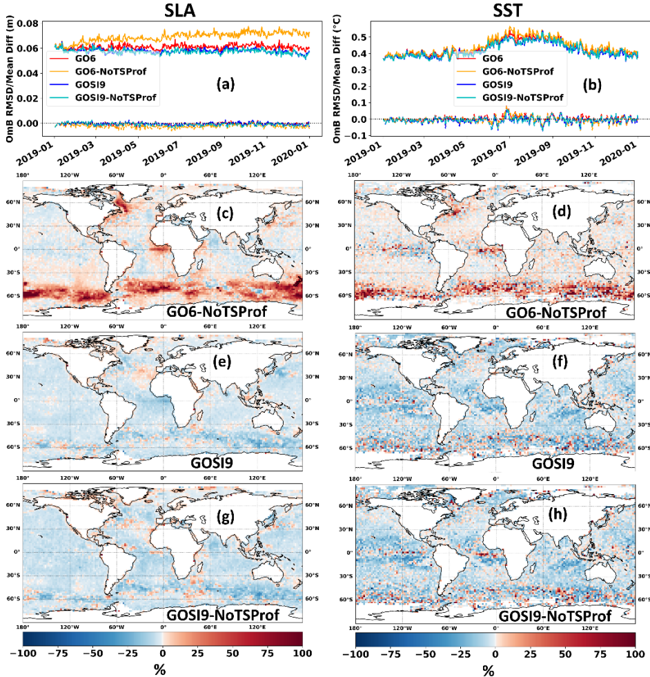
Figure 10. (a, b) 2019 ORCA025 OmB statistics for FOAM GO6 (red), GO6-NoTSProf (orange), GOSI9 (blue) and GOSI9-NoTSProf (cyan), calculated against SLA (m) and SST (°C) observations, respectively. The solid lines correspond to RMSDs, and the dashed lines represent mean differences. 2019 RMSD percentage improvements (blue) and degradations (red) of (c, d) GO6-NoTSProf, (e, f) GOSI9 and (g, h) GOSI9-NoTSProf relative to GO6 for SLA and SST, respectively. Observations used for SLA are all the along-track altimeters available, whereas for SST observations used are in situ drifters. The observations are binned onto a 0.25° grid in c-h.
