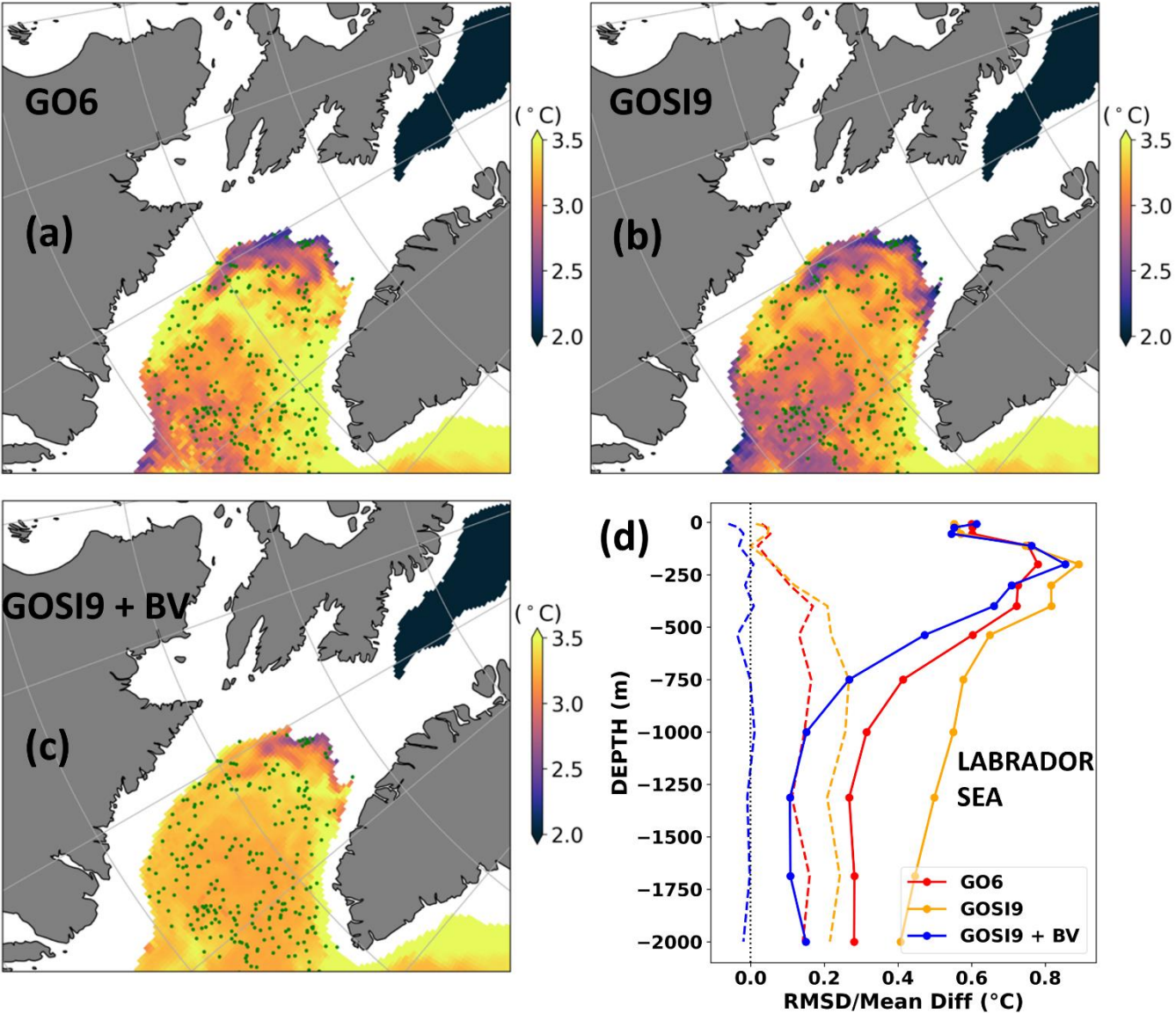
275 Figure 4. ORCA025 temperature fields (°C) at 1200 m in the Labrador Sea for FOAM (a) GO6, (b) GOSI9 and (c) GOSI9 additionally applying Brunt-Väisälä verifications on the T/S increments. These are snapshots of 31 March 2019 after all runs have been initialised on 1 January 2019 from the same initial condition. (d) OmB RMSD (solid) and mean difference (dashed) relative to 157 T profiles observations (green dots) between January and April 2019 for the Labrador Sea region.
