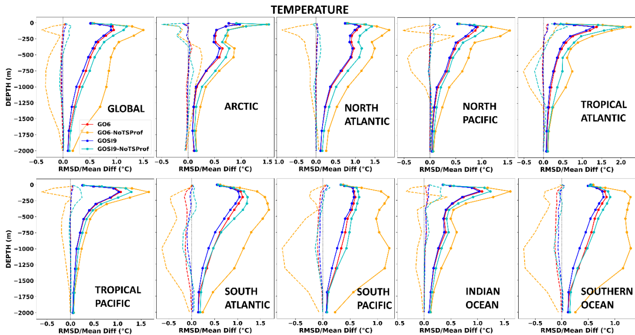
Figure 11. 2019 ORCA025 OmB temperature statistics (°C) for FOAM GO6 (red), GO6-NoTSPProf (orange), GOSI9 (blue) and GOSI9-NoTSPProf (cyan) calculated against profile observations in different ocean basins. The solid lines correspond to RMSDs, and the dashed lines represent mean differences.
