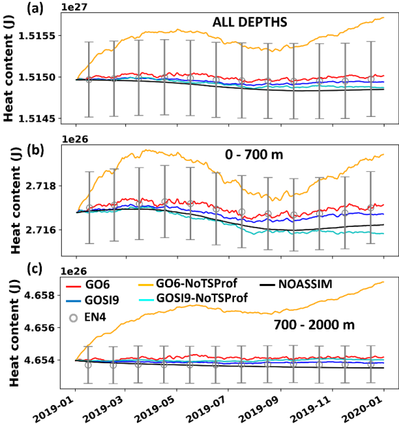
515 Figure 13. Daily heat content (J) time series for the global ocean calculated (a) at all depths, (b) 0-700 m and (c) 700-2000 m. Monthly heat content and its uncertainties from the EN4 objective analysis are also shown. The heat content uncertainties are derived from EN4 monthly temperature uncertainties.
