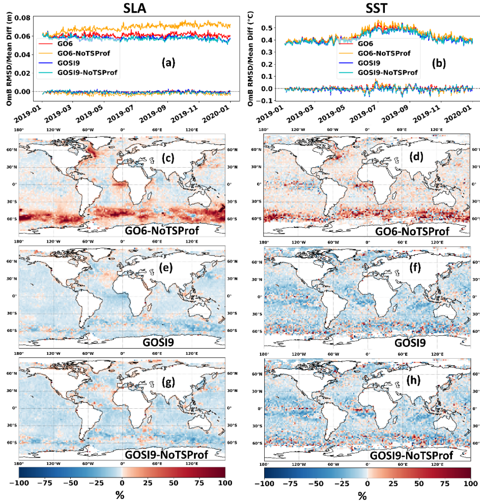
Figure 10. (a, b) 2019 ORCA025 OmB statistics for FOAM GO6 (red), GO6-NoTSPProf (orange), GOSI9 (blue) and GOSI9-NoTSPProf (cyan), calculated against SLA (m) and SST ( ^{\circ}\text{C} ) observations, respectively. The solid lines correspond to RMSDs, and the dashed lines represent mean differences. 2019 RMSD percentage improvements (blue) and degradations (red) of (c, d) GO6-NoTSPProf, (e, f) GOSI9 and (g, h) GOSI9-NoTSPProf relative to GO6 for SLA and SST, respectively. Observations used for SLA are all the along-track altimeters available, whereas for SST observations used are in situ drifters.
