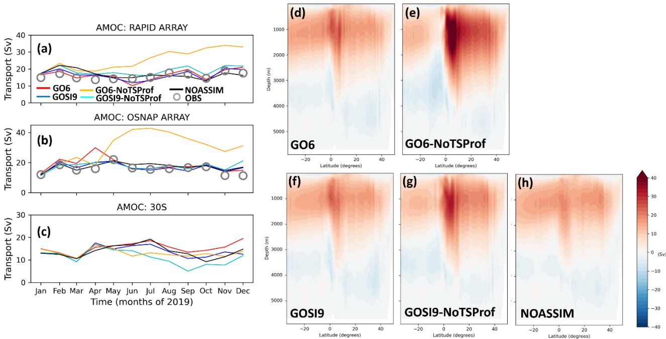
580 Figure 14. Monthly AMOC transports (Sv) in 2019 at along the (a) 26.5°N RAPID array, (b) 50°N OSNAP array and (c) 30°S for FOAM GO6 (red), GO6-NoTSProf (orange), GOSI9 (blue), GOSI9-NoTSProf (cyan) and NOASSIM (black). Note that observed AMOC transports from the RAPID and OSNAP arrays (grey) are also included at 26.5°N. (d-h) AMOC stream function (Sv) for all the FOAM runs.
