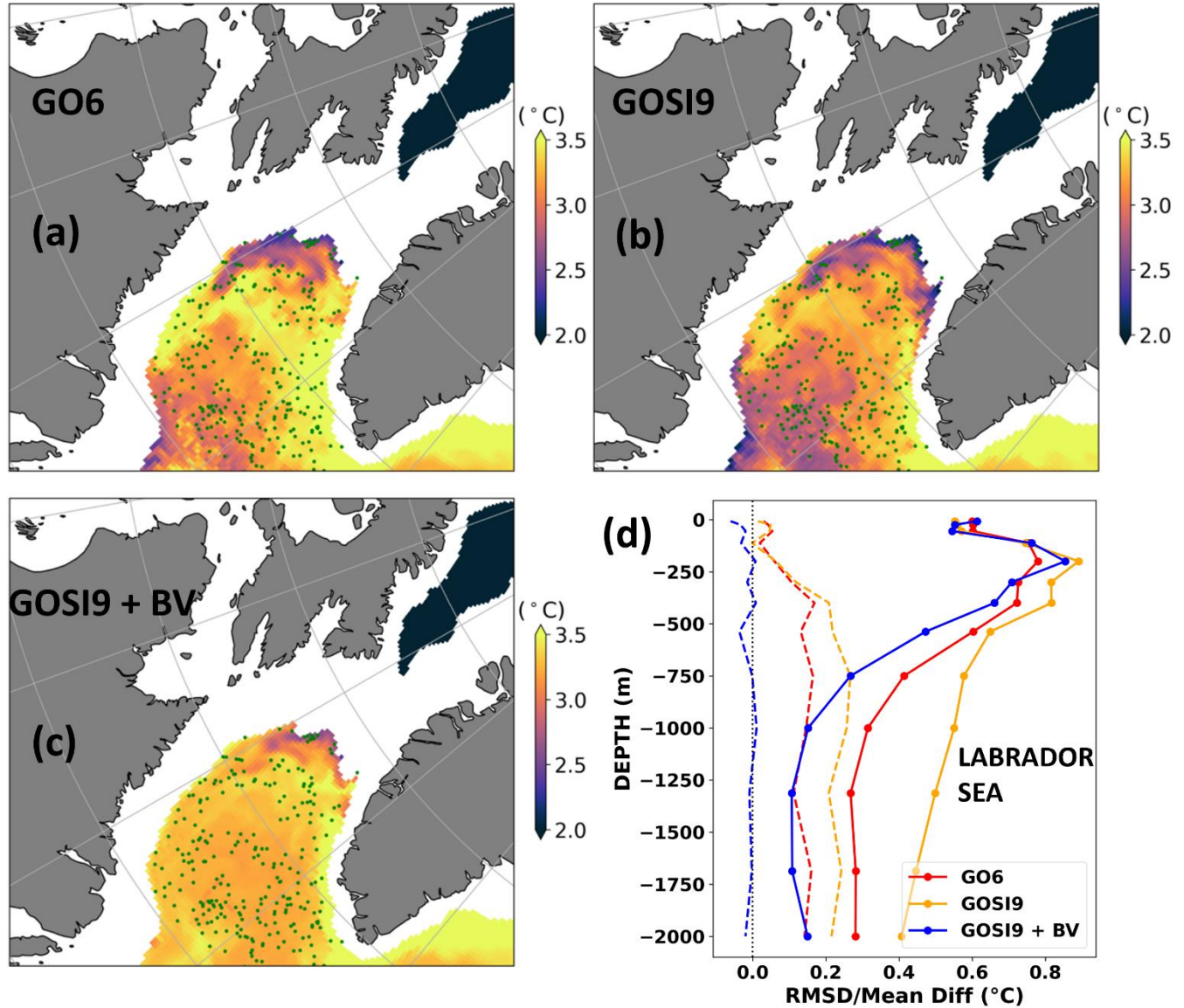
Figure 4. FOAM -ORCA025 temperature fields (°C) at 1200 m in the Labrador Sea for FOAM (a) GO6, (b) GOSI9 and (c) GOSI9 additionally applying Brunt-Väisälä verifications on the T/S increments. These are snapshots of 31 March 2019 after all runs have
