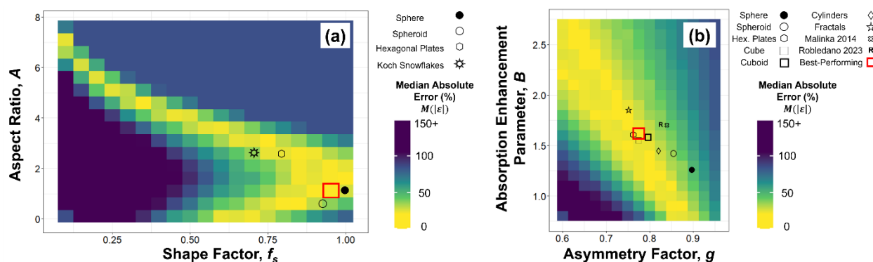
525 Figure A1: Heat maps depicting median r_{opt} absolute retrieval error for SNICAR (a) and TARTES (b) as a function of shape parameters for the R_{1064} retrieval technique. The best-performing combination tile for each technique is boxed in red. For TARTES, the optimal combination from Robledano et al. (2023) is marked with an “R”, as well as other idealized shapes evaluated in their work. For SNICAR, the locations of idealized shapes from He et al. (2017) are denoted.
