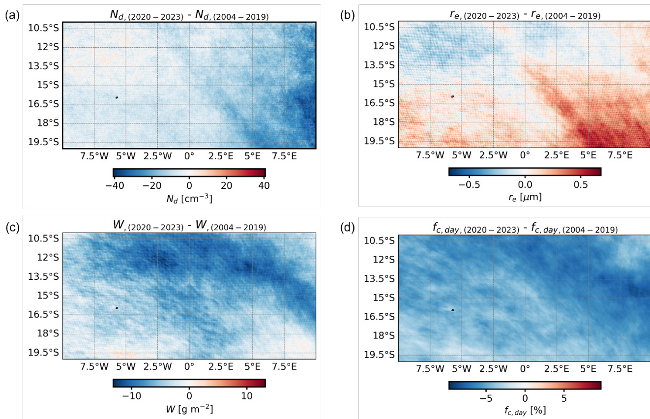
415 Figure 8: Maps of N_d (a), liquid r_e (b), W (c) and f_{c, day} (d) differences between the periods after and before 2020. Corresponding uncertainties are shown in supplementary Fig. S9.
