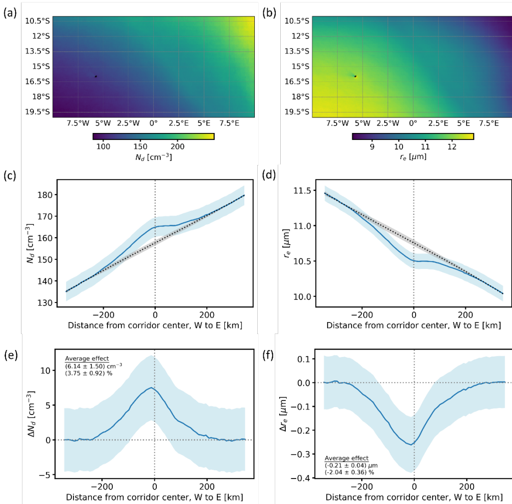
195 Figure 2: Maps of monthly time series averages of (a) N_d , and (b) liquid r_e over the study region (with corresponding uncertainties given in supplementary Fig. S1). Plots (c) and (d) show the corresponding across-corridor average distributions, with the propagated uncertainties ( 1\sigma ) in light blue shades and the no-ship scenarios in dotted curves. The standard deviation of the no-ship scenarios ( 1\sigma_{std} ) are shown in grey shades. Plots (e) and (f) show the corridor effect, calculated as the differences between the actual distribution and the no-ship scenarios, and their combined uncertainties. The average effects, calculated from the corridor core in absolute and relative terms, are also displayed. Dotted vertical lines denote the corridor center. In plots (e) and (f) the zero lines are also shown.
