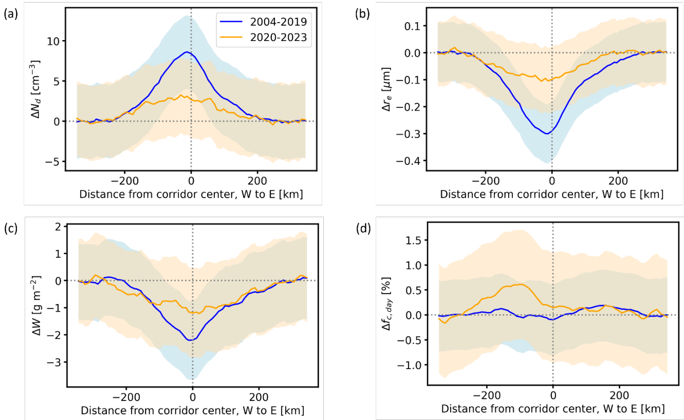
390 Figure 7: Corridor effects on N_d (a), r_e (b), W (c) and f_{c, \text{day}} (d), in the periods 2004-2019 and 2020-2023, calculated as the differences between the actual average distribution and the no-ship scenarios for these periods. The light-coloured bands show the associated propagated uncertainties ( 1\sigma ). Dotted vertical lines denote the corridor center. The zero lines are also shown.
