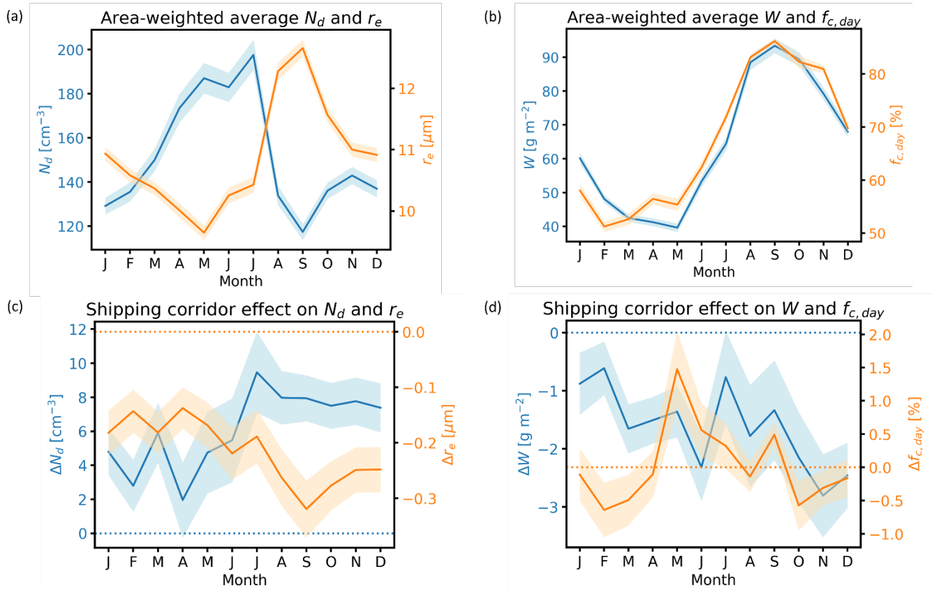
270 Figure 4: Seasonal variability of the spatially averaged (area-weighted over study domain as in Fig. 1) N_d and liquid r_e (a), W and f_{c, \text{day}} (b) and corresponding monthly corridor effects (c and d). The corridor effect values are calculated by averaging differences between the actual and the no-ship scenario values in a 150 km-wide area centered on the corridor (see also Sect. 2.3). Light-coloured bands show the uncertainties ( 1\sigma ) for each parameter. Dotted lines in (c) and (d) show the zero lines for each variable.
