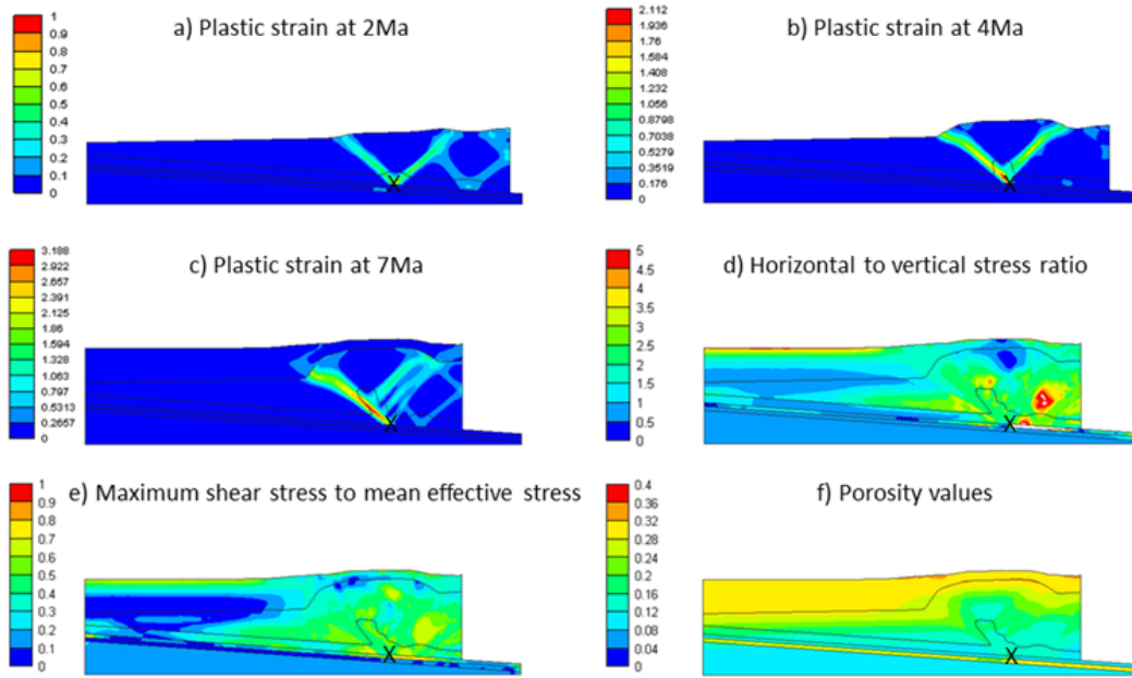
Figure 7: Progressive development of plastic strain and the final values of the \sigma_{xx}/\sigma_{zz} , \tau_{max}/p and n for the case #16 ( \beta = 4^\circ , \alpha = -1^\circ , \mu_{decol.} = 0 , and pc = 50 MPa). The black cross symbol shows the initial location of the discontinuity point over the décollement.
