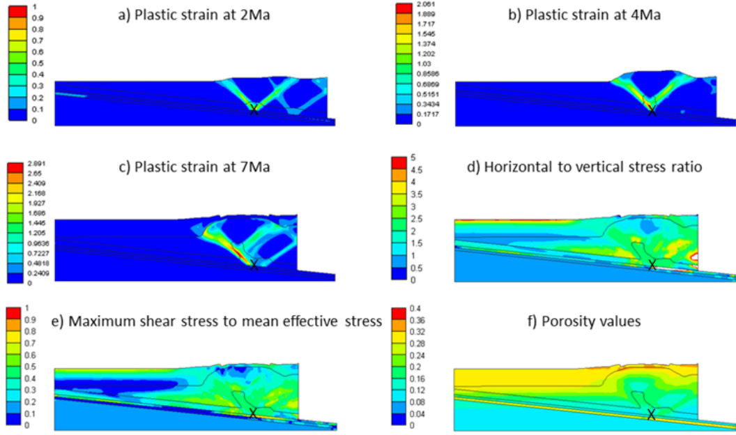
Figure 4: Progressive development of plastic strain and the final values of the \sigma_{xx}/\sigma_{zz} , \tau_{max}/p and n for the case #4 ( \beta = 6^\circ , \alpha = 0^\circ , \mu_{decol.} = 0 , and pc = 50 MPa). The black cross symbol shows the initial location of the discontinuity point over the décollement.
