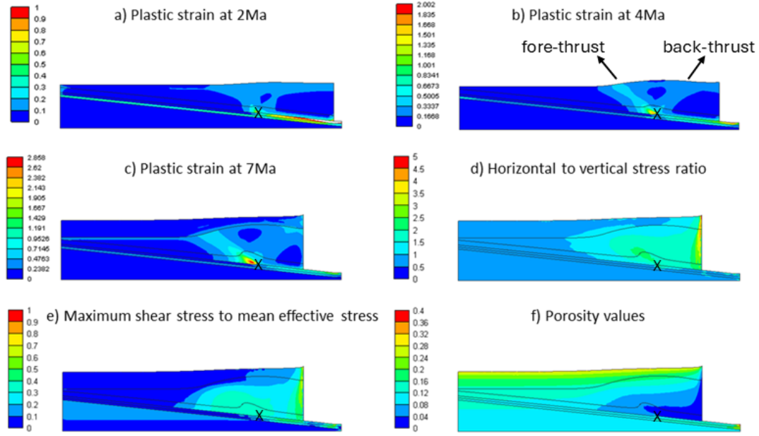
Figure 3: Results of Case #1 ( \beta = 6^\circ , \alpha = 0^\circ , \mu_{\text{decol.}} = 0 , and p_c = 2.5 MPa). A-C: Progressive development of plastic strain at 2 Ma, 4 Ma and 7 Ma, respectively. D-F: Distribution of horizontal-to-vertical stress ratio \sigma_{xx}/\sigma_{zz} , maximum shear stress-to-mean effective stress ratio \tau_{\text{max}}/p , and porosity n at 7 Ma. The black cross symbol shows the initial location of the discontinuity point over the décollement.
