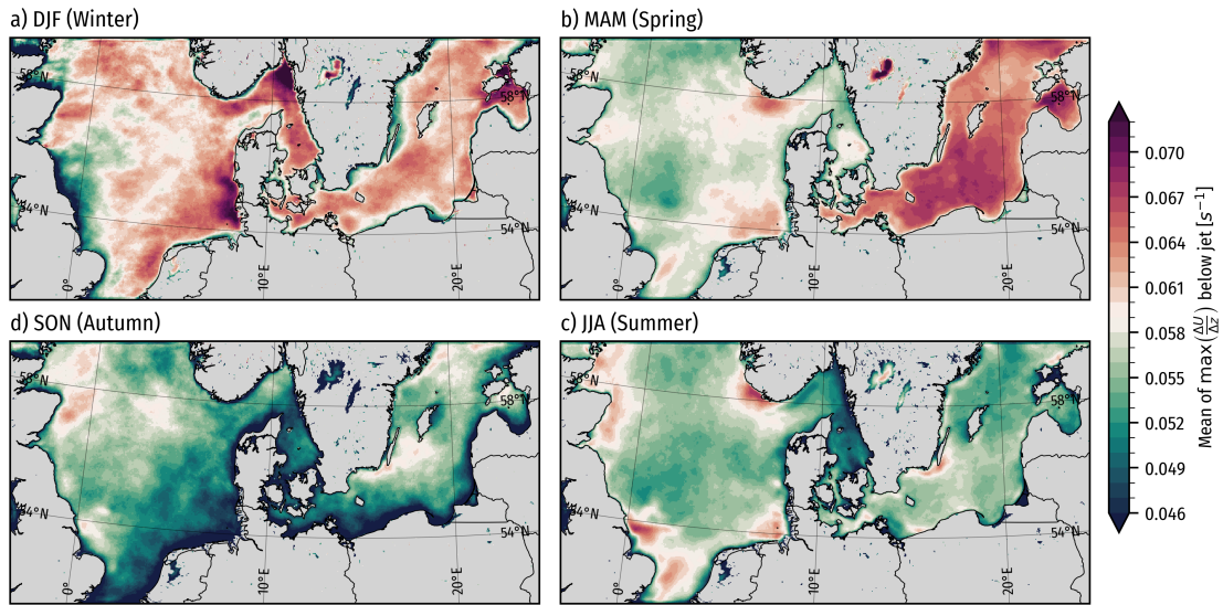
Figure F1. Mean of \max \left( \frac{\Delta U}{\Delta z} \right) in the WRF model climatology (P_CLIM) from 26 June 2019 to 26 June 2024, separated by season. Onshore, the shear is dominated by surface roughness effects, so these are greyed out to keep the focus on offshore locations.
