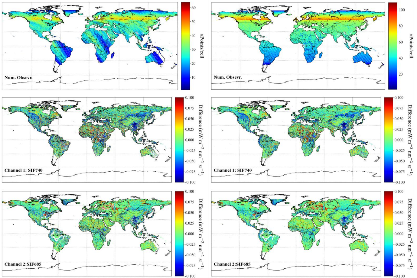
510 Figure A1. Global maps of TanSat-2 observation counts (top panels) and retrieval errors (retrieved SIF minus reference SIF) for Channel 1 (middle panels) and Channel 2 (bottom panels). Results derive from 4-day (left column) and 8-day (right column) composites at 0.05^\circ grid resolution.
