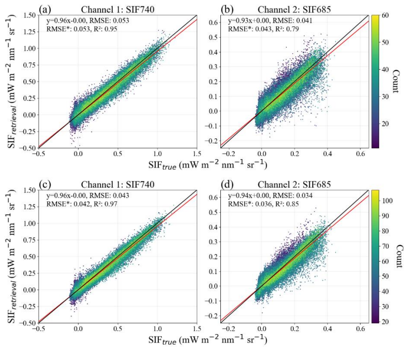
515 Figure A2. Retrieved versus reference SIF relationships for TanSat-2's two channels derived from 4-day composites (a, b) and 8-day composites (c, d). Black lines denote the 1:1 relationship, while red lines indicate linear regression fits.
