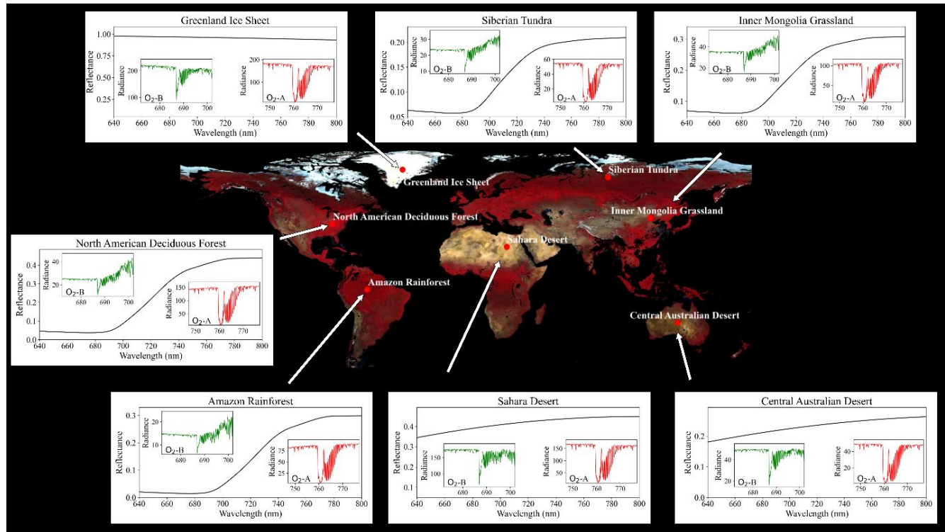
Figure 4. Global reflectance pseudo-color composite and the BOA reflectance along with simulated TOA radiance for two channels in typical regions.
