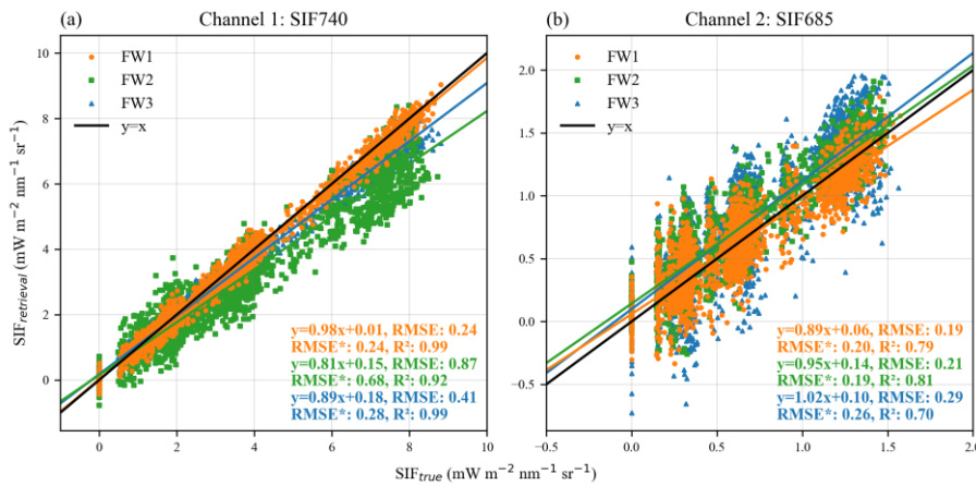
335 Figure 6. Retrieval using simulated datasets of two channels with different fitting windows: the windows for channel 1 are 747-758 nm, 759-772 nm, and 747-777 nm; the windows for channel 2 are 672-686 nm, 682-697 nm, and 672-702 nm. For demonstration purposes, only a randomly selected portion of the data is used to draw the scatter plot.
