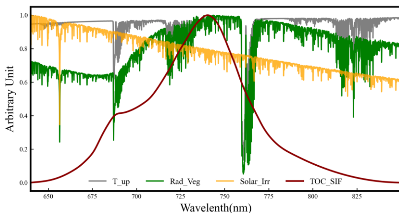
185 Figure 1. A collective set of normalized, simulated spectra at the TOA over vegetated surfaces (Rad_Veg), together with the incident solar radiance that arrives at the TOC (Solar_Irr), upward transmittance of the atmosphere (T_up), and SIF at the TOC (TOC_SIF). These spectra are presented with an SR of 0.12 nm and an SSI of 0.04 nm derived from SCOPE and MODTRAN 5 models.
