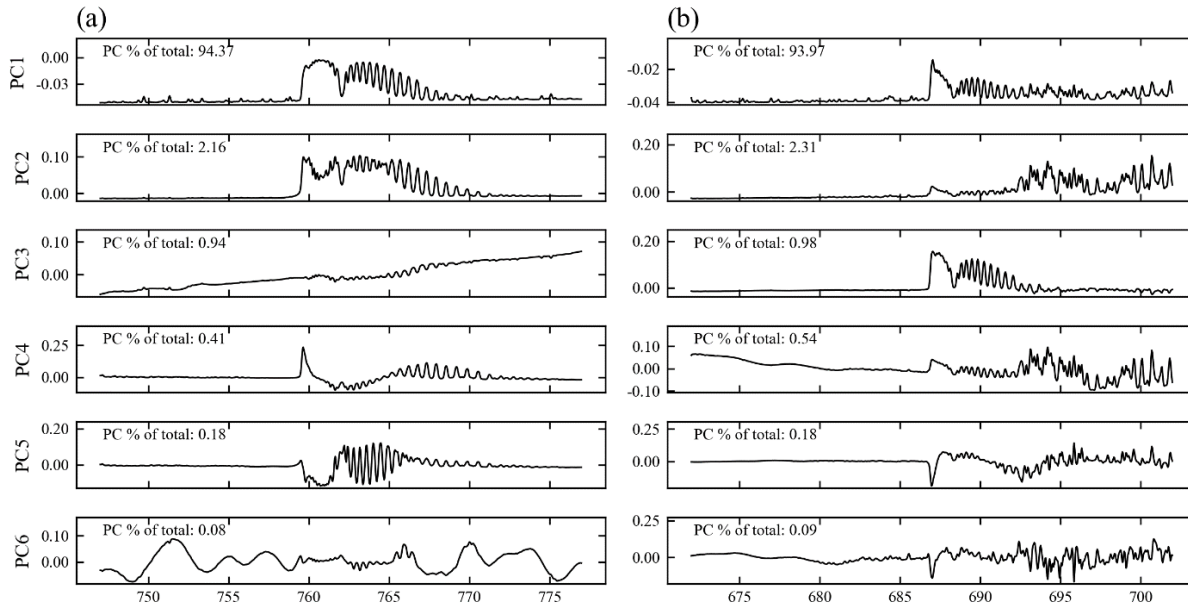
295 Figure 5. The first 6 bias vectors from the SVD of the spectral simulation training dataset in two spectral ranges: (a) 747–777 nm and (b) 672–702 nm.
