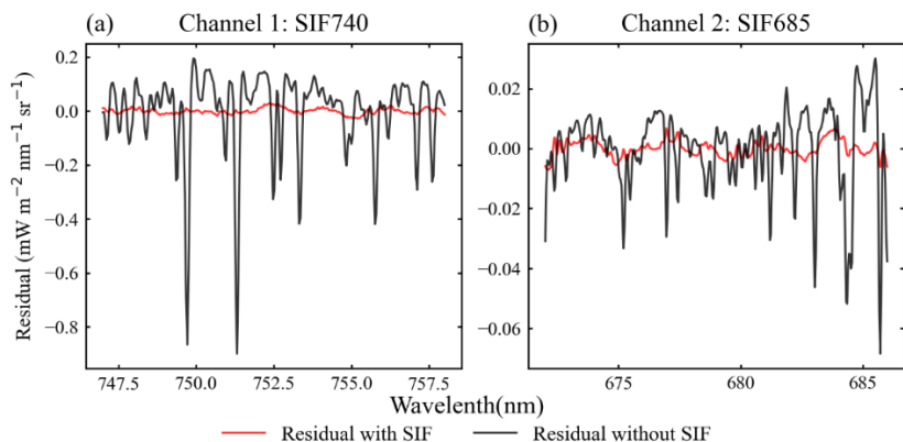
375 Figure 10. Spectral residuals between the fitted and observed TOA radiances, shown for cases where the model includes SIF (red) and excludes SIF (black) in two spectral ranges: (a) 747–758 nm and (b) 672–686 nm. (a) and (b) correspond to channels 1 and 2.
