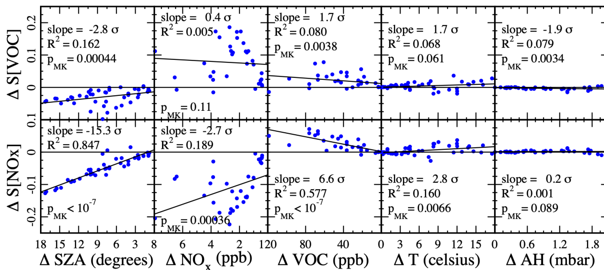
Figure 8. The change in sensitivity, ΔS NO x or ΔS VOC , induced by the change in one of the five variables, solar zenith angle (Δ SZA), NO x concentration (Δ NO x ), VOC concentration (Δ VOC), temperature (Δ T), and absolute humidity (Δ AH) for various models listed in Table 3. The scale on the abscissa appears in descending order if the corresponding variable trends downward during the winter. The slope of each trend line as a multiple of its standard deviation, the value of Pearson's R^2 , and the Mann-Kendall p -value are shown for each data set.
