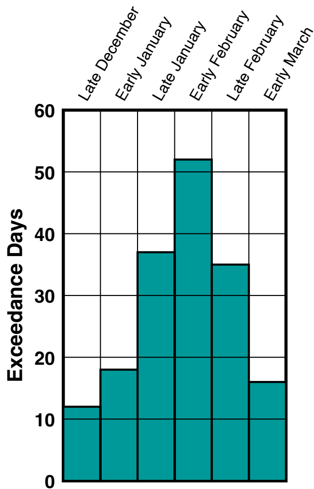
390 Figure 10. The number of days in each of the six fortnights between December 2009 and March 2020 during which the 8-hour average ozone concentration at the Ouray monitoring station (central Uinta Basin) exceeded 70 ppb.
