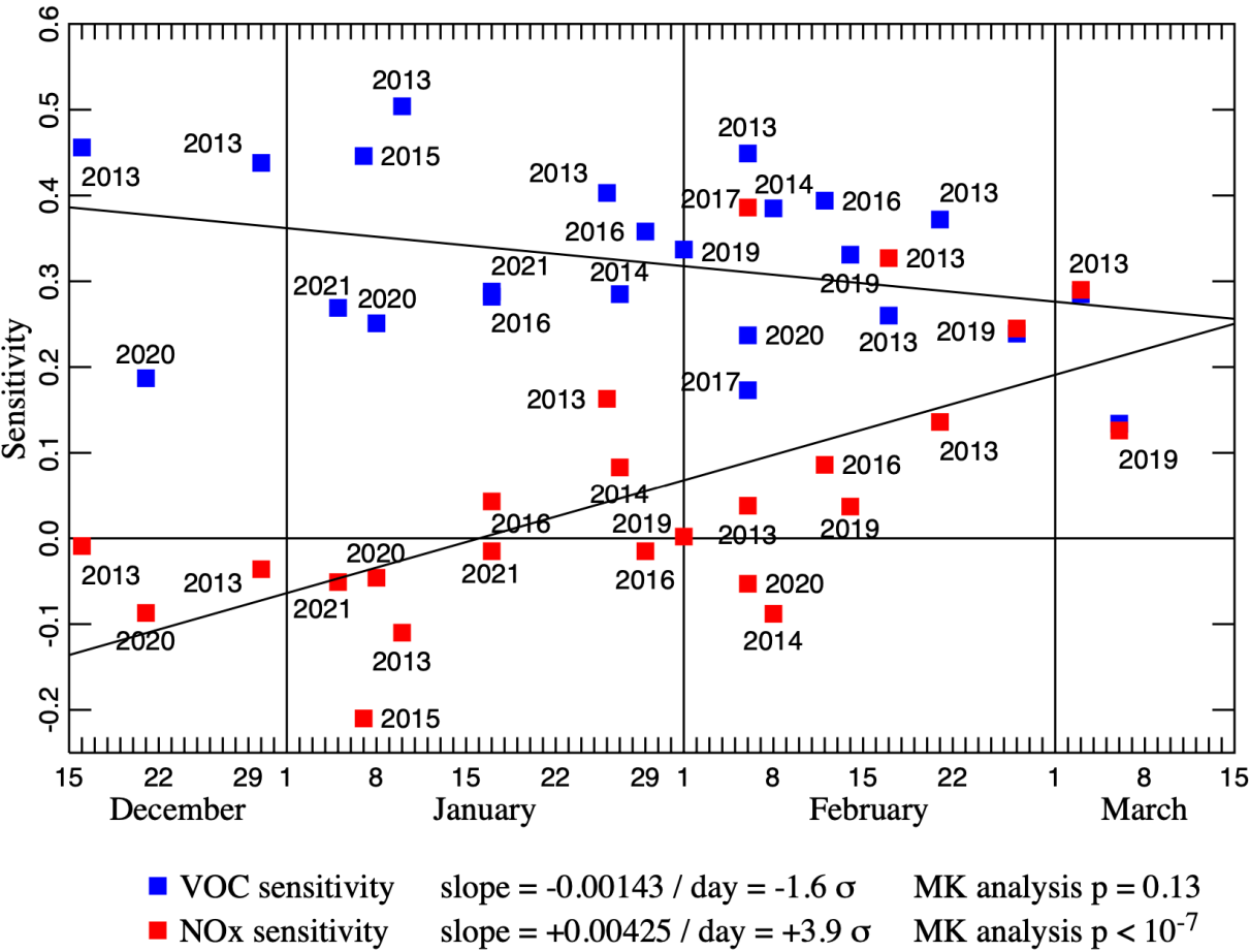
Figure 7. S_{VOC} and S_{NOx} for 24 different box model runs. Slopes of the least-squares trend lines are given both as numerical values and as multiples of the standard deviations of the slopes. The p -values from Mann-Kendall trend analyses are also shown.
