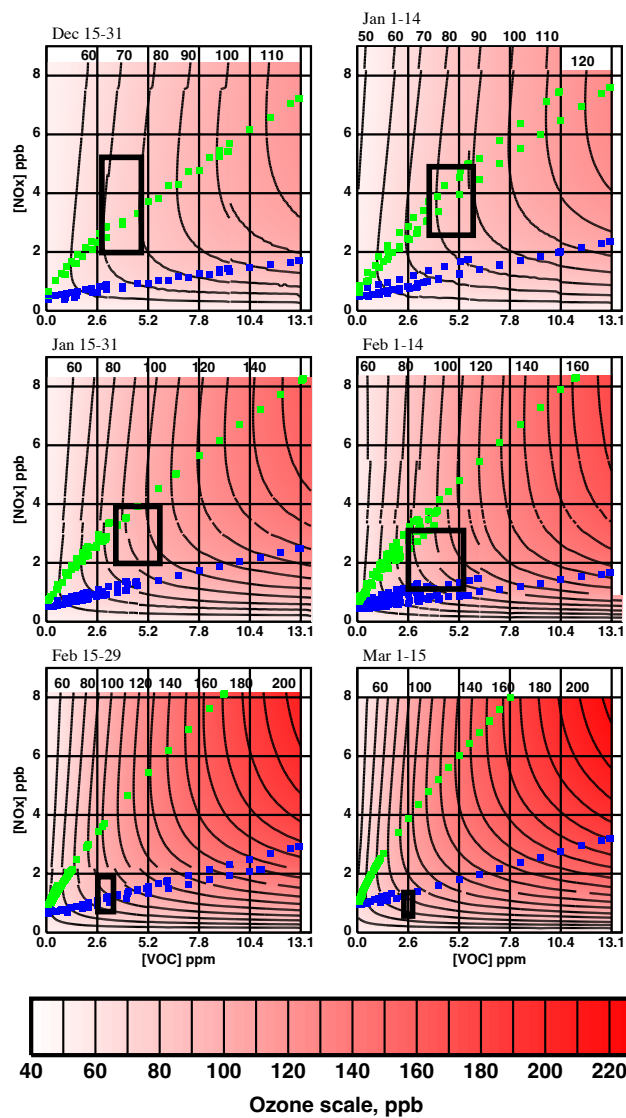
335 Figure 9. Composite ozone isopleth surfaces constructed from the 24 models listed in Table 3. Green squares define the locus of points at which S_{NO_x} = 0 . Blue squares define the locus of points at which S_{NO_x} = S_{VOC} . Black rectangles were derived from the 25 th -to-75 th percentile boxes in Figs. 4 and 5 and therefore display the typical ranges of VOC and NO x concentrations.
