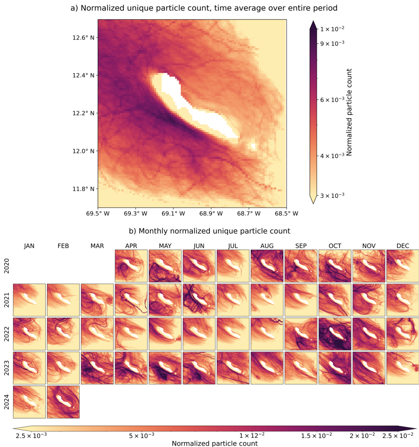
Figure 8: Normalized unique particle counts of particle trajectories around Curaçao, simulated with Scenario 1 method: (a) time-
