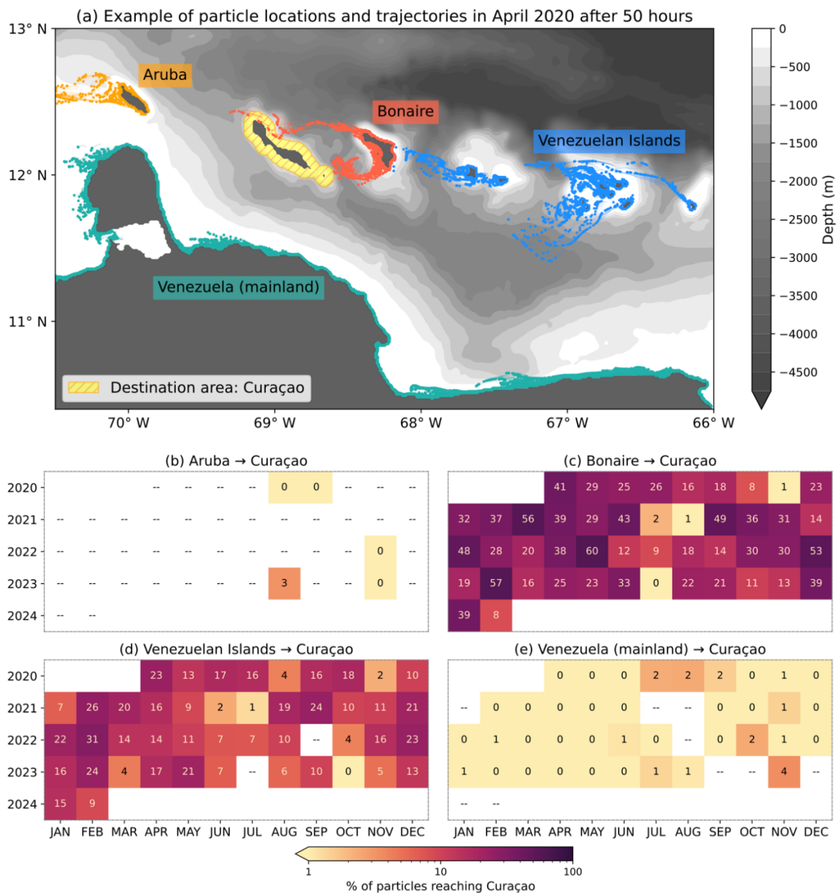
Figure 10: Connectivity matrix, generated in Scenario 3, for the period April 2020 to February 2024, showing connectivity to Curaçao from (b) Aruba, (c) Bonaire, (d) the Venezuelan Islands, and (e) the Venezuelan coastline. "--" indicates zero connectivity during the release month of the particles, although their trajectories may extend into subsequent months. (a) shows example of particle locations in April 2020, 50 hours after their initial simulation time.
