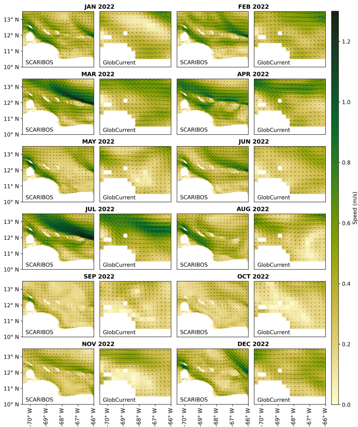
Figure 2: Comparison of surface currents of the entire domain between SCARIBOS model output and Copernicus GlobCurrent Surface (GlobCurrent) for selected 6 months in 2021. The colour scheme represents surface speed, with arrows indicating both direction (arrow shape) and magnitude (arrow size). All plots share the same colour bar and arrow scale.
