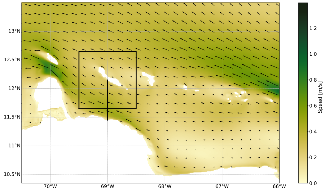
(a) Average current speed and direction, April 2020-March 2024
