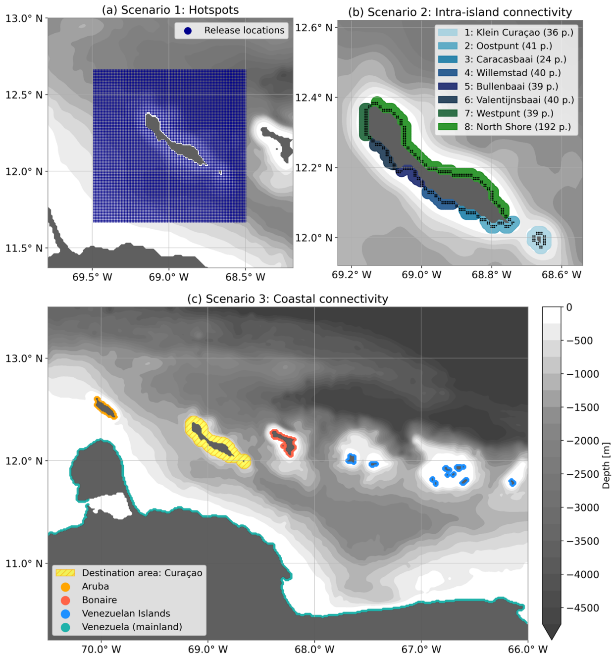
305 Figure 54: (a) Particle release locations for Scenario 1, identifying potential hotspots. (b) Particle release locations (dots) for Scenario 2, colour-coded for by coastal zone, with surrounding areas indicating potential destinations for connectivity analysis. (c) Particle release locations (dots) for Scenario 3, colour-coded by coastlines of each source area. The destination area highlighted around Curaçao represents the region within which is destination area where particles are tagged as if they reaching Curaçao coast .
