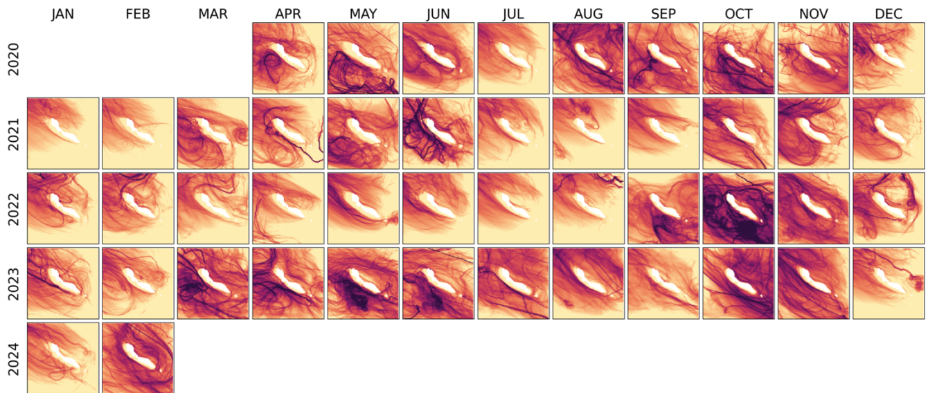
b) Monthly normalized unique particle count
