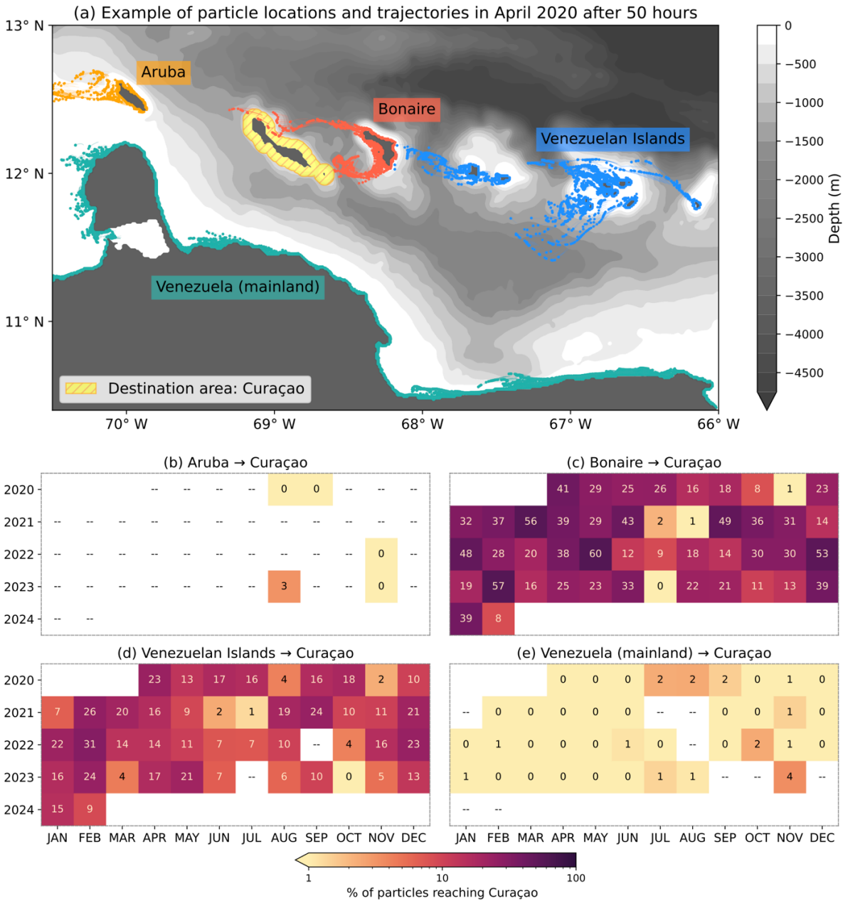
Figure 109: Connectivity matrix, generated in Scenario 3, for the period April 2020 to February 2024, showing connectivity to Curaçao from (ba) Aruba, (cb) Bonaire, (de) the Venezuelan Islands, and (ed) the Venezuelan coastline. "--" indicates zero connectivity during the release month of the particles, although their trajectories may extend into subsequent months. (a) shows example of particle locations in April 2020, 50 hours after their initial simulation time.
