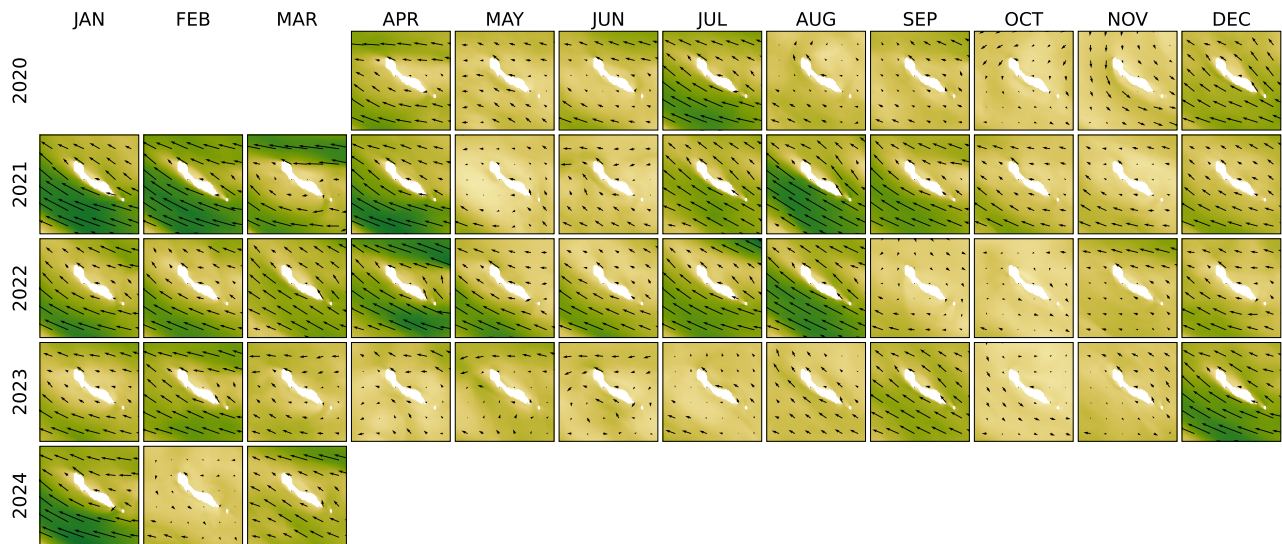
(b) Monthly average current speed and direction around Curaçao
