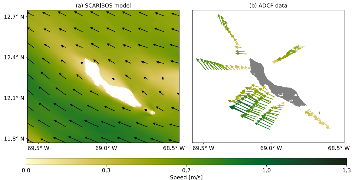
Figure 43 : Comparison of surface currents in the confined area around Curaçao between (a) SCARIBOS model output and (b) observations from a vessel-mounted Acoustic Doppler Current Profiler (ADCP) installed on RV Pelagia during the 64PE529
