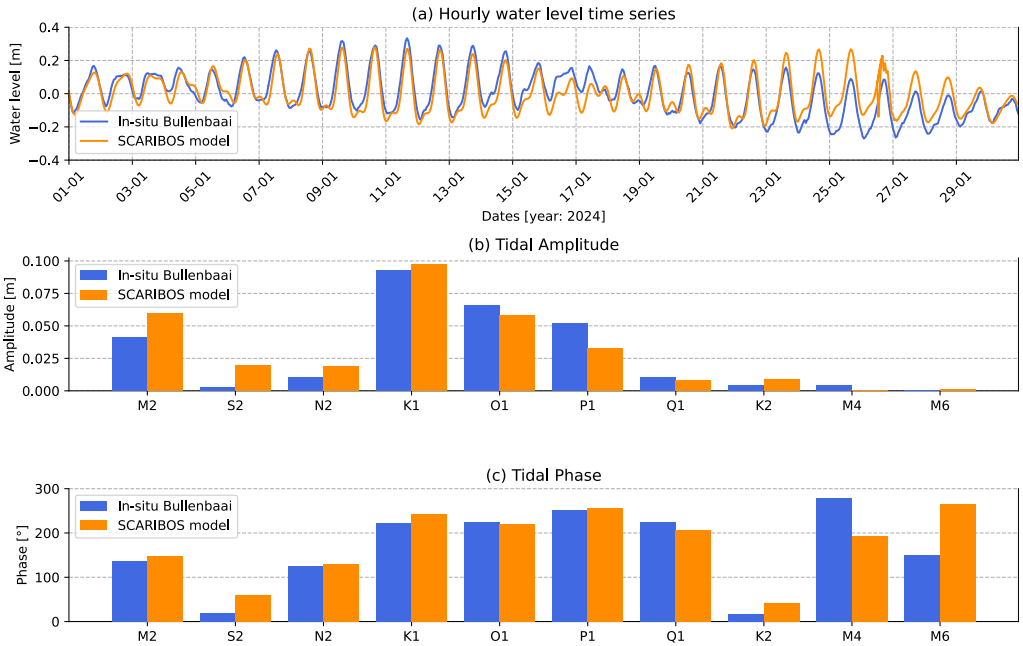
Figure 32: Comparison of water levels at Bullenbaai (12.187° N, 69.019° W) between SCARIBOS model output (in orange) and the observations from a bubbler sensor (in blue) for the entire month of January 2024. (a) Hourly comparison of water levels over the month. (b) Comparison of tidal amplitude for the 10 main tidal constituents (M2, S2, N2, K1, O1, P1, Q1, K2, M4, M6). (c) Comparison of tidal phase for these constituents.
