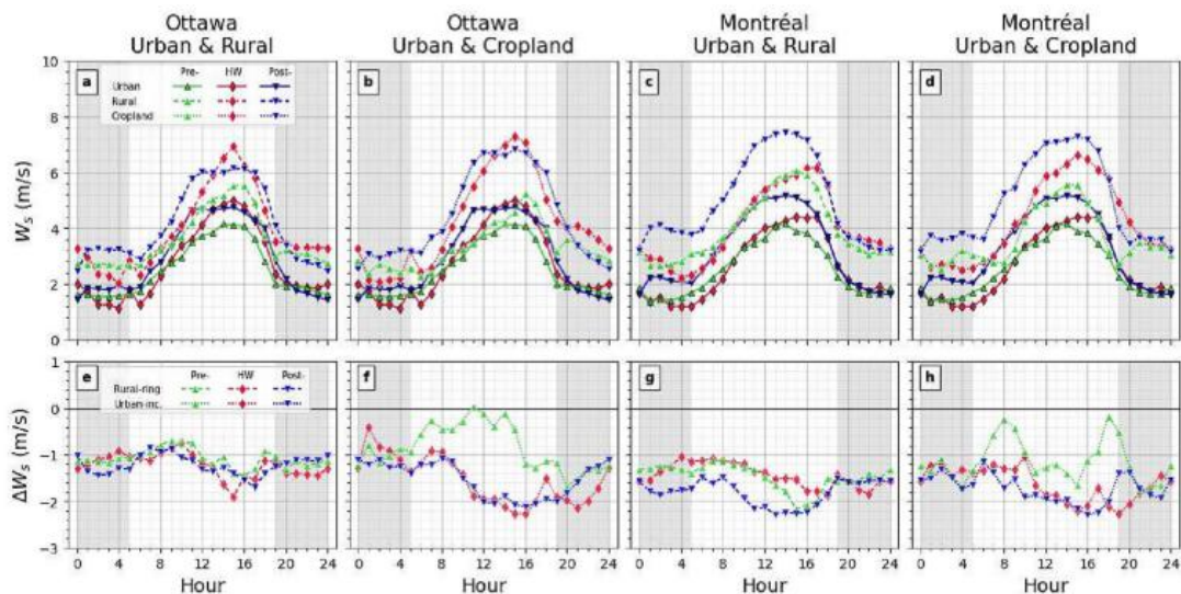
Figure R5: Diurnal profiles of the spatial-averaged (a-d) 10-m wind speed ( W_s ) at the urban and rural/cropland areas, and (e-h) 10-m wind speed difference ( \Delta W_s ) between the urban and rural/cropland areas. The shaded area in grey indicates the night-time hours. (Shu, et al., 2023).
