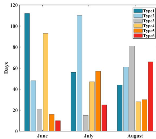
Figure R2: (a) Daily, (b) Interannual and (c) Monthly occurrence frequencies of the six SWPs in YRDUA from 2011 to 2020.
