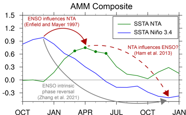
133 134 Figure 3. ERA5 SST anomalies in the northern tropical Atlantic (NTA; 40-10W, 10-20N; green line) and Niño 3.4 (blue line) regions, 135 composited on positive AMM events, which are defined here as SST anomalies in the NTA region exceeding 0.8 standard deviations 136 in March-April-May. The years 1979, 1980, 1981, 1983, 1987, 1988, 1997, 1998, 2005, and 2010 are selected by this criterion. Values 137 significant at the 95% level are marked by dots (note that none of the Niño 3.4 values are significant). The composite shows that 138 NTA events tend to be preceded by El Niño events, a well-known remote impact of ENSO (indicated by the curved red arrow; 139 Enfield and Mayer, 1997). Furthermore, there are weak La Niña conditions in the winter following the peak of the positive AMM 140 event. This has been interpreted as the NTA influencing ENSO (dashed curved red arrow; Ham et al., 2013), but some studies have 141 challenged this, including Zhang et al. (2021), who suggest that the apparent influence stems from a misinterpretation of ENSO's 142 intrinsic phase reversal (i.e., El Niño events tend to be followed by La Niña, regardless of any tropical Atlantic SST anomalies; 143 curved grey arrow). The experiments proposed for TBIMIP will allow evaluating the importance of the NTA influence on ENSO.
