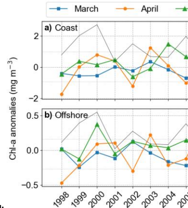
Figure 10: Spatial averages of Chl-a anomalies in coastal waters (a) and offshore (b) for the months March, April and May. The NAO index winter mean (December, January, February) is the black thin line.¶
