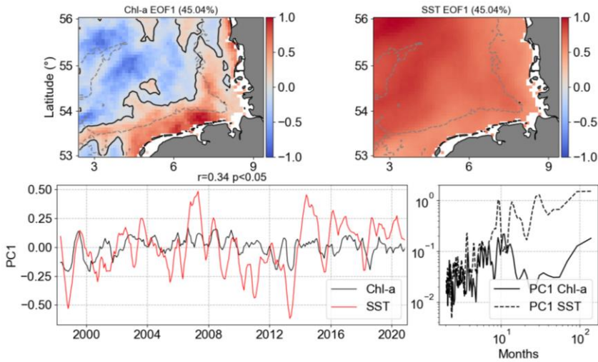
695 Figure 14: Results of MCA showing the first co-varying mode between Chl-a and SST anomalies. Top images are the co-variability mode maps (Chl-a: left; SST: right). Bottom images are the temporal co-variability PC1 (left) and the corresponding spectra (right). PC1 is shown as rolling means of 6 points to better visualize the temporal co-variability of mode 1 between Chl-a and SST anomalies.
