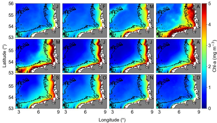
Figure 8: Monthly-averaged GlobColour Chl-a, from January 1998 to December 2020 (letters on top right). The Chl-a monthly anomalies are calculated subtracting the monthly-averaged Chl-a from the absolute Chl-a data.
