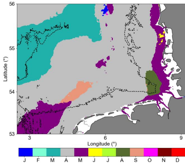
535 Figure 7: Month (colour bar from January to December) with maximum Chl-a by pixel from the monthly climatology means of Chl-a (Fig. 6; \text{mg m}^{-3} ). April (light grey) is the dominant month.
