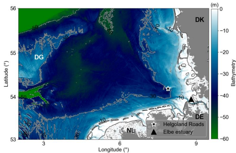
Figure 1: Bathymetry of the German Bight. Dot-dashed, solid, and dashed grey lines are 10, 30, and 50 m isobaths respectively. Areas with depths less than 5 m represented by white colour. Black star marks the location where the Helgoland Roads time series have been collected. The black triangle indicates the Elbe river estuary. The acronym DG refer to Dogger Bank; DE to Germany; DK in Denmark; and NL to Netherlands.
