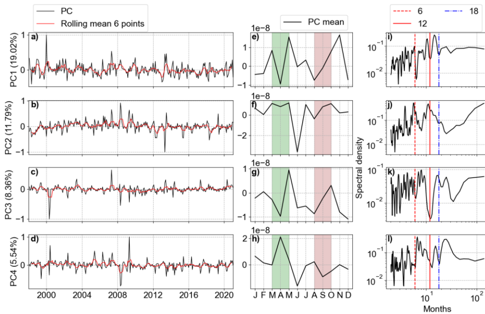
Figure 12: First four Chl-a anomalies PC. a-d) the PC amplitudes (black) with 6 point rolling means (red solid). e-h) PCs monthly means. i-l) Spectral analysis of PCs time-series. The amplitude values are max-normalized. Explained variability percentages are depicted inside parenthesis. March-April (green shaded) and August-September (pink shaded).
