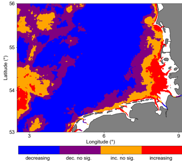
Figure 6: Trend significance of Chl-a anomalies computed with modified Mann-Kendal trend test. Pixels with p-values <0.05 are considered significant, dec. no sig.= decreasing not significant, inc.no sig. = increasing not significant.
