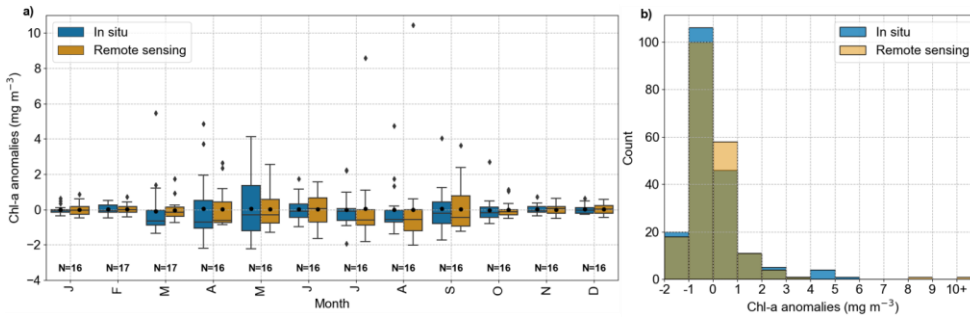
Figure 3: a) Boxplots and b) distributions of remote sensing (orange) and in-situ (blue) monthly Chl-a anomalies. The shaded areas in b) are the superimposition of in situ and remote sensing bars.
