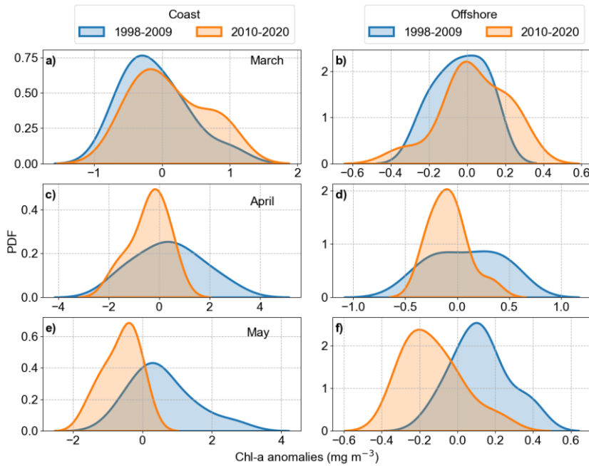
575 Figure 10. Probability Density Function estimated from 1998-2009 (blue) and 2010-2020 (orange) for the Chl-a anomalies in March, April and May in the coastal and offshore areas of the German Bight.
