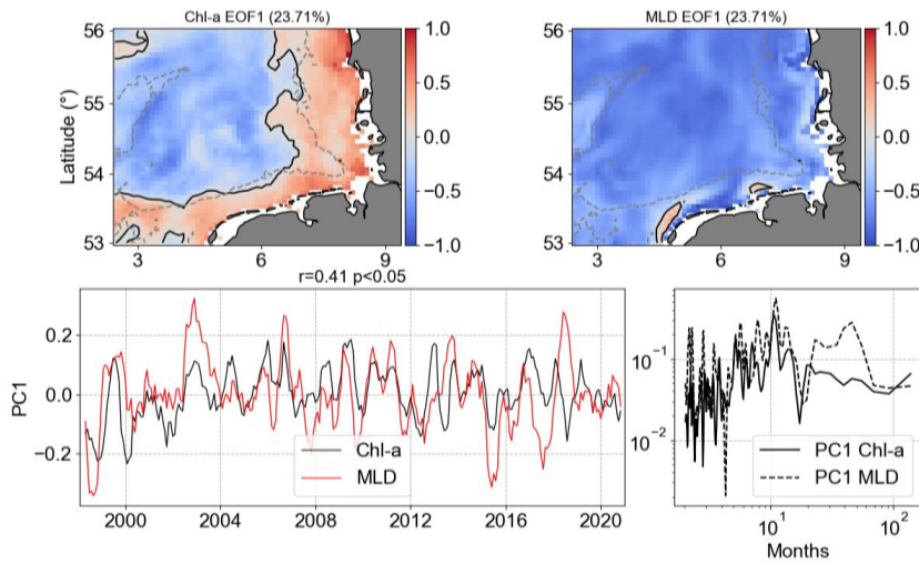
Figure 15: Results of MCA showing the first co-varying mode between Chl-a and MLD anomalies. Top images are the co-variability mode maps (Chl-a: left; MLD: right). Bottom images are the temporal co-variability PC1 (left) and the corresponding spectra (right). PC1 is shown as rolling means of 6 points to better visualize the temporal co-variability of mode 1 between Chl-a and MLD anomalies.
