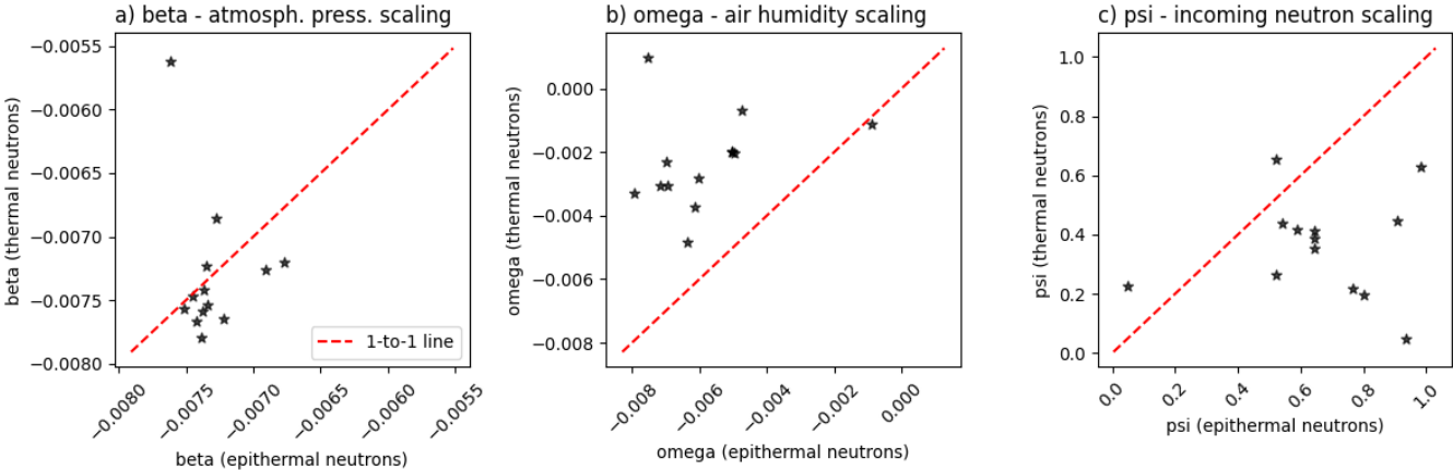
Figure 6: Results of scaling parameters, namely a) beta, b) omega, and c) psi, for thermal neutron counts using bare counter tubes against epithermal neutron counts using a moderated tube. Moderated i.e. epithermal counts are commonly used for soil moisture determination with CRNS.
