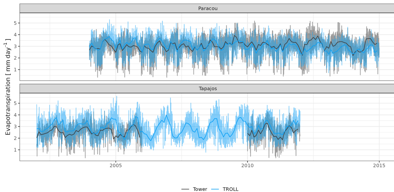
Figure A8: Daily and monthly total of evapotranspiration for Paracou and Tapajos. Dark lines are the monthly means, semi-transparent lines are the daily means variations.
