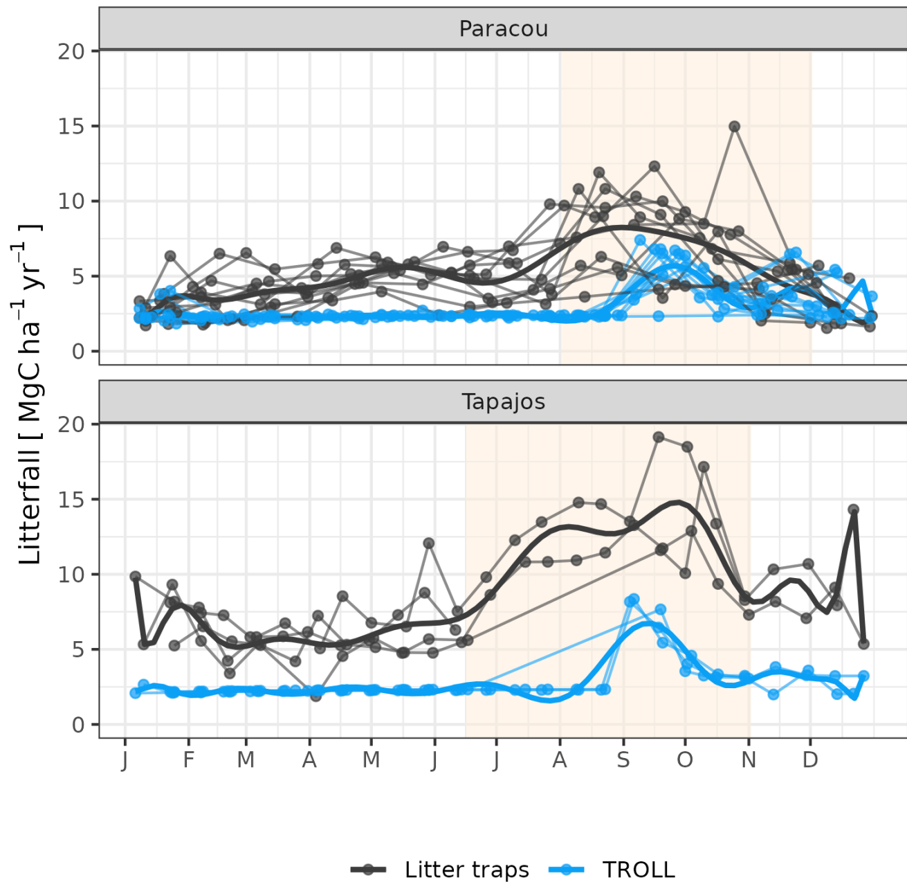
Figure 7: Litterfall annual cycle from fortnightly litterfall fluxes at Paracou and Tapajos. Each thin line represents one year with points showing values at sampling dates, the thick lines represent polynomial smoothing among years, and the vertical yellow bands in the background correspond to the site's climatological dry season. Simulated values correspond to the last 10 years of 20-year simulations starting from the end-state of 600-year regeneration from bare ground with calibrated parameters at each site.
