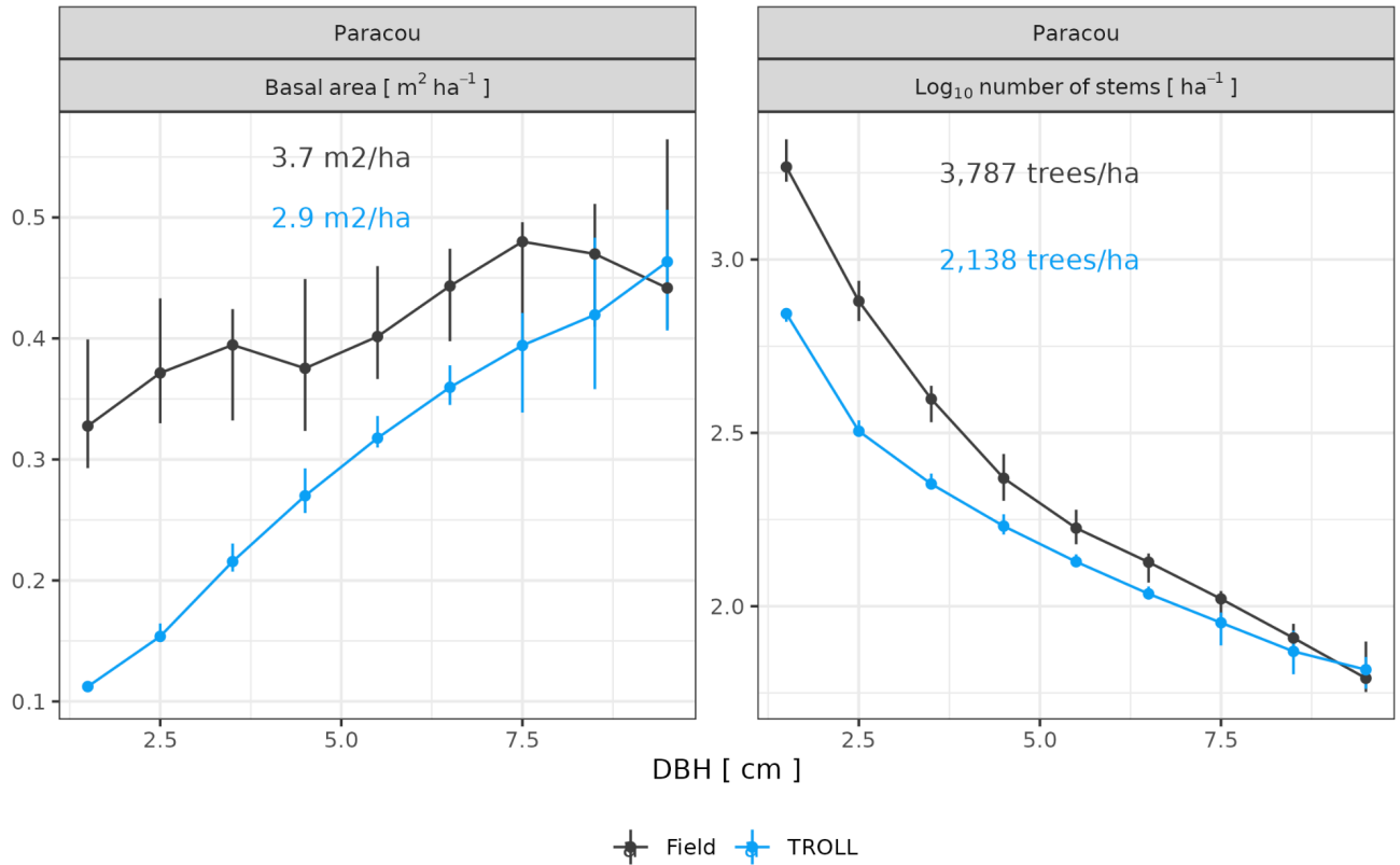
Figure 3: Understory tree size structure at Paracou, expressed in terms of basal area distributions (left) and number of stems (right) per 1 cm-dbh classes. The figures compare distributions simulated by TROLL 4.0 in blue and field inventory observations in black. Simulated values and their confidence intervals correspond to the end-state of simulations of ten 4-ha 600-year regeneration from bare ground. Confidence intervals at 95 % are shown with error bars and are based on variations among plots (9 plots of 1 ha) for the observations. Simulated (blue) and observed (black) total basal area (left) and densities (right) for trees with dbh >1 cm and < 10 cm are also provided. To the best of our knowledge, similar data was not available in Tapajos.
