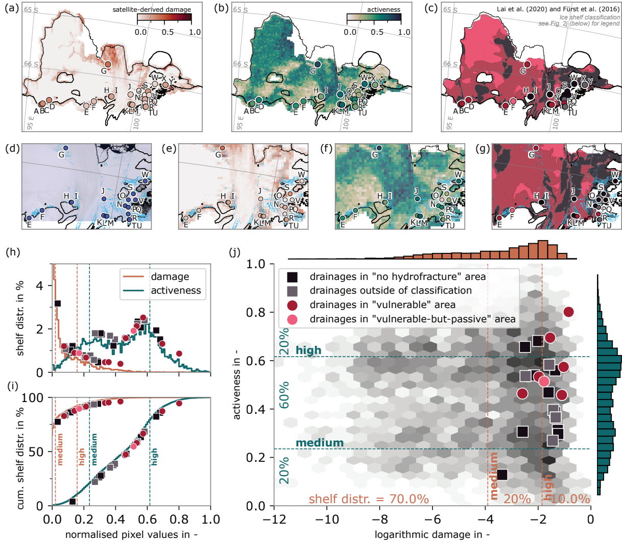
Figure 2. Spatial occurrence of observed lake drainages on Shackleton ice shelf. a) presents the satellite-derived damage and b) the activeness metrics, both for the 2019/20 melt season. c) shows the comparison to vulnerability to hydrofracturing estimates of Lai et al. (2020); Fürst et al. (2016). Panels d)-g) show zoomed section around the glaciers on the ice shelf, with d) maximum lake extent and e)-g) the same as a)-c). The superimposed coloured dots display the location of observed drainage events, the colour of each dot represents the respective value at the drainage location for the respective melt season in which it occurred. Thick/thin black line: Grounding and Shelf coastline from MEaSUREs data (Gerrish et al., 2022). Panel h) and i) show the distribution and the respective cumulative shelf distribution of satellite-derived damage and activeness together with the drainage events and in which area they were found. Panel j) presents a comparison between satellite-derived damage (in logarithmic scale), activeness, observed drainage and vulnerability to hydrofracturing estimates of Lai et al. (2020); Fürst et al. (2016).
