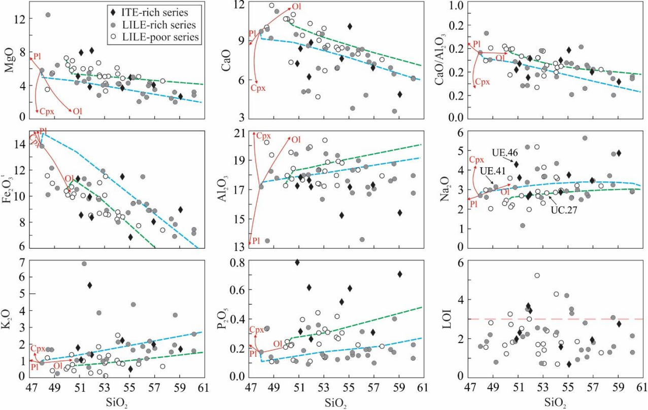
200 Figure 2: Major element oxides vs. SiO 2 variation diagrams for the LILE-poor, LILE-rich, and ITE-rich series from the UDMA. For details of the variation diagrams also see Figs. S3.a-c. The red solid lines with arrows indicate the effect of 20% fractional crystallization of olivine (Ol), clinopyroxene (Cpx), and plagioclase (Pl) on the whole-rock compositions (calculated using MagPath spreadsheet software; Mayborn and Leshner, 2011). Blue dashed line is the calculated liquid line of descent by 83% fractional crystallization of 0.18 olivine + 0.41 clinopyroxene + 0.40 plagioclase + 0.01 apatite, followed by 17% fractional crystallization of 0.05 olivine + 0.31 clinopyroxene + 0.48 plagioclase + 0.16 Ti-magnetite. Green dashed line denotes the calculated liquid line of descent by 75% fractional crystallization of 0.25 olivine + 0.41 clinopyroxene + 0.33 plagioclase + 0.01 Ti-magnetite, followed by 25% fractional crystallization of 0.06 olivine + 0.32 clinopyroxene + 0.46 plagioclase + 0.16 Ti-magnetite. The calculated liquid lines of descent match well with the trend defined by natural samples. These FC models imply that the LILE-poor and LILE-rich samples were derived from different parental magmas.
