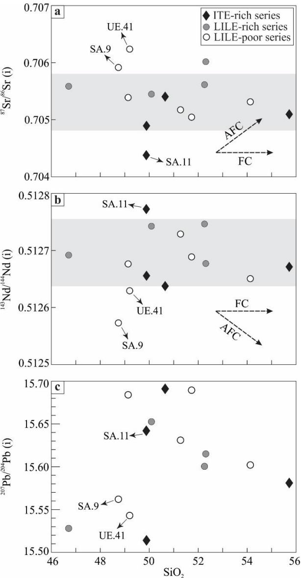
350 Figure 5: Plots of (a) ^{143}\text{Nd}/^{144}\text{Nd}(\text{i}) , (b) ^{87}\text{Sr}/^{86}\text{Sr}(\text{i}) , and (c) ^{207}\text{Pb}/^{204}\text{Pb}(\text{i}) vs. \text{SiO}_2 , as a fractionation index, for the LILE-rich, LILE-poor, and ITE-rich series mafic volcanic rocks from the central UDMA; details in the text. Gray areas/bands marks restricted Sr-Nd isotopic variation for most of the mafic rocks. One sample from the ITE-rich series plots towards less radiogenic Sr-Nd isotopic ratios (see Section 6.5 and Fig. 4.a for details). Two samples from the LILE-poor series plot towards more radiogenic Sr-Nd isotopic ratios; this is due to the higher slab components (i.e., slab + sediment) involvement (see Section 6.6 and Fig. 4.a).
