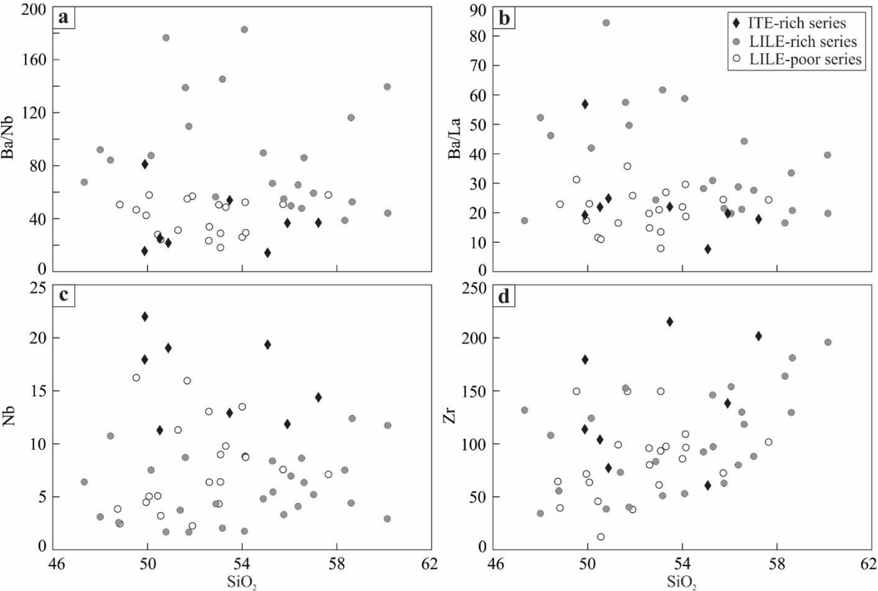
Figure 6: SiO 2 versus (a) Ba/Nb, (b) Ba/La, (c) Nb, and (d) Zr plots for discrimination of LILE-rich, LILE-poor, and ITE-rich series.
