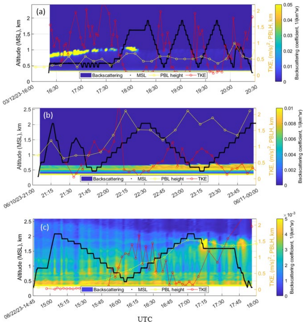
Figure 5. Aerosol backscattering overlaid with the ArcticShark flight altitude, the PBL height and TKE values on (a) March 12, (b) June 10, and (c) August 22. The y-axis is the altitude above mean sea level (MSL).
