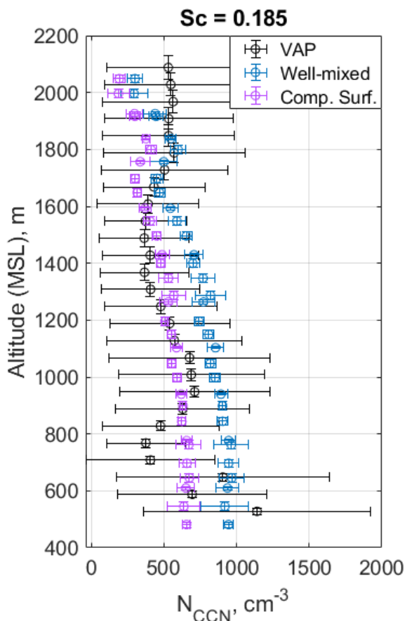
Figure 9. Cloud condensation nuclei (CCN) concentration ( N_{\text{CCN}} ) comparison with the CCNc profile from RNCCN VAP on Aug. 22, 2023. The estimated CCN concentrations were under two conditions: 1) chemical species in the CCN population were well-mixed (Well-mixed), and 2) the surface activity can be explained by a compressed-film model (Comp. Suf.).
