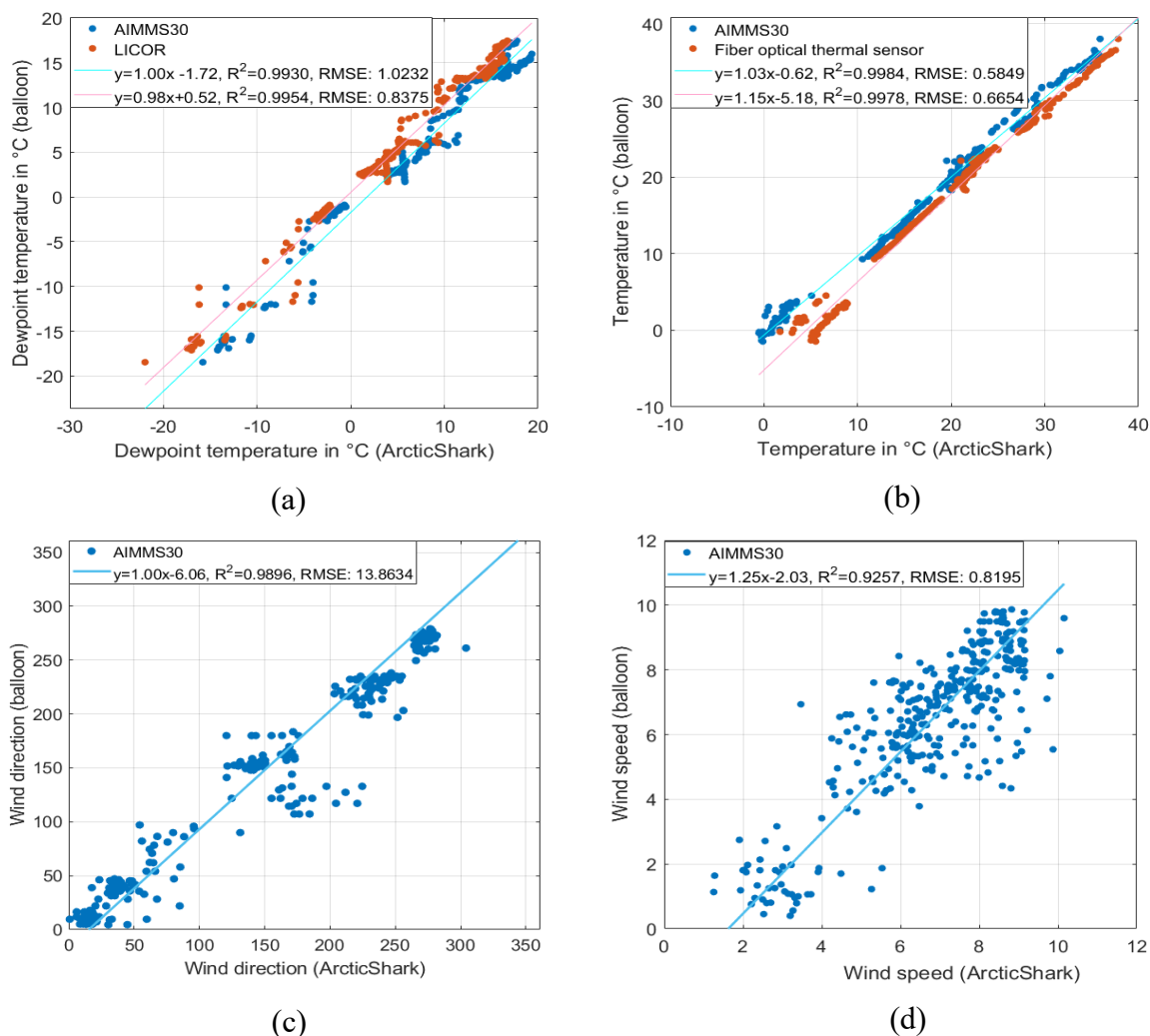
230 Figure 3. Meteorological data comparison between the ArcticShark flight (for March, June, and August) and the weather balloon 2023. (a) Dew temperature comparison, AIMMS-30 and LICOR aboard ArcticShark; (b) Temperature comparison, AIMMS-30 and the Fiber optical thermal sensor aboard ArcticShark; (c) Wind direction comparison; and (d) Wind speed comparison.
