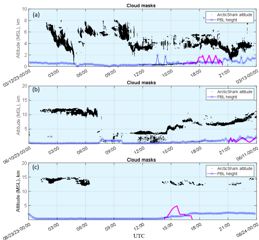
245 Figure 4. Typical ArcticShark flight altitude overlay with the cloud masks and the planetary boundary layer height on (a) March 250 12, (b) June 10, and (c) August 23. The y-axis is the altitude above the mean sea level (MSL).
