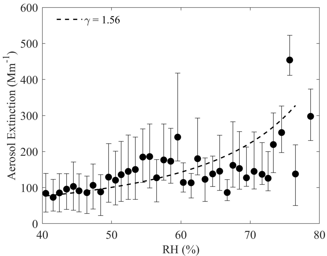
Figure S5. Humidigram of aerosol extinction at 355 nm based on the data between Aug 16 -26, 2023
