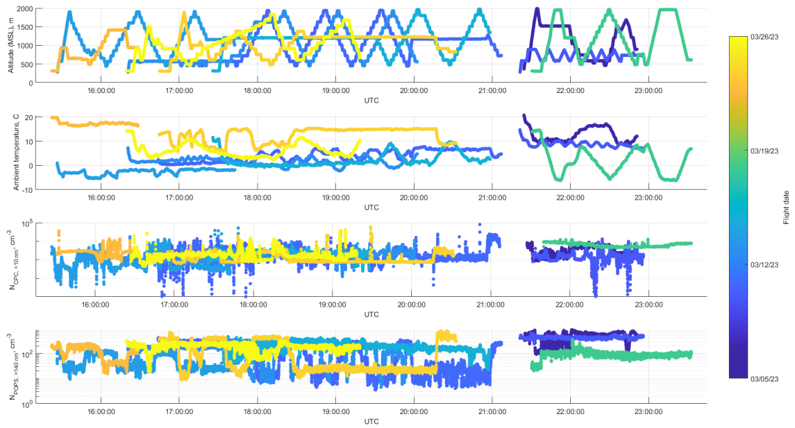
Figure S1. Time series representation of UAS altitude, ambient temperature, and aerosol number concentrations, colored by flight dates in March.
