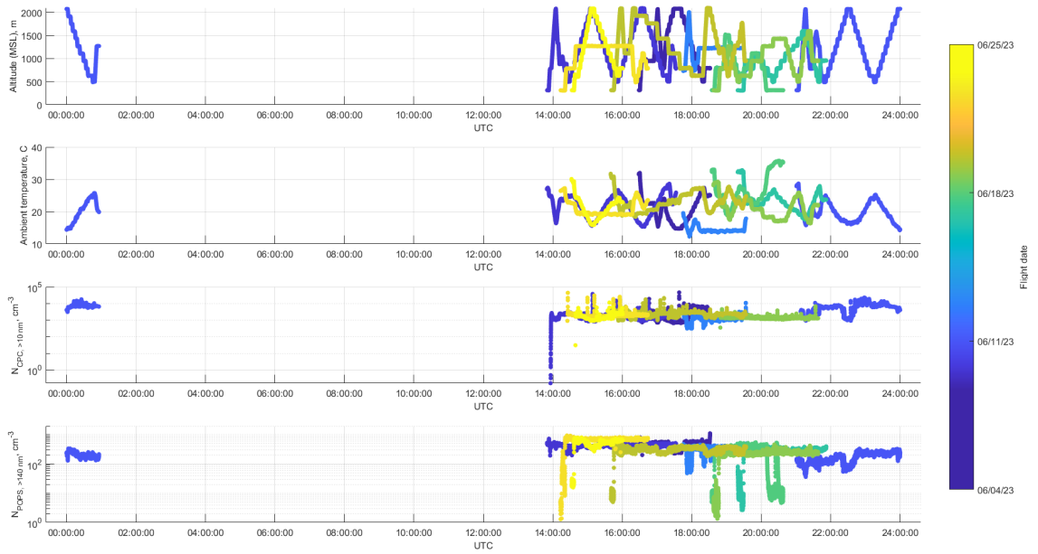
Figure S2. Time series representation of UAS altitude, ambient temperature, and aerosol number concentrations, colored by flight dates in June.
