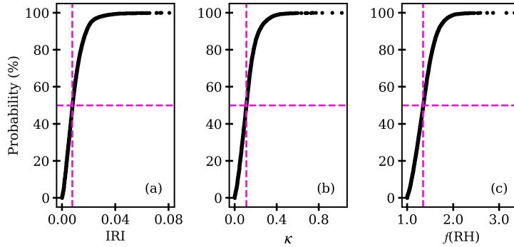
Figure 4. Cumulative probability distribution plots of retrieved (a) IRI, (b) \kappa , and (c) f(\text{RH}) derived from ACTIVATE 2020–2022 data. The intersection of the dashed magenta lines marks the medians of the data sets, which are 0.008, 0.11, and 1.34 for IRI, (b) \kappa , and (c) f(\text{RH}) , respectively.
