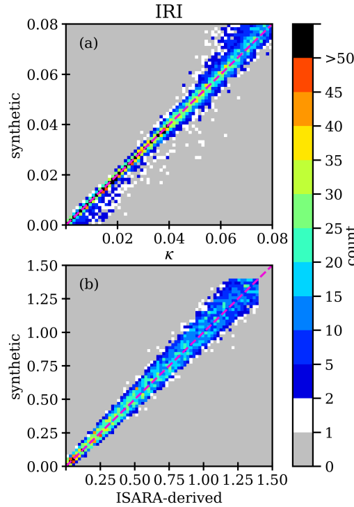
Figure 7. Heat map scatterplot of ISARA-retrieved versus synthetic (a) IRI (count = 9244, r = 0.99 , MRB= -3%, SRB = 17%, and NRMSD = 4%) and (b) \kappa (count = 9004, r = 0.99 , MRB= 3%, SRB = 20%, and NRMSD = 4%). The dashed line represents the one-to-one line and the color bar indicates density of points in a given area of the plot.
