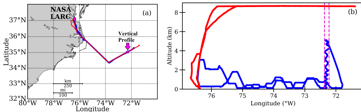
Figure 10. (a) Top-down and (b) longitudinal views of the Falcon and King Air flight tracks from Research Flight 131. The location of the “unicorn” spiral (Case 7) is bounded by the magenta box in panel (a) and by the vertical dashed lines in panel (b).
