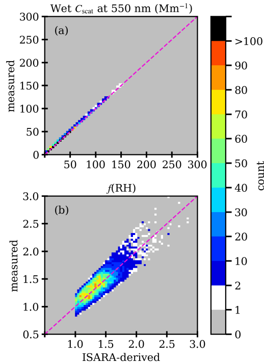
Figure 9. Heat map scatterplot of measured versus ISARA-derived in-situ values for (a) wet scattering coefficient ( C_{\text{scat}} ) at 550 nm ( r = 1.00 , \text{MRB} = 1\% , \text{SRB} = 0.1\% , \text{NRMSD} = 0.2\% ) and (b) hygroscopic amplification factor ( f(\text{RH}) ) at 550 nm ( r = 0.85 , \text{MRB} = 2\% , \text{SRB} = 9\% , \text{NRMSD} = 5\% ) from the 11914 successful ISARA retrievals that resulted from the 2020–2022 ACTIVATE data. The dashed line represents the one-to-one line and the color bar indicates density of points in a given area of the plot.
