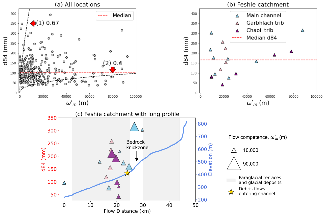
Figure 6. d84 as a function of variable \omega'_m which is a proxy for flow competence (Equation 8). (a) shows the results for our Scotland-wide dataset. The median of the entire d84 distribution is shown by the red dashed line. Black dashed lines represent power law relationships between d84 and \omega'_m with exponents of 2/3 and 0.4 (curves (1) and (2), respectively). These curves bracket the range of exponents found by Attal et al. (2015) in the Feather River basin, Sierra Nevada, California: they found exponents of 0.4, 0.53 and 0.61 best fit their data for the d100, d84 and d50 of their measured surface sediment, respectively. Median grain size d50 was fit with the exponent closest to the expected 2/3 value from experimental work and compilation of field studies (Bathurst, 2013; Whitaker and Potts, 2007). In a scenario where sediment grain size is controlled by flow competence ('transport-limited'), a power relationship between grain size and \omega'_m would be expected. (b) shows the relationship between \omega'_m and d84 for the Feshie basin which is a mountain river in the Spey catchment where 18 data points are available (see Figure 3 for the Feshie's location). The median of the Feshie's d84 distribution is shown by the red dashed line. Blue triangles show points located along the main channel, and purple and pink triangles show points located along the Chaoil and Garbhloch tributaries. (c) shows the long channel profile of the Feshie catchment with grain sizes and key geomorphic domains that influence sediment supply and transport (Towers et al., 2025). The size of the grain size markers are scaled according to the flow competence of each site. As shown in Figure 6b, grain size markers are coloured according to the tributary name. The type and location of each geomorphic landform is taken from Towers et al. (2025).
