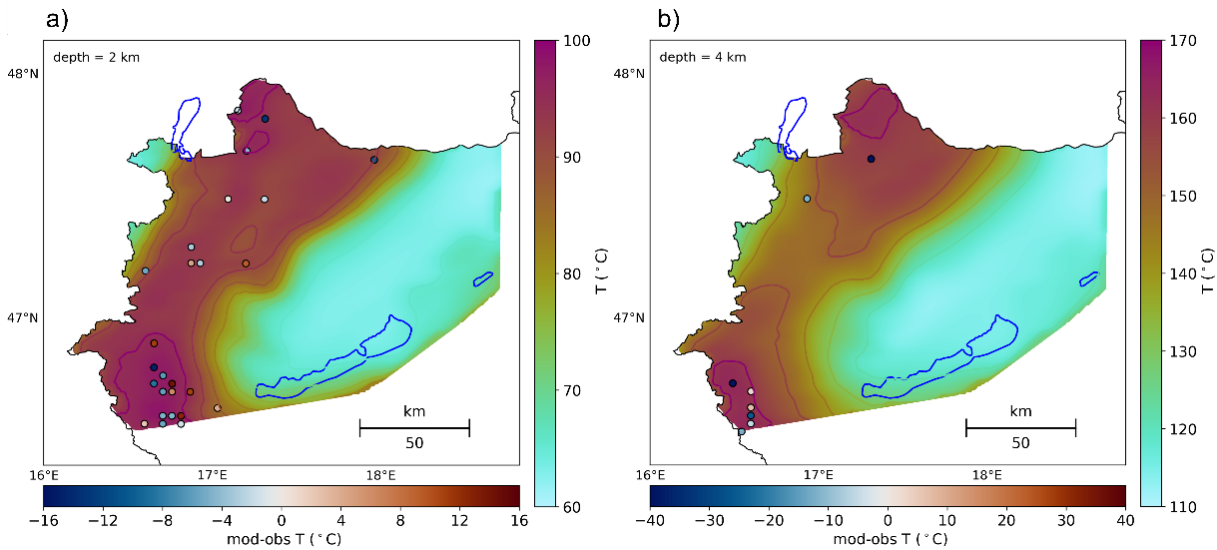
Figure 6: (a) Isodepth temperature maps predicted by the present-day posterior model at 2 km (left panel) and 4 km (right panel) depth. The misfits between modelled and observed temperatures are indicated with color-coded circles, within the depth interval of \pm 200 m.
