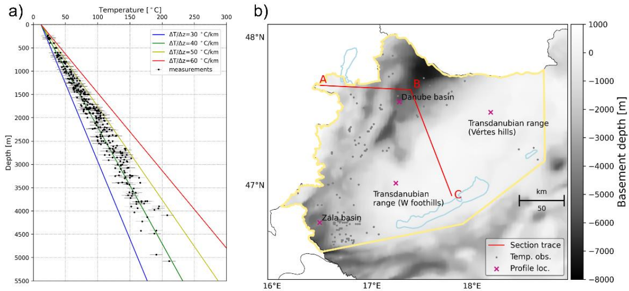
160 Figure 3: (a) Temperature dataset used for the calibration of the thermal model. Temperature measurements were obtained from the Geothermal Database of Hungary (Dövényi and Horváth, 1988; Dövényi et al., 2002) and the Geothermal Information System (Ogre, 2020). Colours represent geotherms between 30 °C/km to 60 °C/km. (b) Locations of temperature measurements (grey circles), and locations of temperature profiles (pink crosses) and section (red line) shown in Figs. 7-9, plotted on top of the pre-Cenozoic basement map (Haas et al., 2014).
