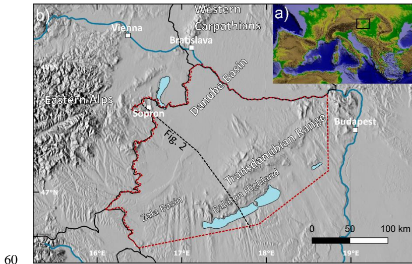
60 Figure 1: a) Topographic map of Europe based on the SRTM digital elevation model (Farr et al., 2007) , showing the outline of Fig. 1b (black rectangle) b) Geography of the study area based on the GMTED2010 elevation model (Danielson and Gesch, 2011). Red polygon denotes the extent of the thermal model (restricted to the borders of Hungary due to data availability), black lines denote state borders.
