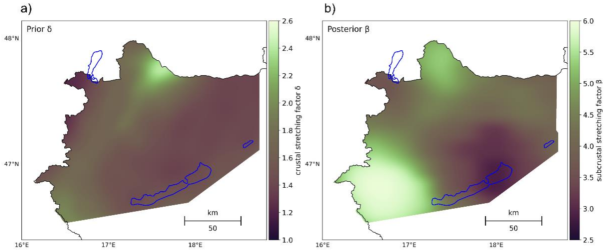
245 Figure 5: (a) Prior crustal stretching ( \delta ) and (b) posterior subcrustal stretching ( \beta ) values representing the extension of the crust and mantle lithosphere. Note that \delta shown in (a) and \beta=3 were used as input parameters for the stretching module, and \beta shown in (b) is the posterior mantle stretching factor resulting from the inversion procedure, conditioned with temperature observations.
