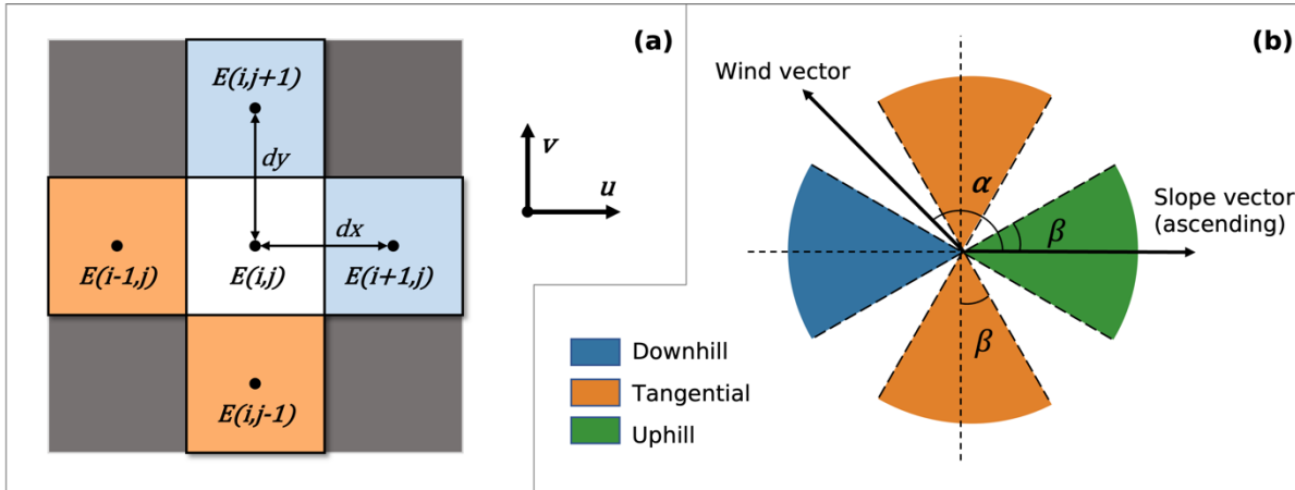
Figure 1. (a) Variables used in the calculation of the upwind slope. The elevations in the target grid, E(i,j) and the upwind grids (in orange if the wind components were positive; in light blue if the wind components were negative) were used to calculate the upwind slope components in x and y directions. (b) Methods for assigning the type of wind direction over topography. The angle between the upwind slope and the wind vector, \alpha , and the predefined cut-off angle, \beta , together determined whether the wind from an event was typical for any of the three categories of relative wind direction, namely downhill, tangential, and uphill winds.
