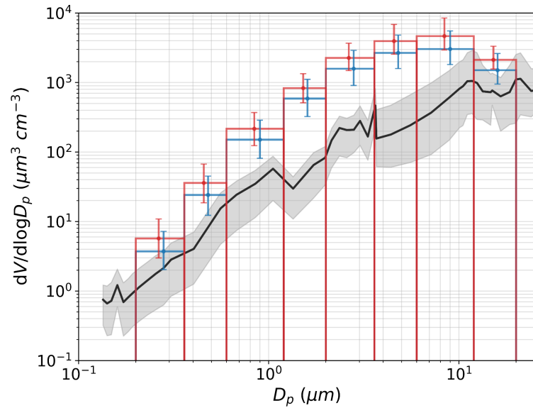
Figure 3. The black line shows the average volumetric concentration ( \mu\text{m}^3\ \text{cm}^{-3} ) of dust sampled during three Fennec flights (6 flight segments) and the grey shaded area denotes the range of values. The blue bars show the volumetric concentration ( \mu\text{m}^3\ \text{cm}^{-3} ) of dust in corresponding grids from the MONARCH reanalysis calculated from the weighted average mass concentration, with a particle density of 2,500\ \text{kg}\ \text{m}^{-3} for the finer four bins and 2,650\ \text{kg}\ \text{m}^{-3} for the coarser four bins. The error bars denote the range of values.
