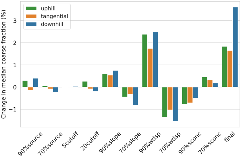
345 Figure 5. Percentage change in the median coarse fraction by wind direction type for all sensitivity runs (see Table 1) as compared to the “initial” 346 run.
