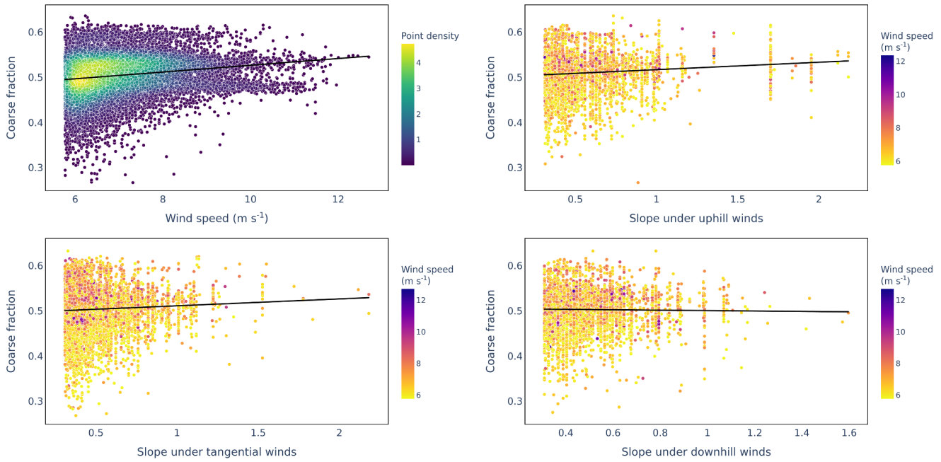
Figure 6. Scatter plots and linear trend lines of relationships between the coarse fraction of surface dust concentration in fresh emissions and the wind speed and the slope under three different wind directions. In the upper left panel for wind speed, the color-codes present the number of overlapping data points. In the other three panels for slope, the color of each scatter point represents the associated wind speed for each dust event.
