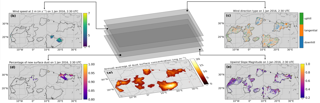
237 238 Figure 4. Schematics showing the procedures for screening the 10-year dust reanalysis data for fresh dust emissions. First, dust sources were 239 assigned to regions where the annual average of dust surface concentration is among the top percentile (i.e., 20% as shown in (a)) of all values 240 across the study domain of North Africa. Subsequently, additional screening criteria were applied simultaneously to events that occurred within 241 these dust sources. These criteria include (b) high wind speed, (c) wind direction over topography, (d) high increase in dust surface concentration, 242 and (e) steep slope. Maps (b–e) are examples of filters used in the “initial” run (see in Table 1) for 1 January 2016, at 2:30 UTC.
