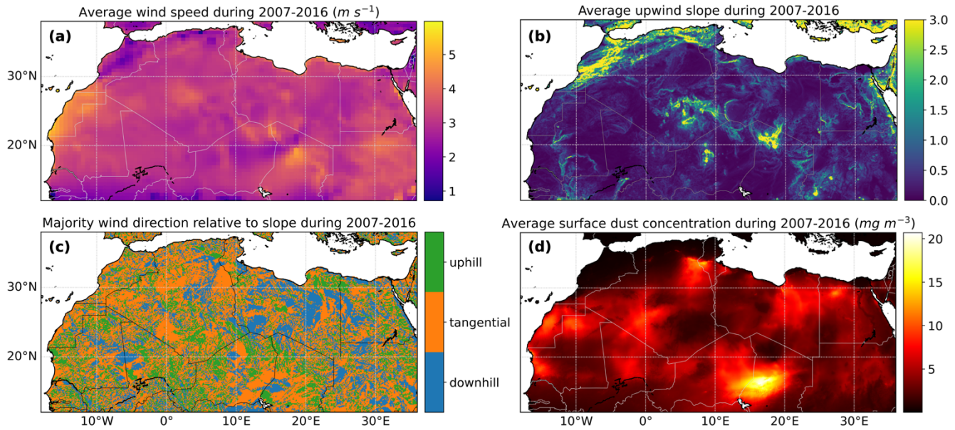
188 Figure 2. General spatial patterns of (a) 2m wind speed from the MERRA-2 reanalysis, (b) calculated upwind slope, (c) derived wind direction 189 type relative to slope using cut-off angle of 10^\circ , and (d) MONARCH total dust concentration at ground surface from 2007 to 2016. The average 190 values are shown for wind speed, upwind slope, and dust surface concentration, and the most frequent types are shown for the relative wind 191 direction.
