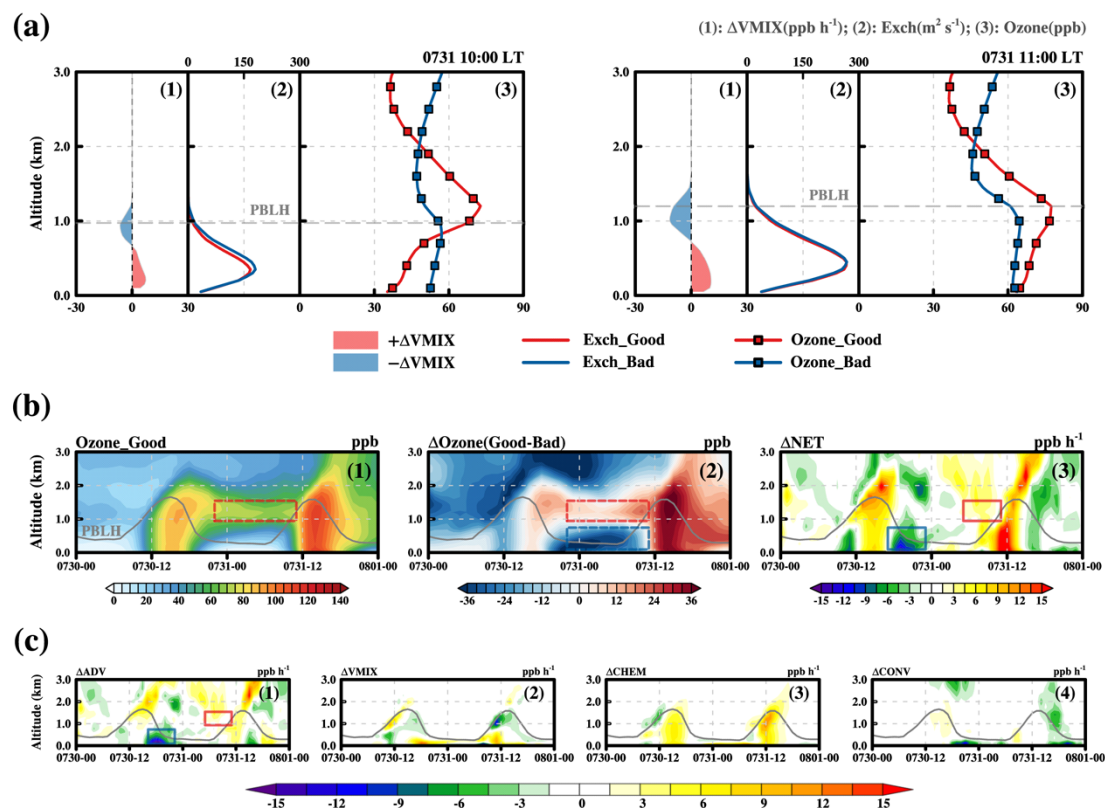
Figure 5: (a) Profiles of (1) \Delta VMIX, (2) exchange coefficient and (3) ozone at 10:00 and 11:00 on July 31; (b) vertical distributions of (1) ozone good and the changes in ozone [(2) \Delta Ozone] and NET [(3) \Delta NET]; (c) vertical distributions of the changes in the ozone contribution of each process [(1) \Delta ADV; (2) \Delta VMIX; (3) \Delta CHEM; (4) \Delta CONV].
