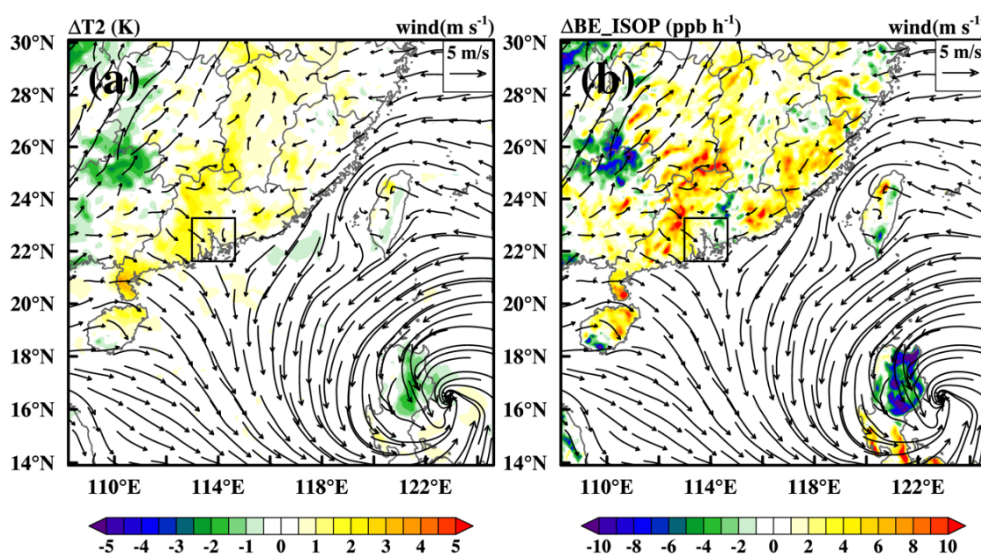
Figure 9: Mean distributions of \Delta T_2 (a) and \Delta BE\_ISOP (b) during the morning (09:00–12:00) of July 31.
