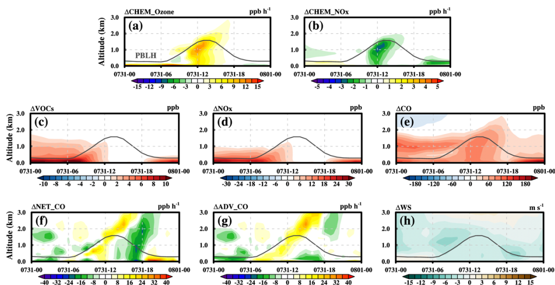
Figure 8: Vertical distributions of the changes in CHEM of ozone and the induced factors on July 31. (a) Changes in CHEM of ozone; (b) changes in CHEM of NO x ; (c) changes in the concentrations of VOCs; (d) changes in the concentrations of NO x ; (e) changes in the concentrations of CO; (f) changes in NET of CO; (g) changes in ADV of CO; and (h) changes in the WS.
