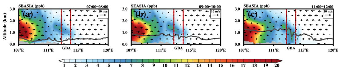
350 Figure 11: Mean vertical cross sections of the ozone contribution from SEASIA along the west-east direction during the morning on July 31. (a) 07:00-08:00; (b) 09:00-10:00; (c) 11:00-12:00.
