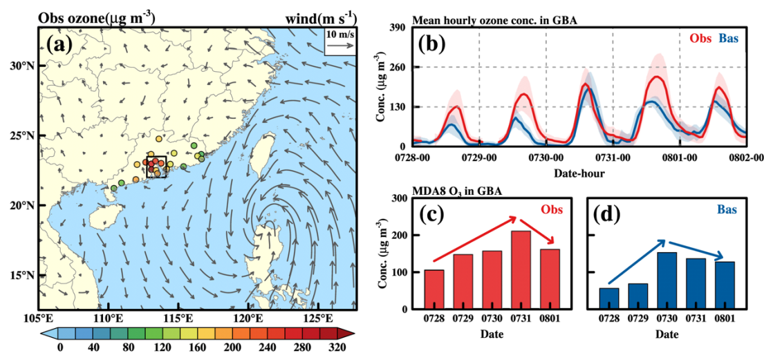
80 Figure 1: (a) Ozone observations (Obs ozone) for Guangdong Province and the 10-m wind fields at 14:00 on July 31, 2016; (b) mean hourly ozone concentrations in the Great Bay Area (GBA) from 00:00 on July 28 to 00:00 on August 2, 2016; (c-d) mean maximum daily 8-hour average ozone (MDA8 O 3 ) in the GBA from July 28 to August 1, 2016. The 10-m wind data originates from the European Centre for Medium-Range Weather Forecasts (ECMWF) Reanalysis V5 (ERA5) dataset. In Fig. 1(b), the shaded areas denote the standard deviations; red and blue denote the ozone observations (Obs) and basic simulation (Bas), respectively.
