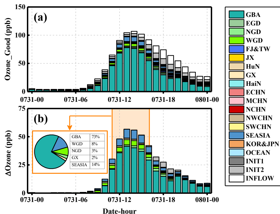
335 Figure 10: Mean surface ozone contributions of good EMs (a) and mean changes in surface ozone contributions between the good and bad EMs (b) in the GBA on July 31.
