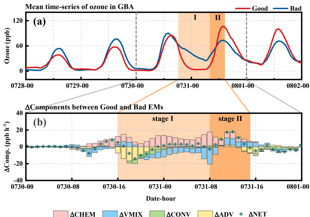
Figure 4: (a) Averaged time series of ozone good and ozone bad in the GBA and (b) the differences in each ozone component between the good and bad EMs from July 30 to 31. CHEM = chemistry, VMIX = vertical mixing, CONV = convection, ADV = advection, NET = net contribution.
