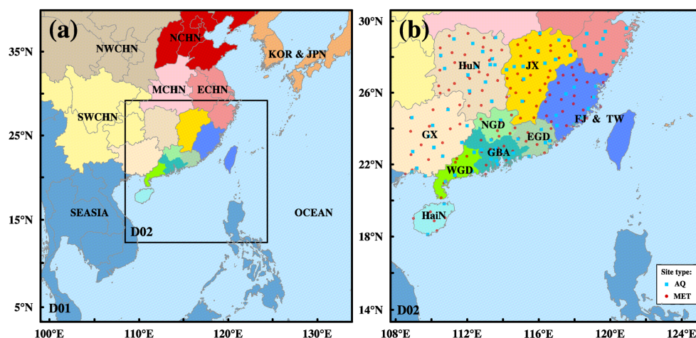
115 Figure 2: Model domain and geographical source region setting. The locations of the air quality (AQ; square) and meteorology (MET; dot) observation stations are shown in (b).
