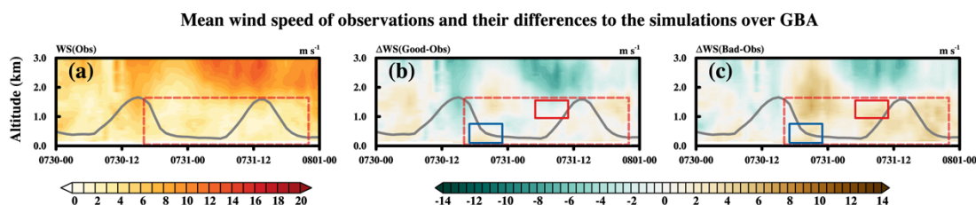
275 Figure 7: Vertical distributions of the WS observations in the GBA (a) and differences of WS between the simulations and observations [(b) for good EMs and (c) for bad EMs].
