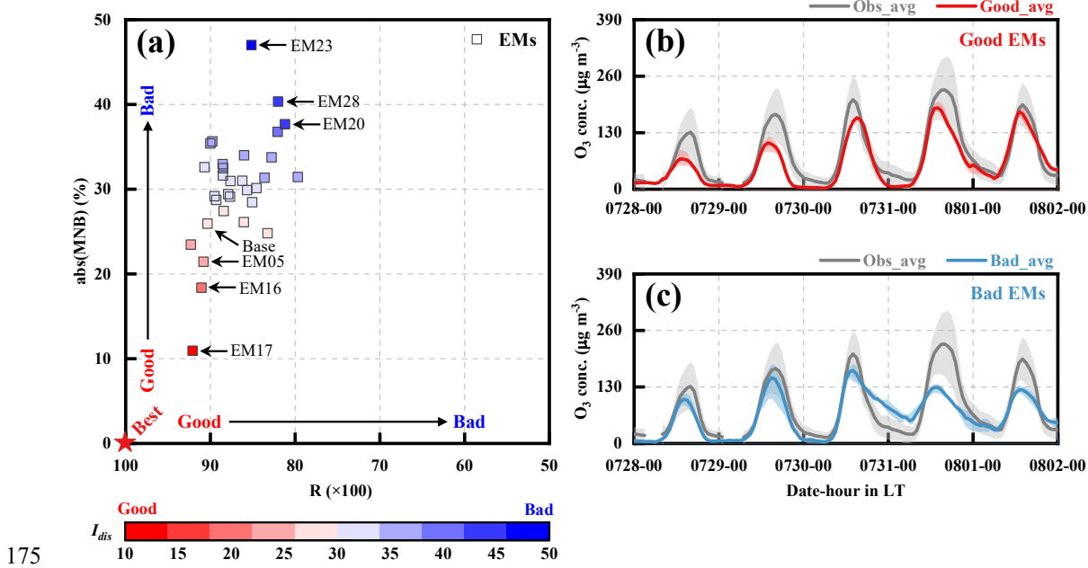
Figure 3: (a) Model performance of each EM on surface ozone in the GBA; comparisons between the observed and simulated surface ozone concentrations in the GBA for (b) good EMs and (c) bad EMs.
