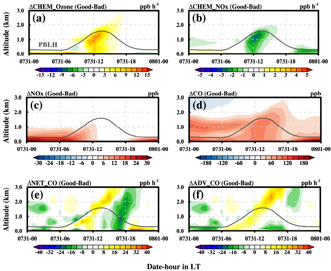
300 Figure 9: Vertical distributions of the changes in CHEM of ozone and the inducing causes on July 31. (a) Changes in CHEM of 305 ozone; (b) changes in CHEM of NO x ; (c) changes in the concentrations of NO x ; (d) changes in the concentrations of CO; (e) 310 changes in NET of CO; (f) changes in ADV of CO.
