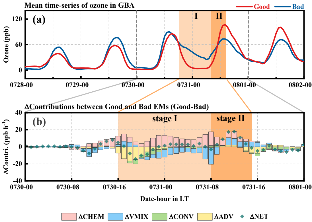
210 Figure 4: (a) Averaged time series of ozone good and ozone bad in the GBA and (b) the differences in each ozone contribution between the good and bad EMs (good-bad) from July 30 to 31. CHEM = chemistry, VMIX = vertical mixing, CONV = convection, ADV = advection, NET = net contribution.
