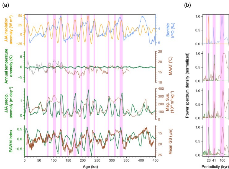
Figure 4: Model-proxy comparison in CLP. (a) Temporal variation in simulated JJA insolation anomaly (orange, W m^{-2} ), benthic \delta^{18}O stack (light blue, ‰, Lisiecki and Raymo, 2005), annual temperature (K), and JJA precipitation ( mm day^{-1} ) anomaly in CLP (green), East Asian Winter Monsoon index based on Wang and Cheng (2014). Insolation was averaged over 20^{\circ} N-40^{\circ} N . Brown lines indicate proxy records: Mean annual air temperature reconstructed from brGDGT ( ^{\circ}C ), magnetic susceptibility ( 10^{-8} m^3 kg^{-1} ), and mean grain size (mm) (Thomas et al. 2016). Vertical pink bars in (a) denote strong periods (SP). (b) Normalized power spectrum density of (a) (kyr). Vertical pink bars in (b) denote the main orbital cycles (precession, obliquity, and eccentricity).
