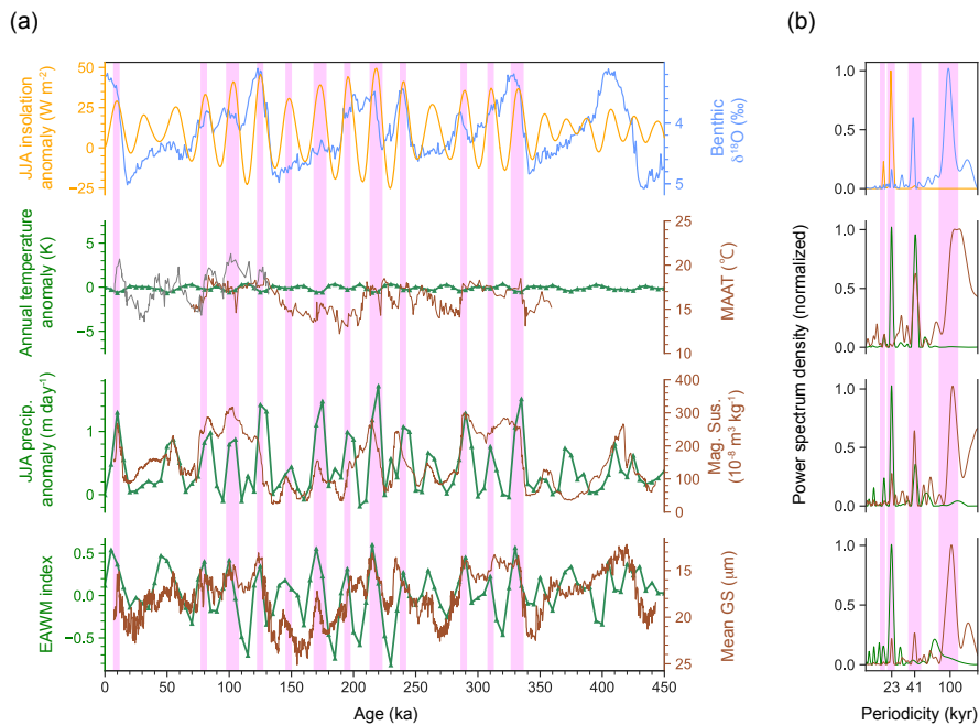
Figure 4: Model-proxy comparison in CLP. (a) Temporal variation in simulated JJA insolation anomaly (orange, \text{W m}^{-2} ), benthic \delta^{18}\text{O} stack (light blue, ‰, Lisiecki and Raymo, 2005), annual temperature (K), and JJA precipitation ( \text{mm day}^{-1} ) anomaly in CLP (green), East Asian Winter Monsoon index based on Wang and Cheng (2014). Insolation was averaged over 20^\circ\text{N} – 40^\circ\text{N} . Brown lines indicate proxy records: Mean annual air temperature reconstructed from brGDGT ( ^\circ\text{C} ), magnetic susceptibility ( 10^{-8}\text{ m}^3\text{ kg}^{-1} ), and mean grain size (mm) (Thomas et al. 2016). Vertical pink bars in (a) denote strong periods (SP). (b) Normalized power spectrum density of (a) (kyr). Vertical pink bars in (b) denote the main orbital cycles (precession, obliquity, and eccentricity).
