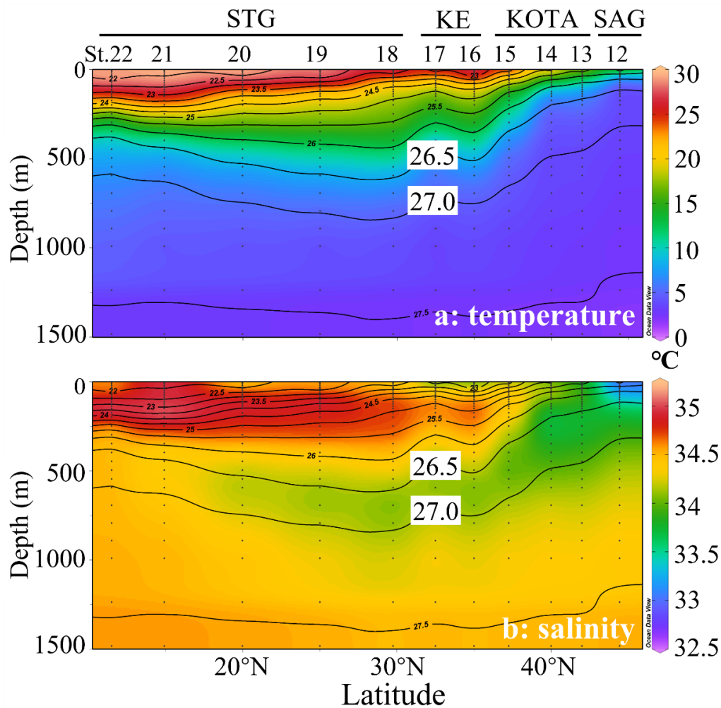
Figure 2: Section profiles of (a) in situ temperature (°C) and (b) salinity along the observational transect at 155° E from the subarctic gyre to the subtropical gyre. SAG : subarctic gyre, KOTA : Kuroshio-Oyashio Transition Area, KE : Kuroshio extension, STG : subtropical area. Black contour lines in the figures denote each potential density ( \sigma_\theta ) with special reference to the 26.5 and 27.0 \sigma_\theta isopycnal surfaces. In Figure 2b, the salinity minimum
