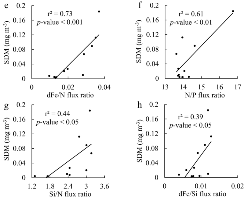
Figure 8: Comparisons of the subsurface diatom-derived Chl a maximum (SDM) to indiv-fluxes or flux ratios. Plots of the SDM vs. (a) dissolved Fe, (b) nitrate, (c) phosphate, and (d) silicate indiv-fluxes. Plots of SDM vs. (e) dFe/nitrate, (f) nitrate/phosphate, (g) silicate/nitrate, and (h) dFe/silicate flux ratios. The results of linear regression analysis with the coefficient of determination ( r^2 ) and p -values are shown in each plot.
