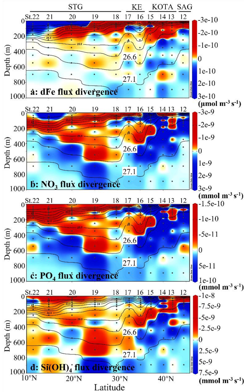
Figure 10: Vertical section profiles of (a) dissolved Fe flux divergence ( \mu\text{mol m}^{-3} \text{s}^{-1} ) along 155° E transect from the subarctic to subtropical Pacific, (b) nitrate flux divergence ( \text{mmol m}^{-3} \text{s}^{-1} ), (c) phosphate flux divergence ( \text{mmol m}^{-3} \text{s}^{-1} ) and (d) silicate flux divergence ( \text{mmol m}^{-3} \text{s}^{-1} ). The red and blue colors indicate the convergence and divergence of each nutrient flux, respectively. The highlighted 26.6 and 27.1 \sigma_\theta isopycnal surfaces suggest the shallower and deeper boundaries of the upper NPIW (U-NPIW). These figures were drawn using the ODV.
