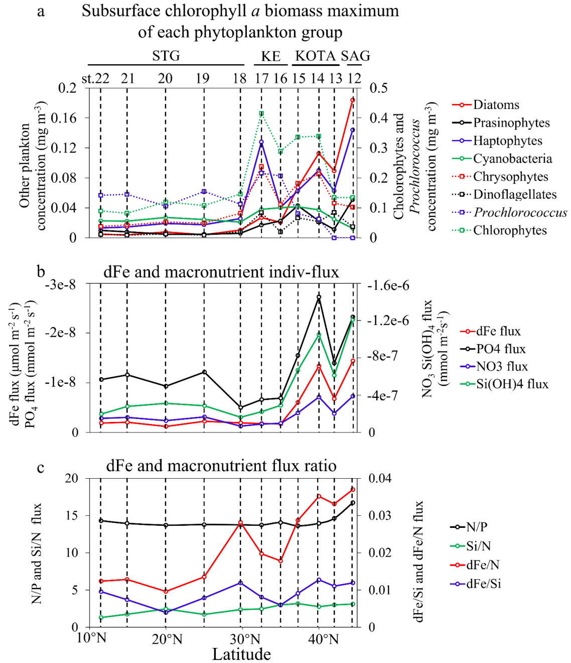
Figure 6: Latitudinal distribution patterns of (a) subsurface chlorophyll a biomass maximum (mg/m 3 ) of phytoplankton groups, including diatoms, prasinophytes, haptophytes, cyanobacteria (except Prochlorococcus ), chrysophytes, dinoflagellates, Prochlorococcus , and chlorophytes in terms of chlorophyll a (Chl a ) biomass (b) dissolved Fe and macronutrient indivi-fluxes and (c) dissolved Fe and macronutrient flux ratio.
