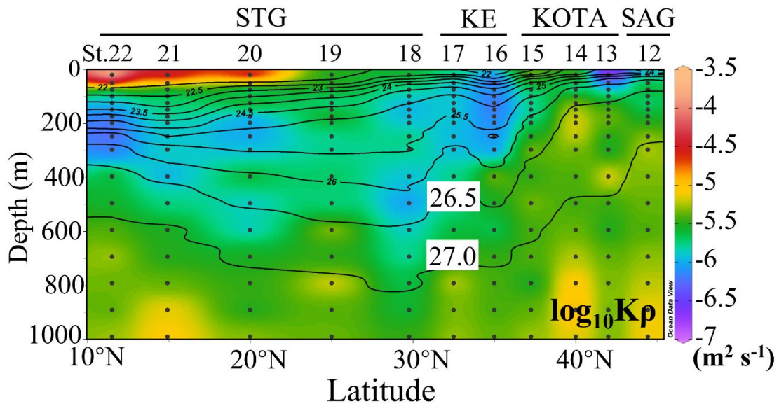
Figure 3: Vertical section profile of vertical diffusivity ( K_\rho ) along the 155° E transect from the subarctic to the subtropical Pacific. Black contour lines in the figure denote each potential density ( \sigma_\theta ) with special attention to the 26.5 and 27.0 \sigma_\theta isopycnal surfaces. This figure was drawn using the ODV.
