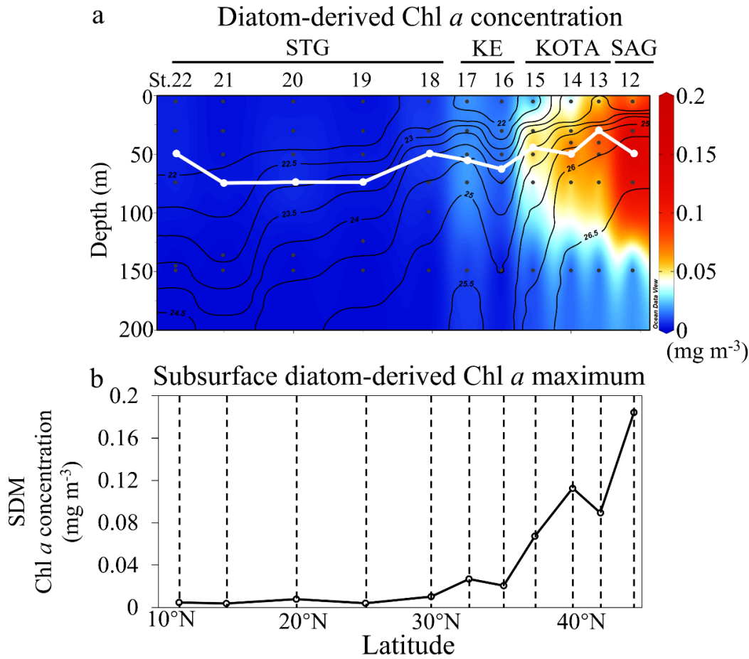
Figure 7: Section profiles of (a) diatom-derived Chl a concentration ( \text{mg m}^{-3} ), (b) the subsurface diatom-derived Chl a maximum (SDM) concentration ( \text{mg m}^{-3} ) at each station. In Figure 7a, the white line indicates the depth of SDM. Figure 7a was drawn using the ODV.
