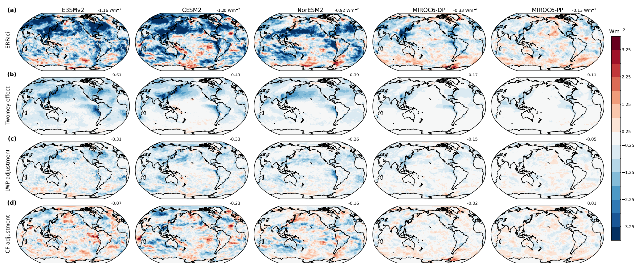
Figure A1. Components of SW ERFaci for each of the five GCMs. (a) Total SW ERFaci. Contribution to SW ERFaci from the (b) Twomey effect, (c) LWP adjustment, and (d) CF adjustment. From left to right, MODIS CRK decomposition for E3SMv2, CESM2, NorESM2, MIROC6-DP, and MIROC6-PP, respectively. Global-mean values of each component are indicated in the top-right corner of each plot.
