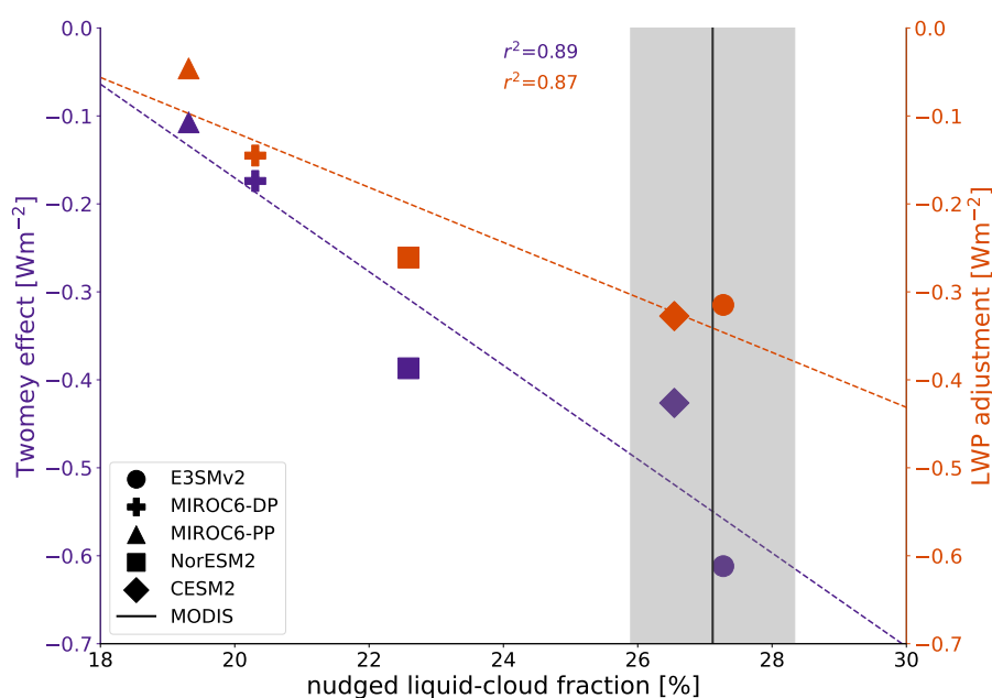
Figure 5. Emergent constraints on the global-mean Twomey effect and LWP adjustment. Each shape represents the estimate of the Twomey effect (purple) and the LWP adjustment (orange) for a specific GCM. The vertical black line indicates the MODIS-reported global annual-mean liquid-cloud fraction over the 2003–2014 period. The grey shading represents the 68 % confidence interval ( \pm 1\sigma range) for the MODIS global-mean LCF. The values in the top-middle section of the plot give the squared coefficient of determination for the ordinary least-squares linear-regression fit ( r^2 ) for each respective fit.
