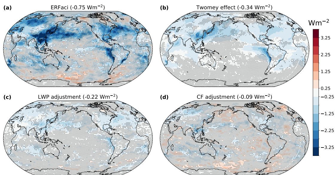
Figure 2. Components of SW ERFaci averaged over the five GCMs. (a) Total SW ERFaci. Contribution to SW ERFaci from the (b) Twomey effect, (c) LWP adjustment, and (d) CF adjustment. Global-mean values of each component are indicated in parenthesis. Stippling indicates regions where the five models disagree on the sign of SW ERFaci.
