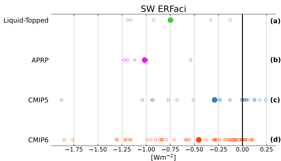
Figure 6. A comparison of global-mean SW ERFaci estimates calculated from the new MODIS CRK method and APRP. (a) Total SW ERFaci from liquid clouds as diagnosed by our new technique. (b) Total SW ERFaci computed using APRP across our ensemble. Total SW ERFaci computed using APRP across an ensemble of (c) CMIP5 and (d) CMIP6 models from Zelinka et al. (2023). A selection of the models analyzed in this paper (CESM2, MIROC6, NorESM2) are included in the CMIP6 ensemble. Present-day aerosols are defined as year 2000 in our results and year 2014 for CMIP6.
