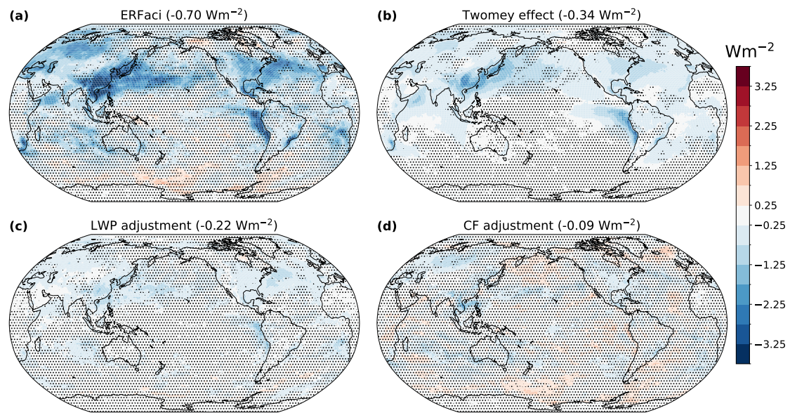
Figure 2. Components of SW ERFaci and its components averaged over the five GCMs. (a) Total SW ERFaci. Contribution to SW ERFaci from the (b) Twomey effect, (c) LWP adjustment, and (d) CF adjustment. Global-mean values of each component are indicated in parenthesis. Stippling indicates regions where the five models disagree on the sign of SW ERFaci.
