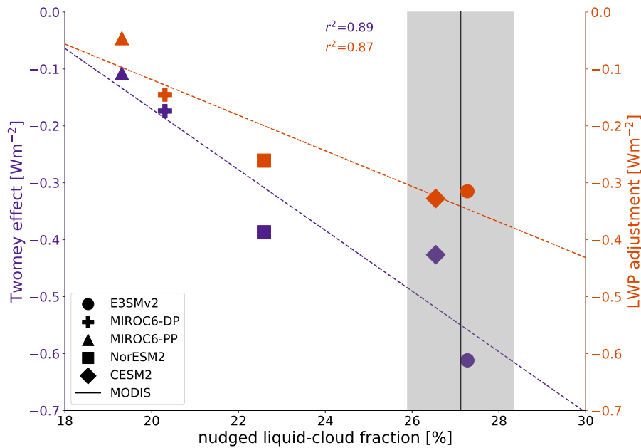
Figure 5. Emergent-Potential emergent constraints on the global-mean Twomey effect and LWP adjustment. Each shape-marker represents the estimate of the Twomey effect (purple) and the LWP adjustment (orange) for a specific GCM. The vertical black line indicates the MODIS-reported global annual-mean liquid-cloud fraction over the 2003–2014 period. The grey shading represents the 68 % confidence interval ( \pm 1\sigma range) for the MODIS global-mean LCF. The values in the top-middle section of the plot give the squared coefficient of determination for the ordinary least-squares linear-regression fit ( r^2 ) for each respective fit.
