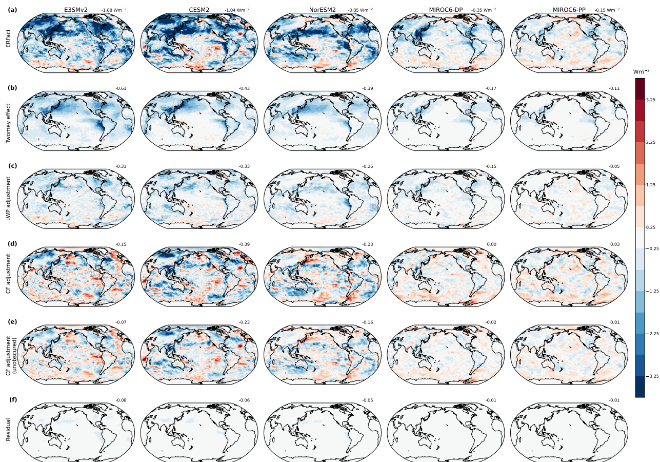
Figure A1. Components of SW ERFaci and its components for each of the five GCMs. (a) Total SW ERFaci. Contribution to SW ERFaci from the (b) Twomey effect, (c) LWP adjustment, and (d) CF adjustment. (e) Obscuration-corrected CF adjustment and (f) residual of the ERFaci decomposition. From left to right, MODIS CRK decomposition for E3SMv2, CESM2, NorESM2, MIROC6-DP, and MIROC6-PP, respectively. Global-mean values of each component are indicated in the top-right corner of each plot.
