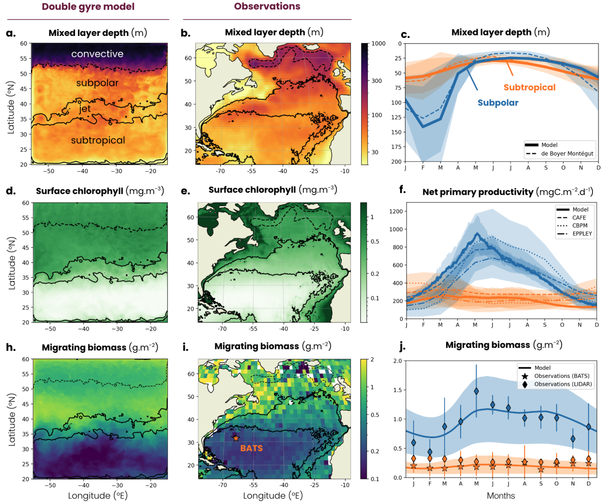
Figure 2. Map of annual mean (a,b) mixed layer depth (MLD), (d,e) surface chlorophyll concentration and (h,i) migrating zooplankton biomass in (a,d,h) the double gyre model and (b,e,i) observation-based data products. The subtropical, jet and subpolar biomes are delimited by solid black lines (mean surface chlorophyll concentration = 0.15 and 0.35 \text{mg m}^{-3} ), while the subpolar and convective biomes are delimited by a dashed line (mean MLD = 200 m, see Methods). Mean seasonal cycle of (c) MLD, (f) net primary productivity and (j) migrating zooplankton biomass in the subtropical biome (orange) and the subpolar biome (blue) in the double gyre model (solid lines) and observation-based products (dashed lines). Shading and error bars correspond to two standard deviations around the average. Orange star in (i) indicate the Bermuda Atlantic Time-series Study (BATS). See Sect. 2.2 for observational product details.
