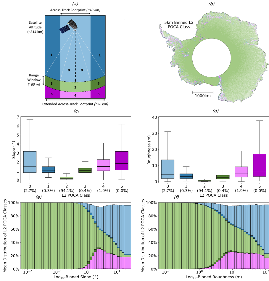
Figure 7. Assessment of the ability of Sentinel-3 to capture the surface reflection at the L2-derived POCA. Panel a outlines the POCA class definitions as per Fig. 1 for ease of cross-referencing. Panel b shows the L2-derived POCA classes, spatially binned to 5 km. Panels c and d show box plots of the L2-derived POCA per-class distribution with respect to slope and roughness, with the percentage of data within each class given in parentheses. Panels e and f show stacked bar charts representing the percentage distribution of the L2-derived POCA classes within each slope and roughness bin.
