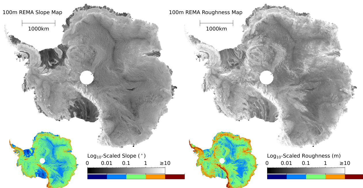
Figure 2. 5 km resolution, \log_{10} -scaled slope and roughness maps of Antarctica generated using 100 m resolution REMA and the Singular Value Decomposition techniques outlined in Sect. 5.1. The coloured inset maps show discretely binned versions of these datasets, to aid the visualisation of broader scale patterns.
