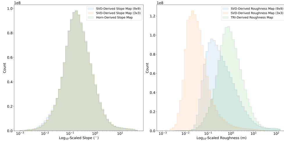
Figure 4. Comparison of slope and roughness estimates using different methods applied to the 100 m resolution REMA DEM. Panel a shows slope calculated using (1) Horn’s method with a 3x3 pixel (300x300 m) window, (2) our SVD-based approach, calculated with a 3x3 pixel window for consistency with Horn’s method, and (3) our SVD-based approach with a 9x9 pixel window. Panel b shows roughness computed using (1) TRI (3x3 pixel window), (2) our SVD-based approach using the same 3x3 pixel window size for consistency with TRI, and (3) our approach using a 9x9 pixel window.
