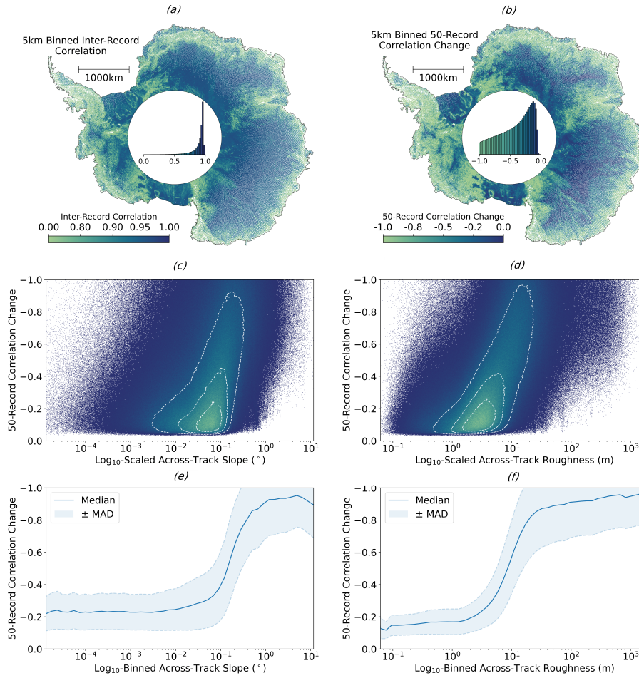
Figure 9. Analysis of the along-track correlation of Sentinel-3 SAR altimetry echoes. Panel a shows the correlation between consecutive records, spatially binned to 5 km. Panel b shows the 50-record correlation change, also spatially binned to 5 km. Histograms showing the overall distribution of each parameter are given within the pole holes of the respective plots. Panel c and d show density plots of the 50-record correlation change as a function of \log_{10} -binned slope and roughness respectively. Concentric contours are included, which contain 75%, 50%, and 25% of the data from outside to in respectively. Panels e and f show the median and median absolute deviation of the 50-record correlation change with respect to \log_{10} -binned slope and roughness, respectively.
