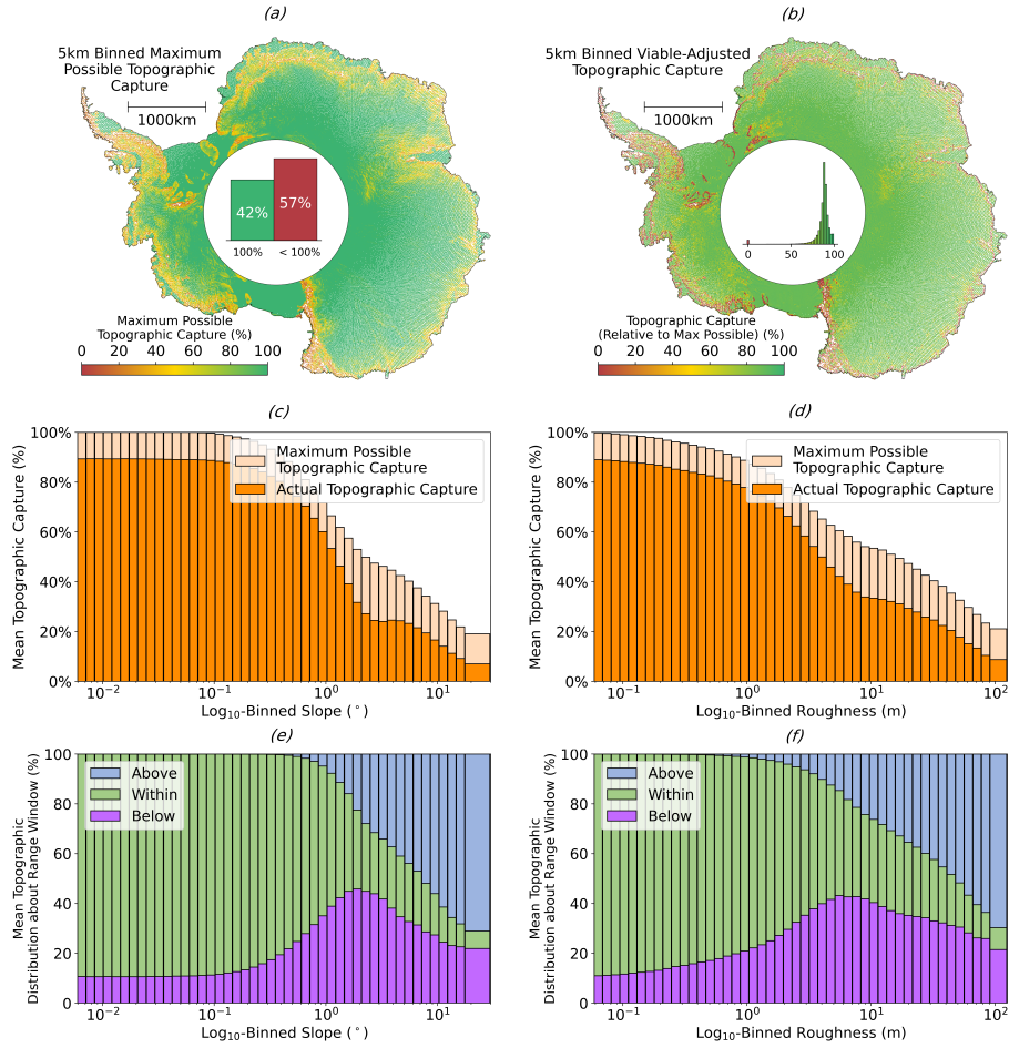
Figure 5. Assessment of the ability of the Sentinel-3 range window to capture the full topographic surface within the beam-limited footprint. Panel a exhibits the maximum possible percentage of topography (REMA; 100 m resolution) that can be captured with an optimal placement of the 60 m range window, binned to 5 km. The percentage of records where full (100%) topographic capture is, and is not, possible is shown within the bar graph in the pole hole. Panel b shows the percentage of topography that is captured by the current placement of the range window with respect to the maximum possible capture (panel a), binned to 5 km, with the corresponding distribution shown within the pole hole. A value of 0 indicates that the current placement of the range window entirely misses the ice surface, whereas a value of 100 indicates that the range window captures the maximum possible area of the illuminated surface (not necessarily 100% of the surface). Panels c and d show stacked bar charts representing the maximum percentage of topography within the satellite footprint that can be captured, and that which is currently captured, with respect to \log_{10} -binned slope and roughness respectively. Panels e and f show stacked bar charts, indicating the distribution of REMA points within the illuminated beam-limited footprint that are above, within, and below the range window, with respect to \log_{10} -binned slope and roughness.
