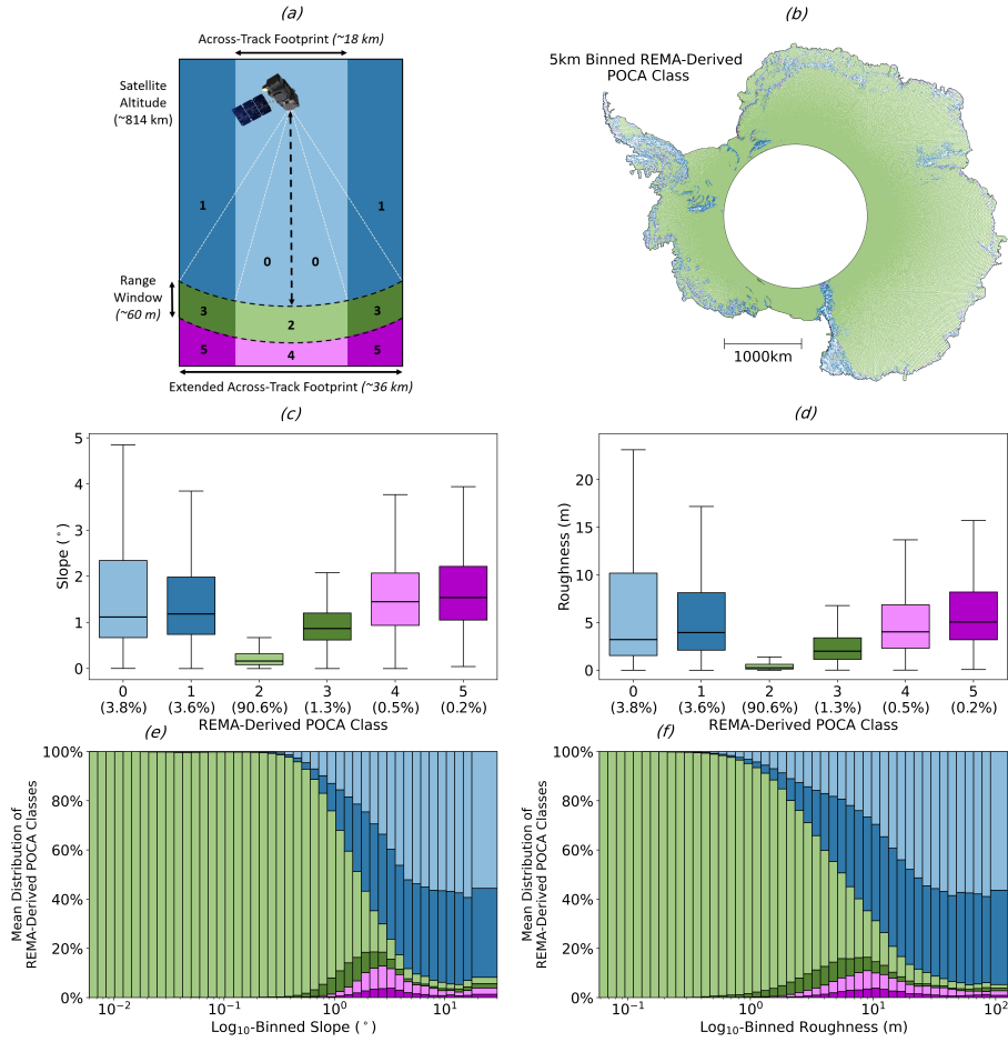
Figure 8. Assessment of the ability of Sentinel-3 to capture the surface reflection at the REMA-derived POCA. Panel a outlines the POCA class definitions as per Fig. 1 for ease of cross-referencing. Panel b shows the REMA-derived POCA classes, spatially binned to 5 km. Panels c and d show box plots of the REMA-derived POCA classes with respect to slope and roughness. Panels e and f show stacked bar charts representing the percentage distribution of the REMA-derived POCA classes with respect to log 10 -binned slope and roughness.
