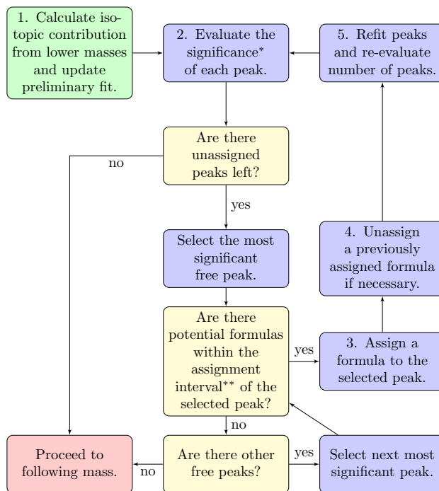
Figure 3. Flowchart describing the peak assignment process on a general level for each integer mass in the spectrum . More detailed description of how each step marked with a number works is provided in Sect. 2.1.3. (*) The significance of a peak refers to how much the omission of that peak would increase the \chi^2 value of the fit. (**) The assignment interval can be adjusted, but is set to the default value of 0.2 \times \text{FWHM} for all of the runs presented in this paper.
