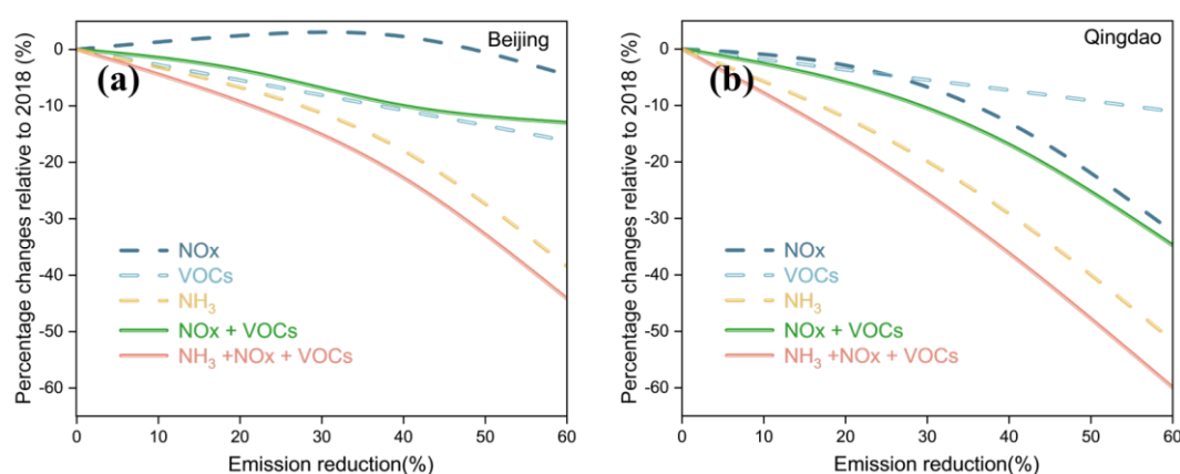
Figure 14 Relative changes in the \text{PM}_{2.5} nitrate contribution in response to the emission reduction scenarios in (a) Beijing and (b) Qingdao, compared with the winter 2018 baseline conditions.
