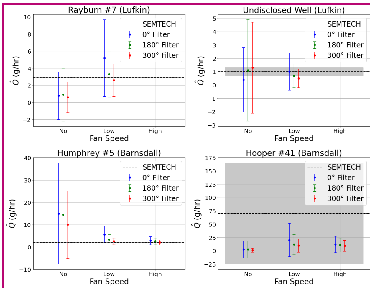
Figure 4611: Estimated leak rates ( \hat{Q} ) and uncertainties ( \sigma_{\hat{Q}} ) for the four wells shown in Figure 436 from the SEMTECH (black and gray) and FAST method (colored). SEMTECH is able to get very accurate readings for all wells except Hooper #41 which was a highly variable well. The FAST method (with the fan on) works almost as well as the SEMTECH with 300 degrees of filtering and provides a more accurate reading than the SEMTECH for Hooper #41, likely due to the larger sampling volume.
