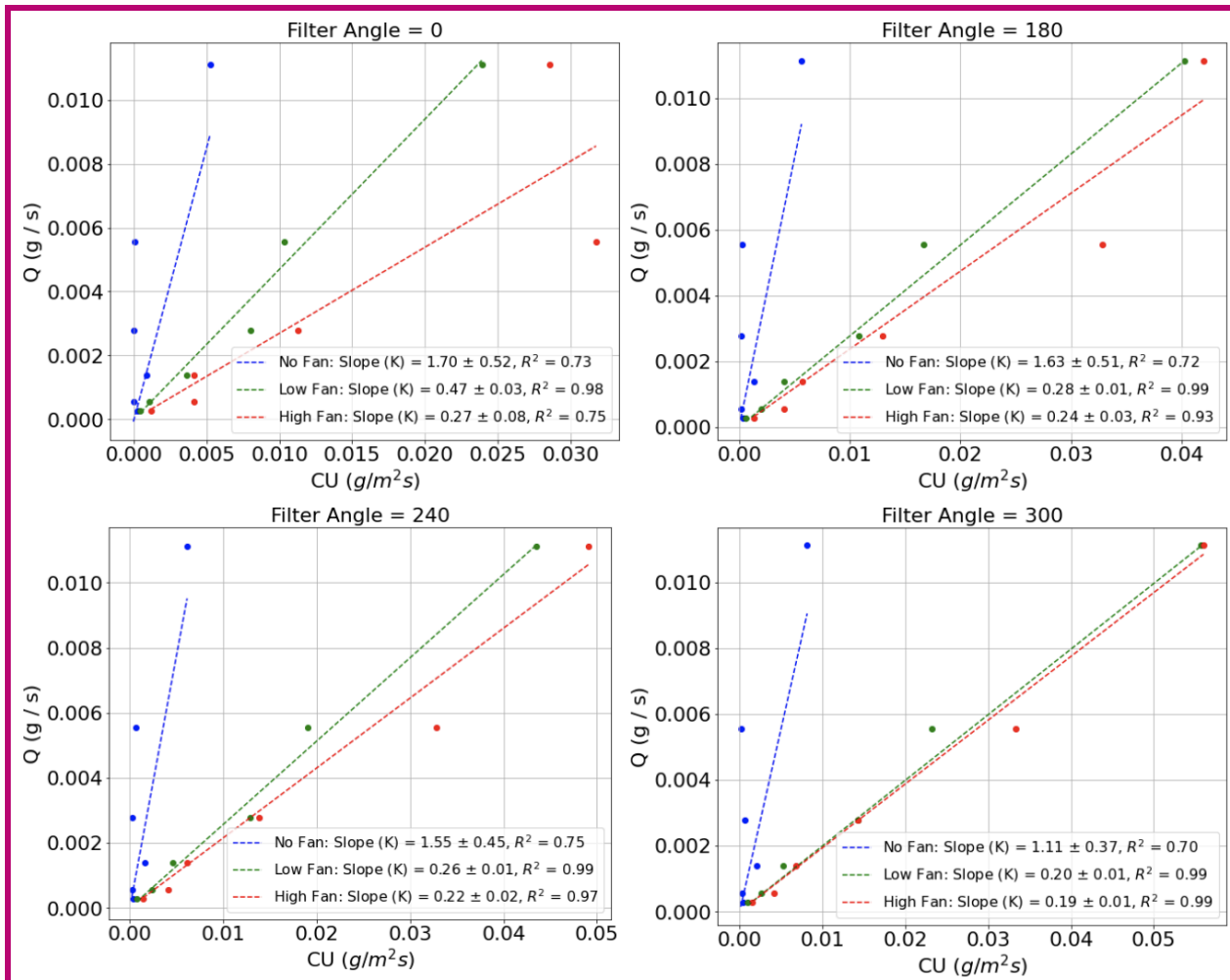
Figure 447: Measured mean C \cdot U (along x) vs. known Q (along y) for the control release experiment used to determine the values of K_{FAST} (slopes) for a range of fan speeds and filtering angles.
