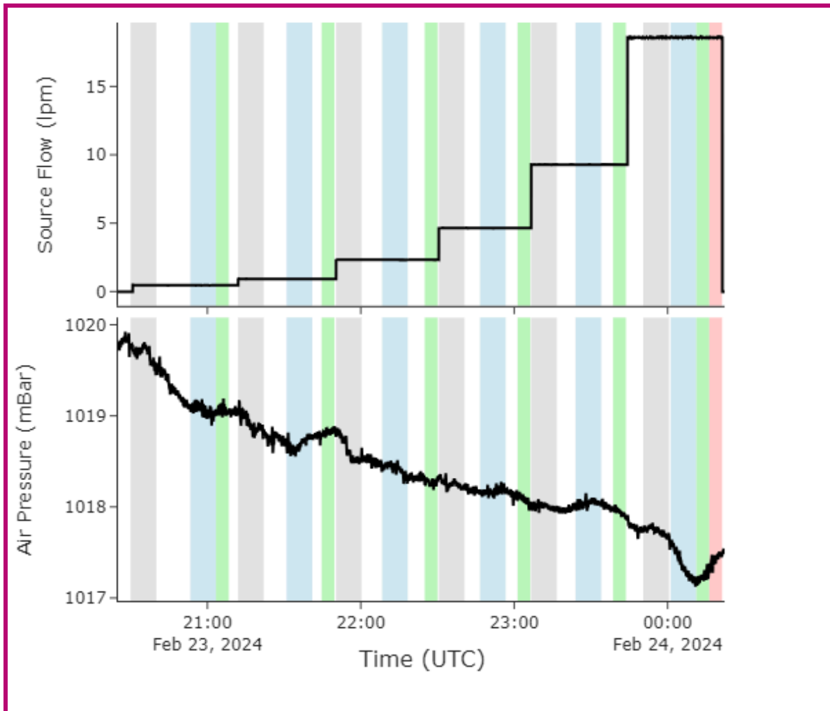
Figure 94: Time series of the output flow rate (liters per minute) throughout the Richmond controlled release experiment with shaded areas indicating the set measurement windows: gray for no fan state, blue for fan on at low speed, green for fan on at high speed, and red for maximum fan speed at the end of the experiment.
