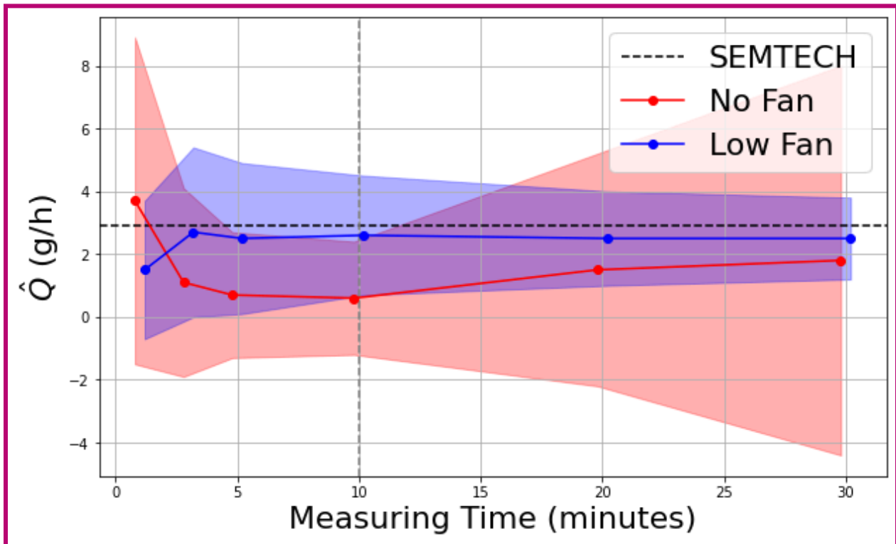
Figure 4712: Estimated leak rates ( \hat{Q} ) and uncertainties ( \sigma_{\hat{Q}} ) from the FAST method for Rayburn #7 as a function of the sampling time used to make the estimate. Without a fan, the measurement is highly uncertain throughout, except for the range from 5-10 minutes. With the fan, the measurement accuracy gets higher with increasing measurement time, but the mean
