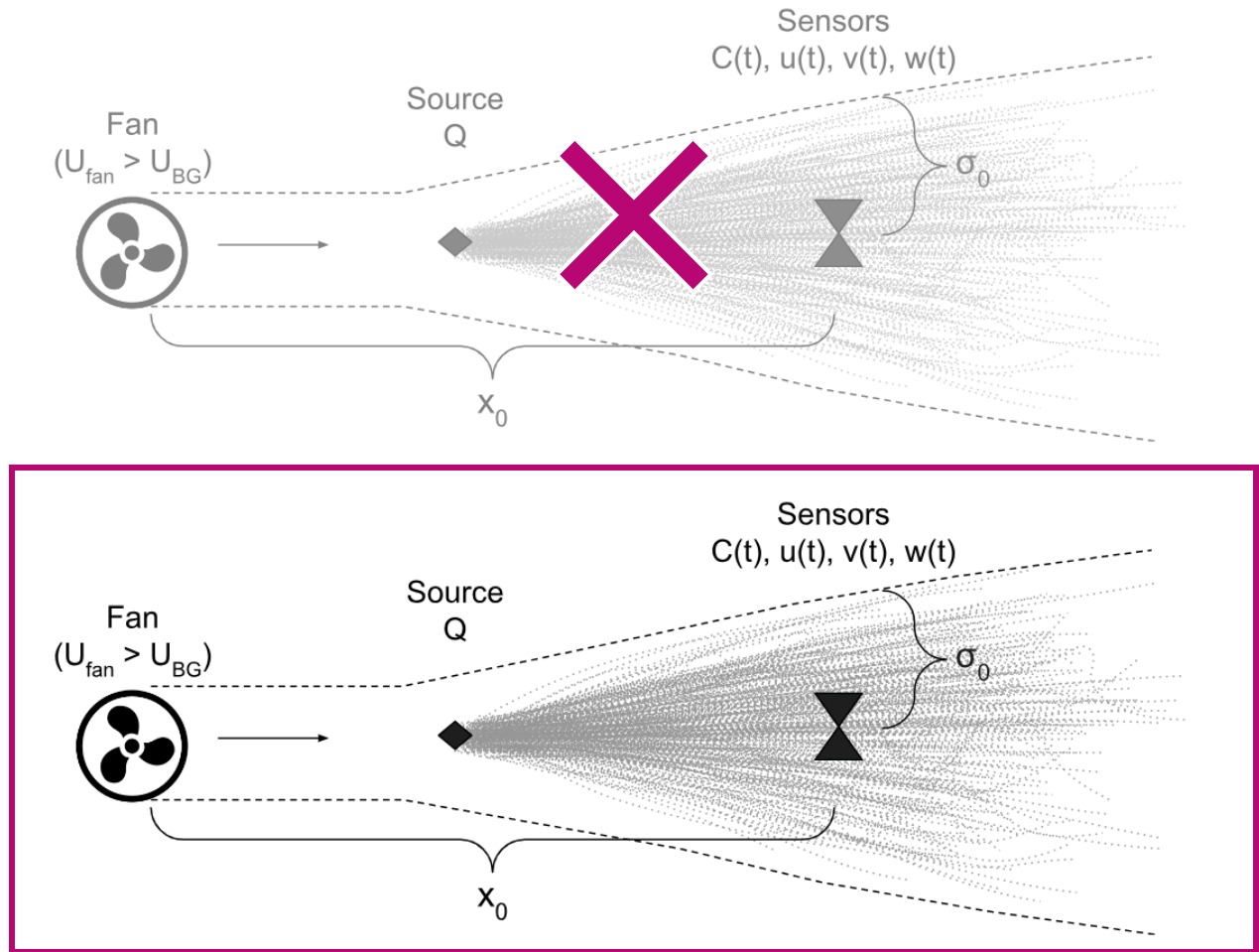
Figure 1: Schematic of the FAST method where an upwind fan (with mean downwind speed U_{fan} larger than the background U_{BG} ) generates a turbulent jet to advect a non-reactive gas ( CH_4 ) leaking at volumetric flow rate ( Q ) from a source to downwind sensors (anemometer measuring u(t) , v(t) , w(t) and CH_4 analyzer measuring C(t) ).
