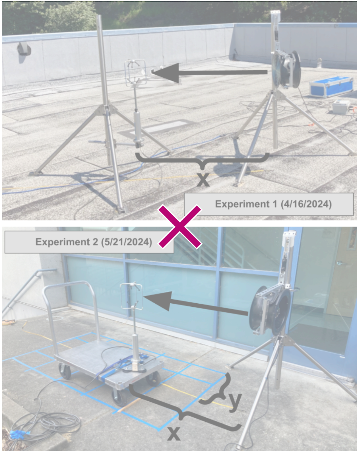
Figure 2: Experimental setup for fan characterization experiments, using an anemometer placed at a downwind distance x and crosswind distance y (second experiment)
