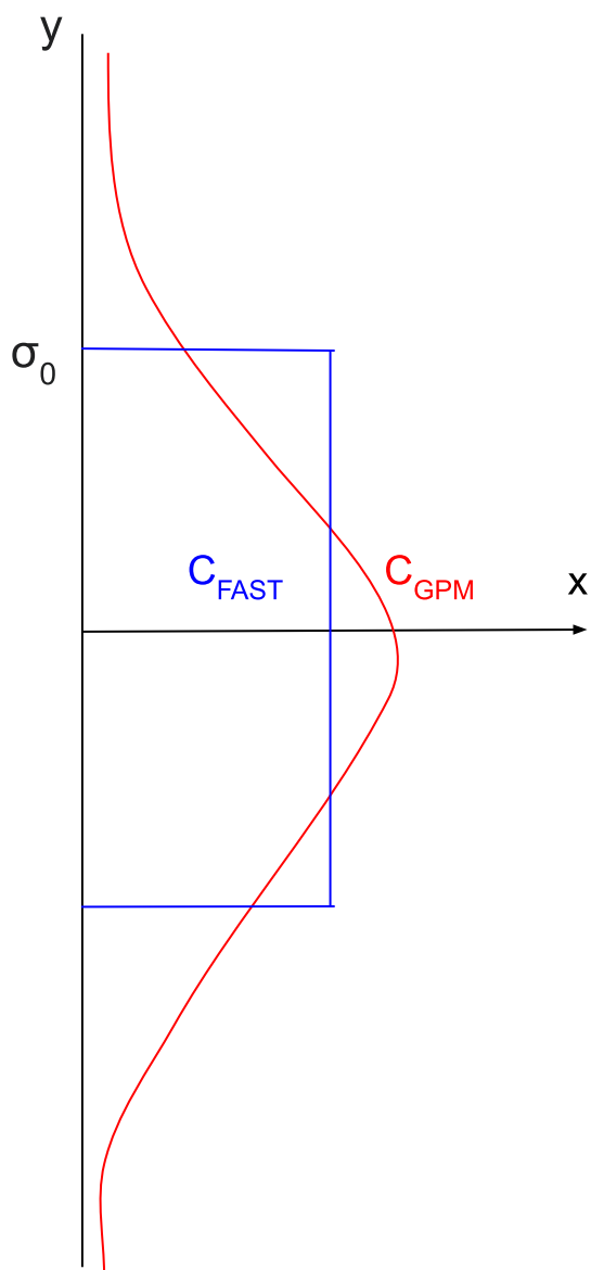
Figure 2A1: Diagram showing the difference in concentration profiles (C) used by the FAST (blue) and GPM (red) methods
