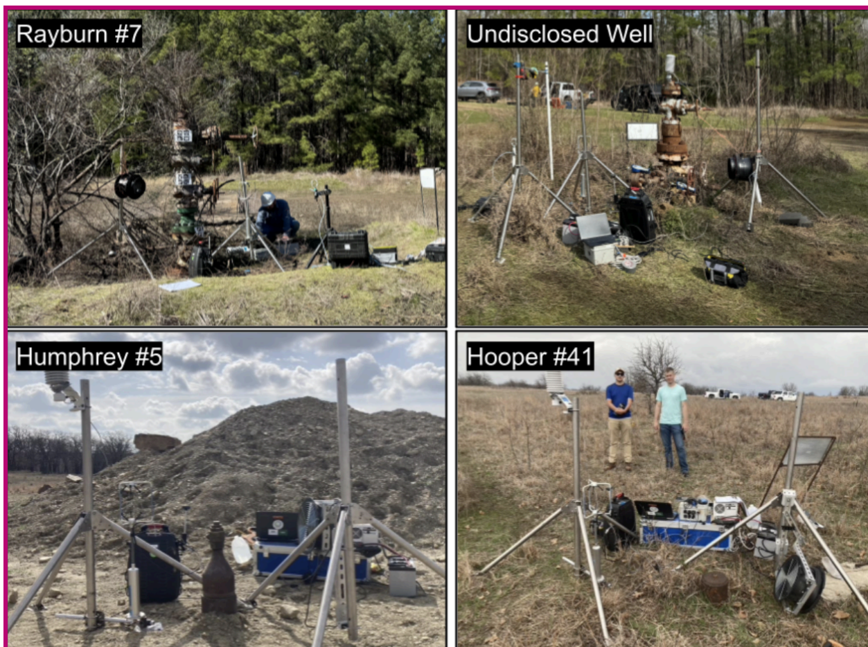
Figure 6: Wells measured in Lufkin, Texas (top) and Barnsdall, Oklahoma (bottom) using the FAST method. Both wells in Texas were of the “christmas tree” variety (multiple potential leak points) and were measured using No Fan and Low Fan speeds because the background wind speeds were < 1 m/s. Both wells in Oklahoma were lower to the ground, had only one leak point and were measured with No Fan, Low Fan and High Fan speeds due to the higher background winds ( > 1 m/s).
