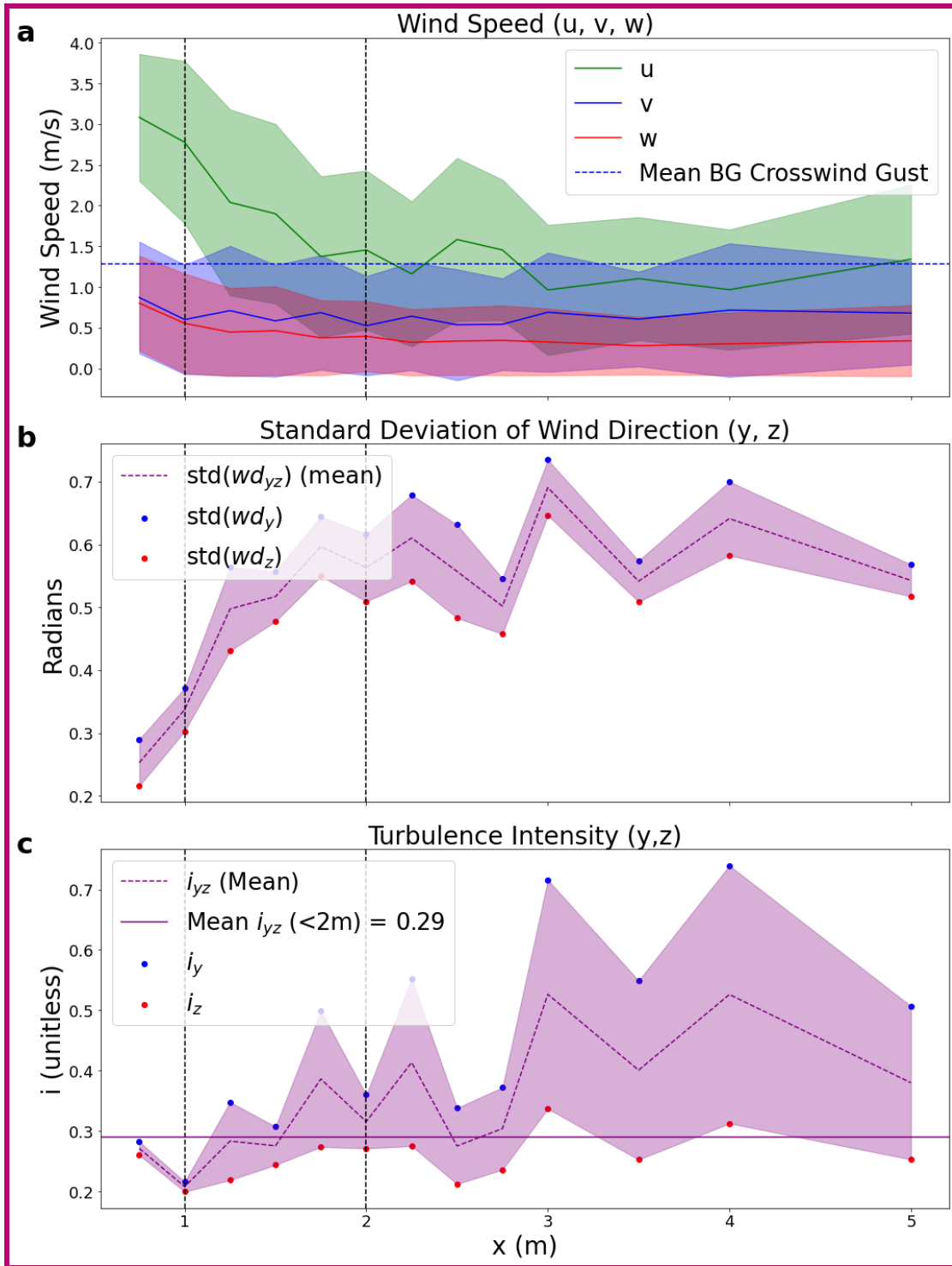
Figure C1: a) Wind speed, b) standard deviation of wind direction, and c) turbulence intensity as a function of downwind distance x for Experiment 1 using the “Low” fan speed setting. Data are filtered to remove any points coming from the negative x direction (180 degrees)
