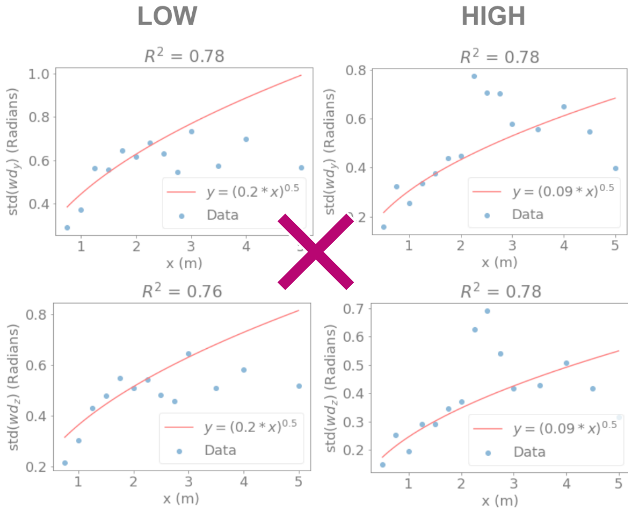
Figure 5: Square root fits to the standard deviations (std) of wind direction with filter angle = 180 degrees as expected by equation 2. The fits are valid in the range of 1-2 meters and depart from the square root curve at larger downwind distances.
