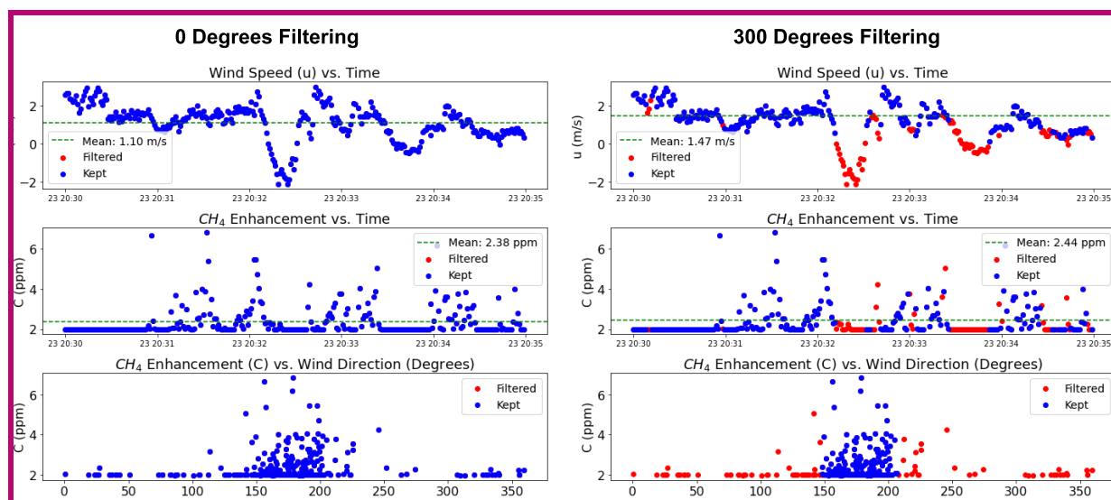
Figure 5: Time series of wind speed ( u ) and methane enhancement ( C ) as well as C vs. wind direction (in degrees) for a 'no fan' release of 1 g/hr at the Richmond Field Station. Kept data are shown in blue while filtered data are shown in red. Mean wind speed and concentration over the 5 minute measurement period are shown in green.
