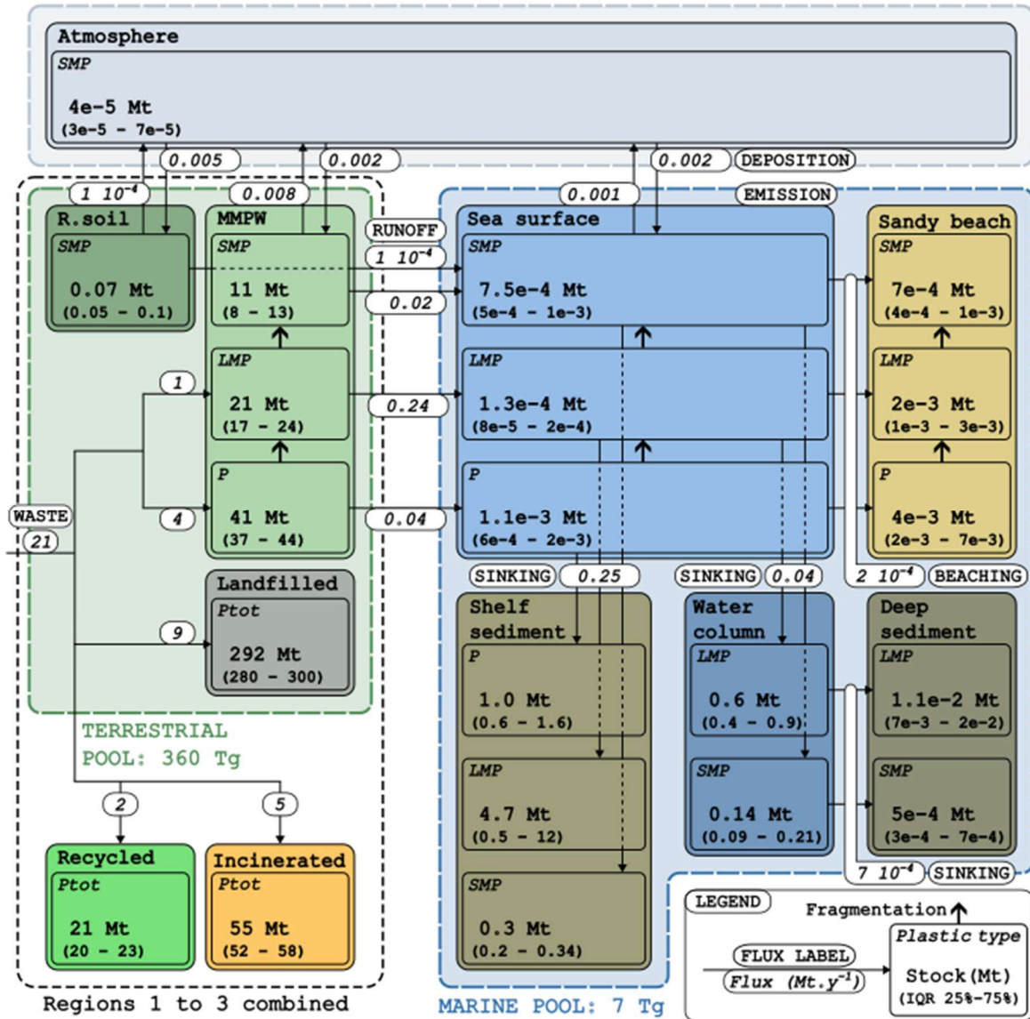
Figure 2 (double column). Structure of the box-model and model estimation of plastic stocks and fluxes for the reference year 2015. Each box is associated with a plastic size category ( P \geq 5\text{mm} , 0.3\text{mm} \leq \text{LMP} < 5\text{mm} and 1\mu\text{m} \leq \text{SMP} < 0.3\text{mm} ) and its corresponding modelled median stock in millions of metric tonnes (Mt) for the year 2015 under all scenarios. The uncertainties provided are interquartile range (Q25-Q75). Numbers in white labels are the annual plastic flux between boxes (in \text{Mt y}^{-1} ). When the label stretches across multiple arrows it indicates the combined flux of these arrows. Bold arrows represent degradation of plastic items to smaller size categories (P to LMP to SMP) under UV and mechanical abrasion. Note that the 3 modelled terrestrial regions are combined in this Figure on the left. “R. soil” stands for “remote soil surfaces” and “MMPW” for “terrestrial mismanaged plastic waste”.
